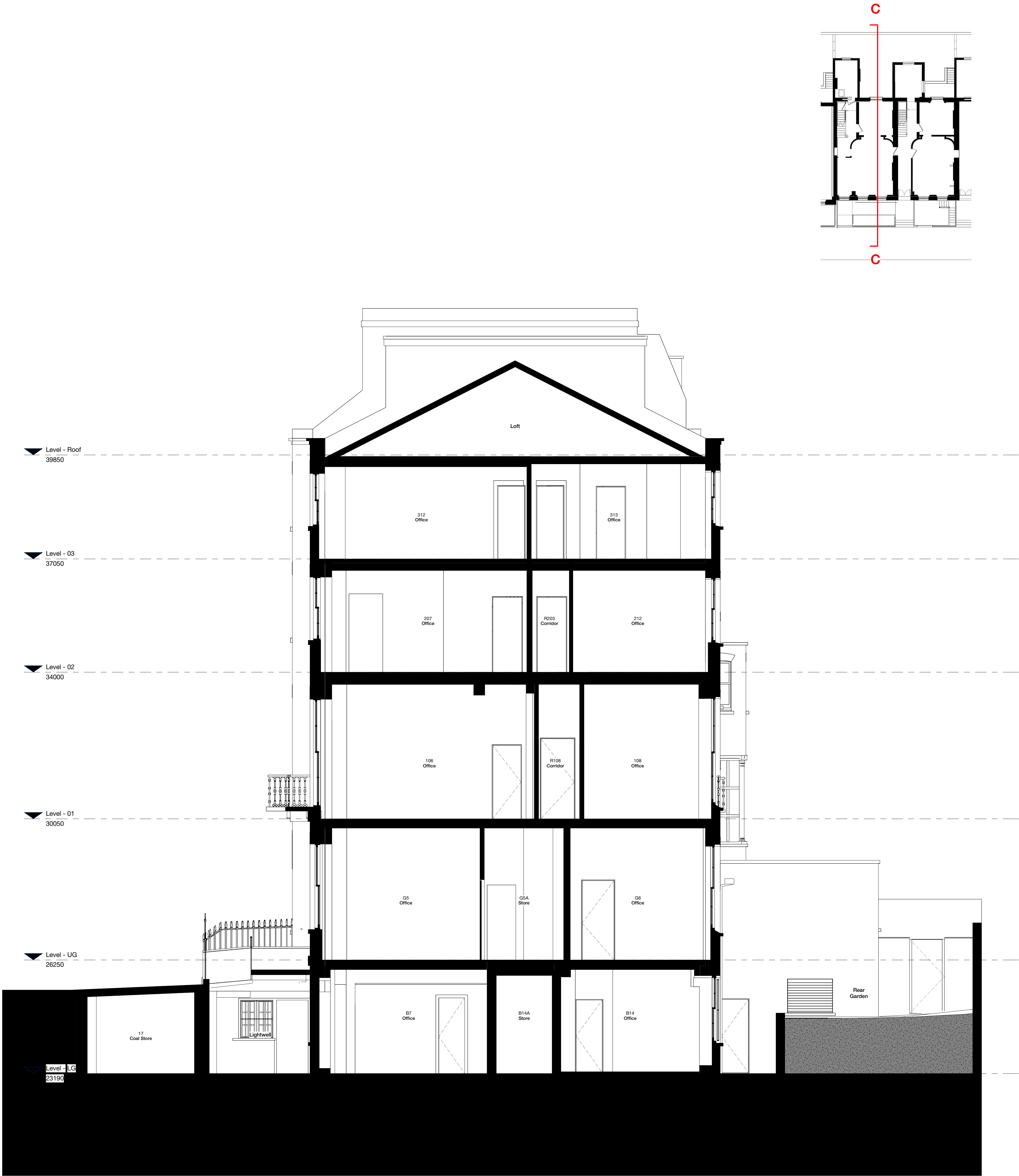
Existing Section CC (Through 26 Woburn Square) 1 : 50
