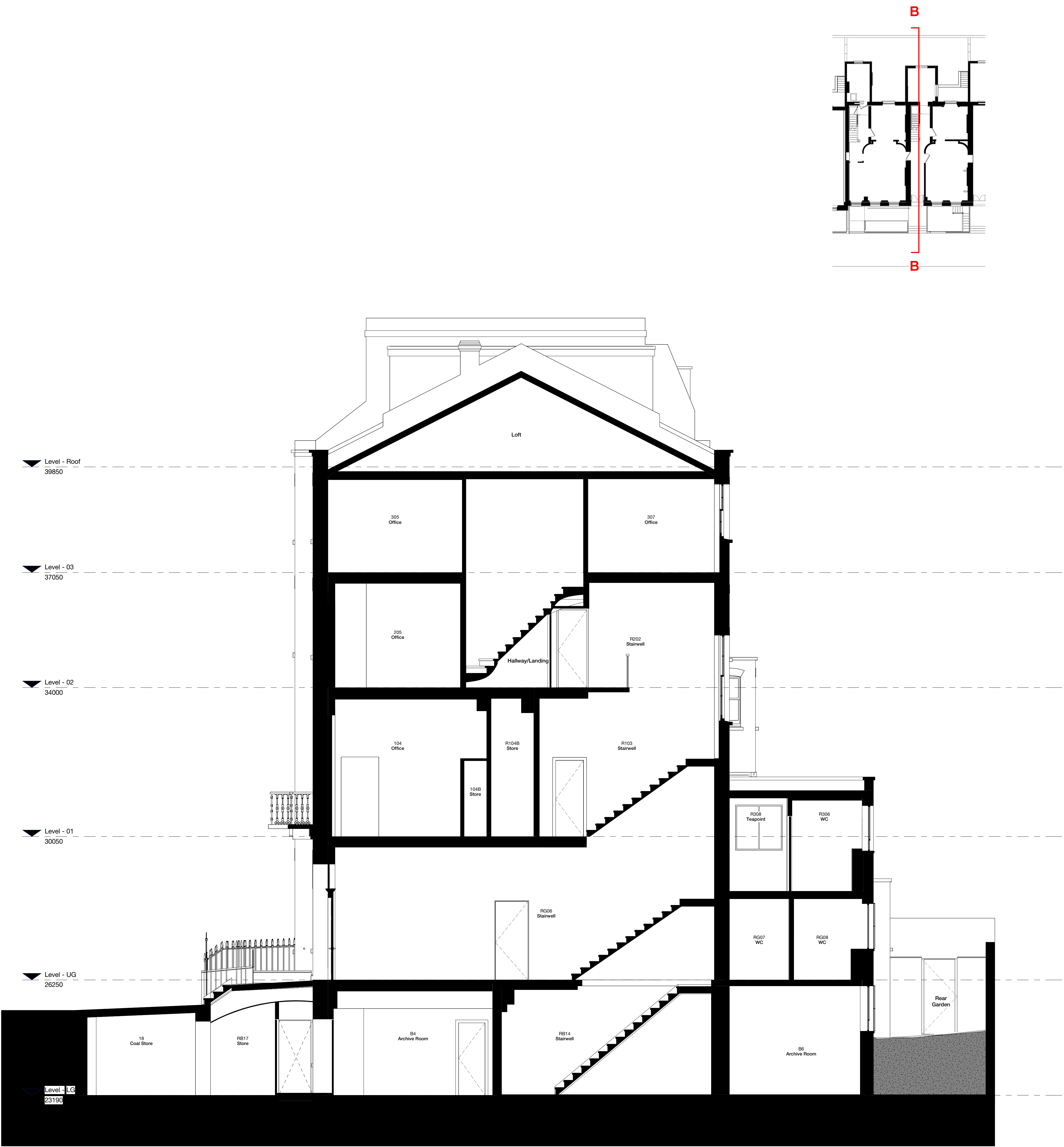
Existing Section BB (Through 25 Woburn Square)
