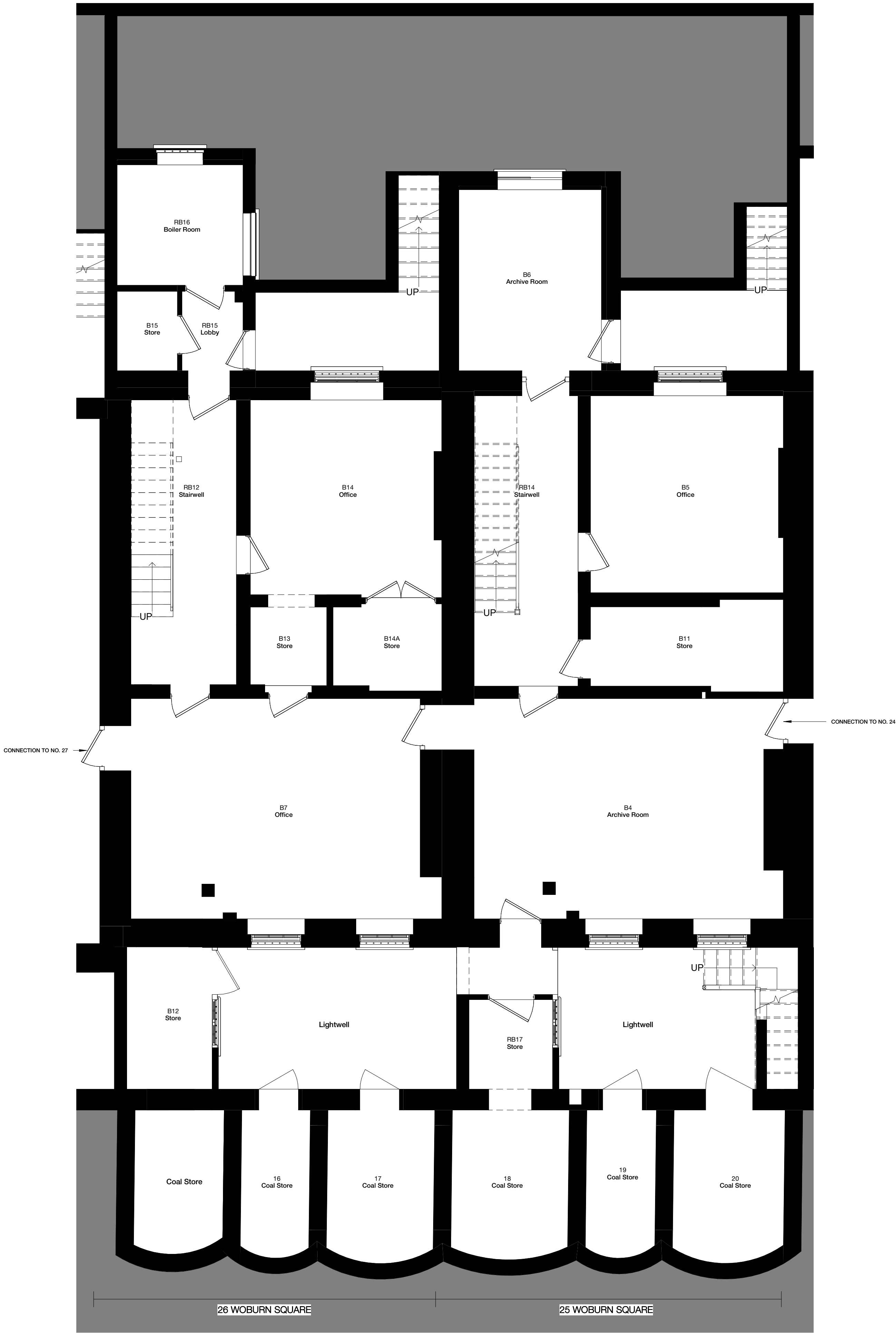
Existing Lower Ground Floor Plan
