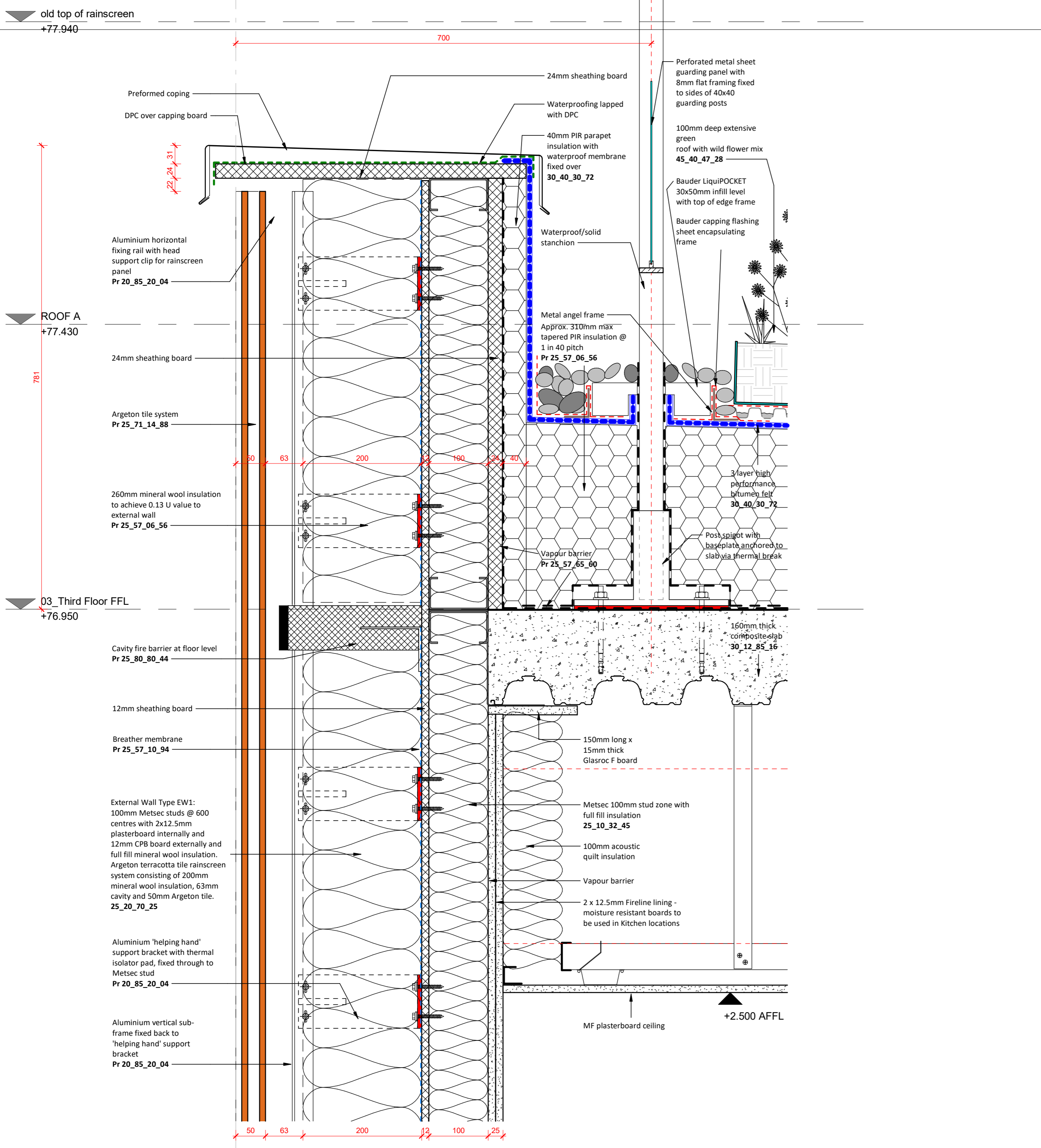
1 Typical Argeton Parapet Section 1:5
