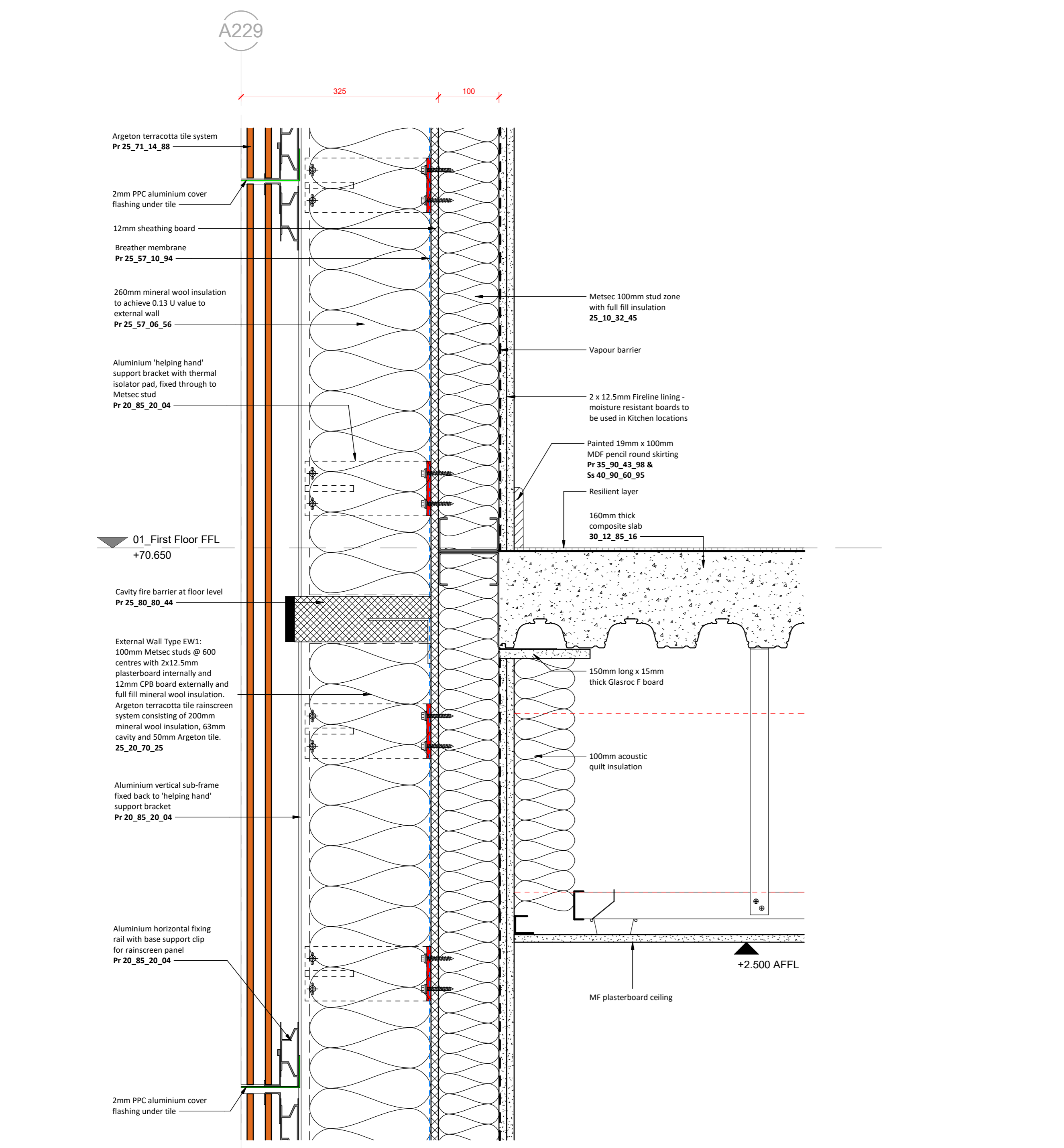
2 Typical Argeton Floor Section 1:5
