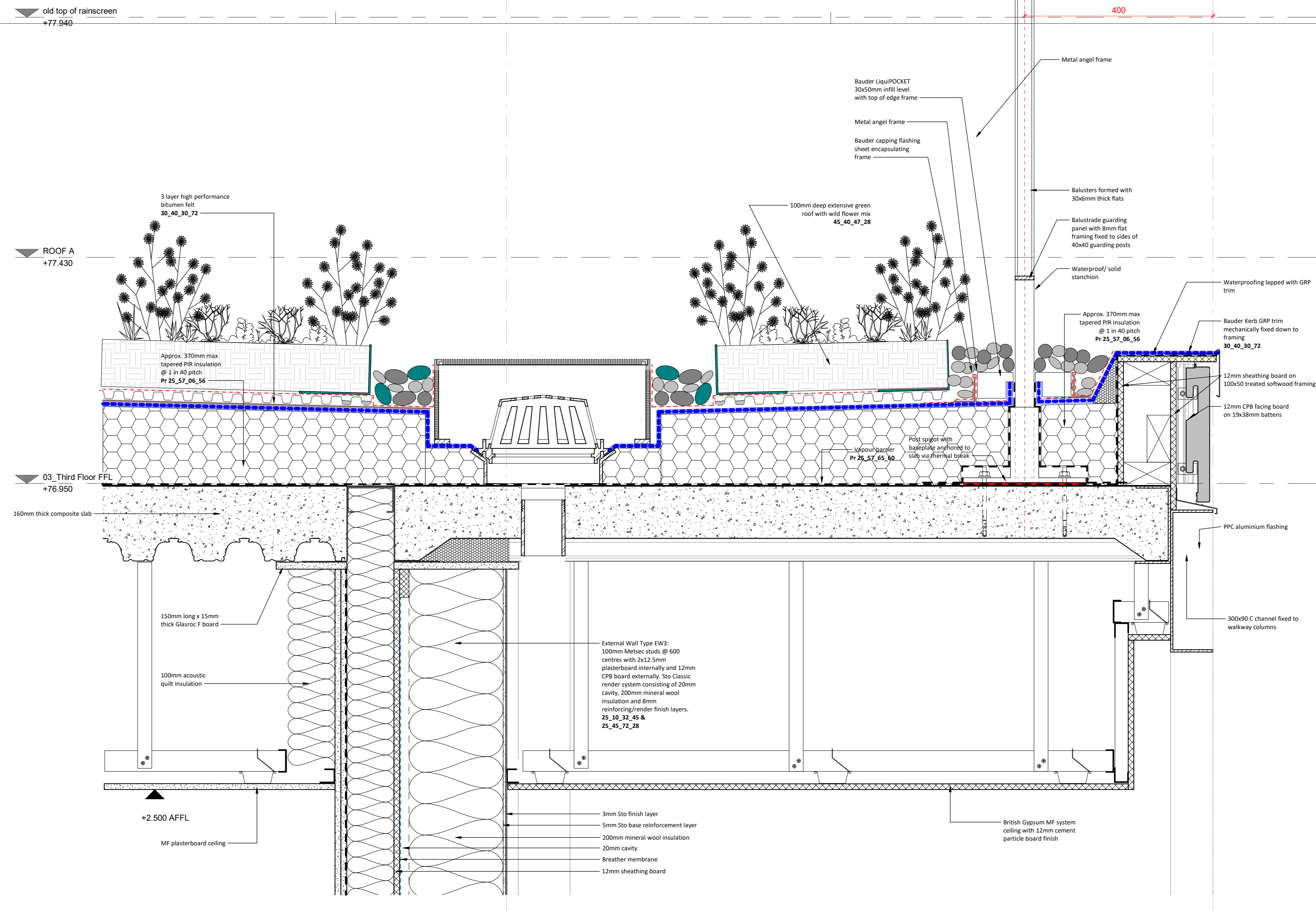
3 Typical Walkway/Sto Roof Section 1:5
