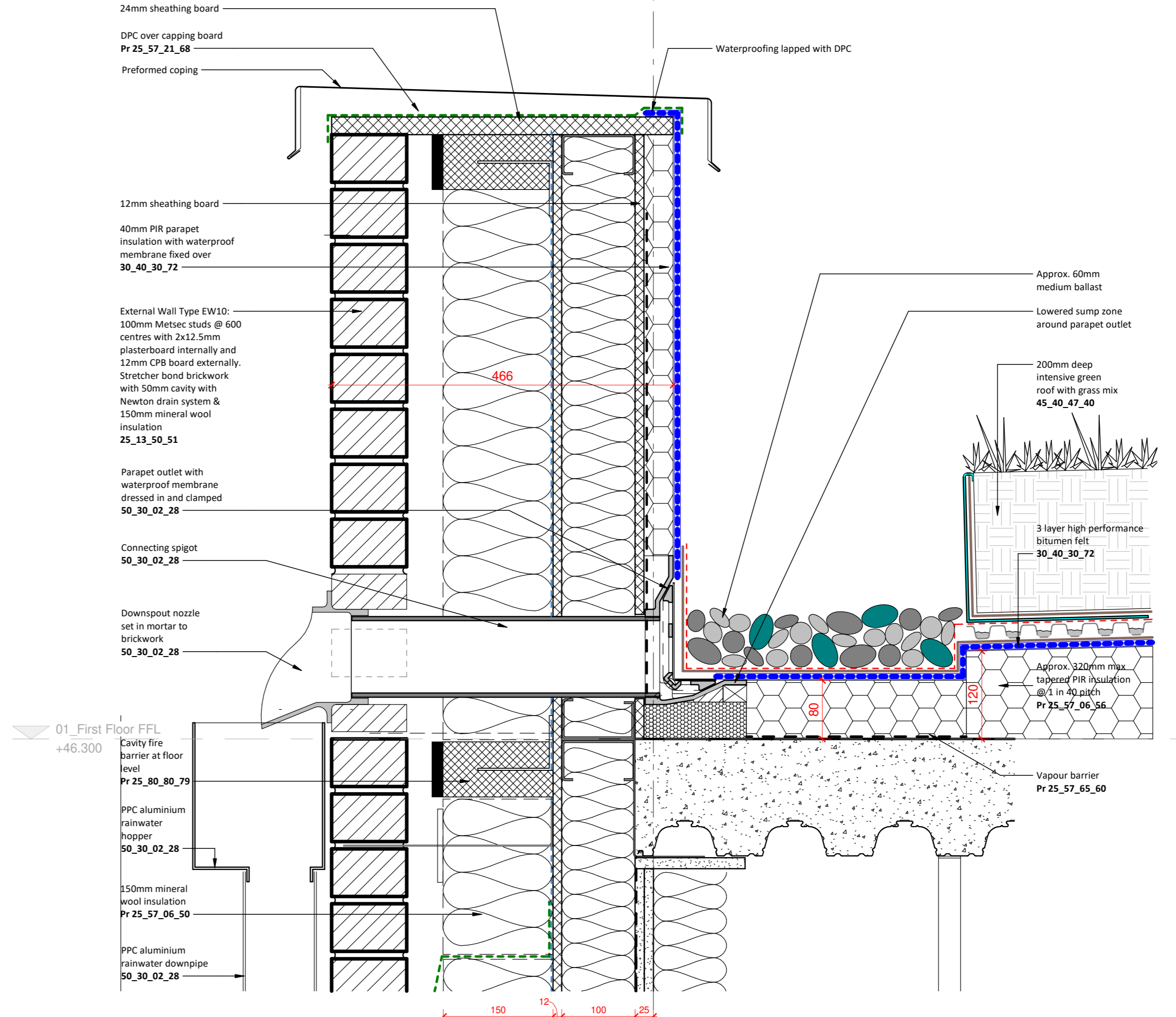
3 Accessible Unit Front Wall Parapet Detail 1 : 5
