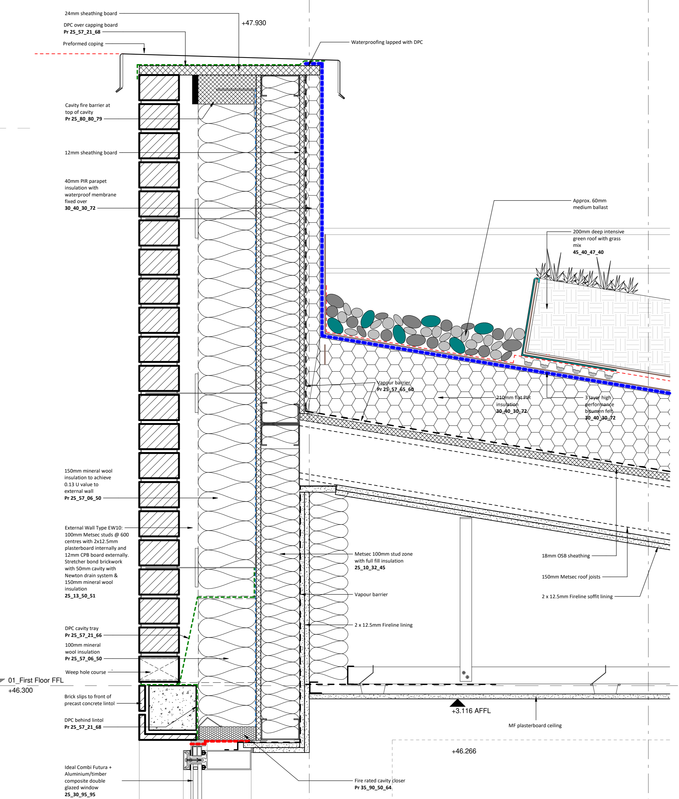
4 Community Room Front Wall Parapet Detail 1 : 5
