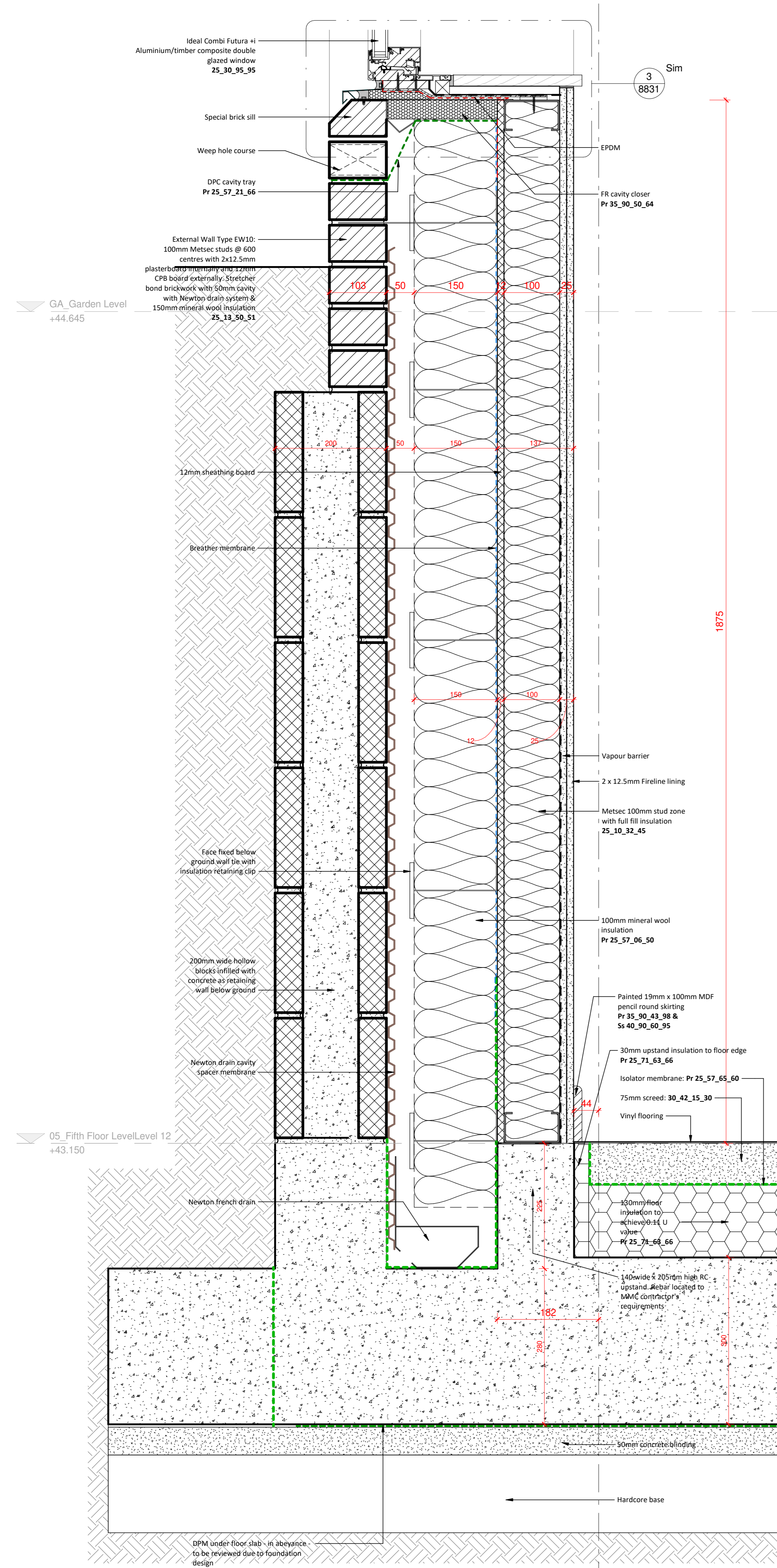
2 Accessible Unit Side Wall Base Detail 1 : 5
