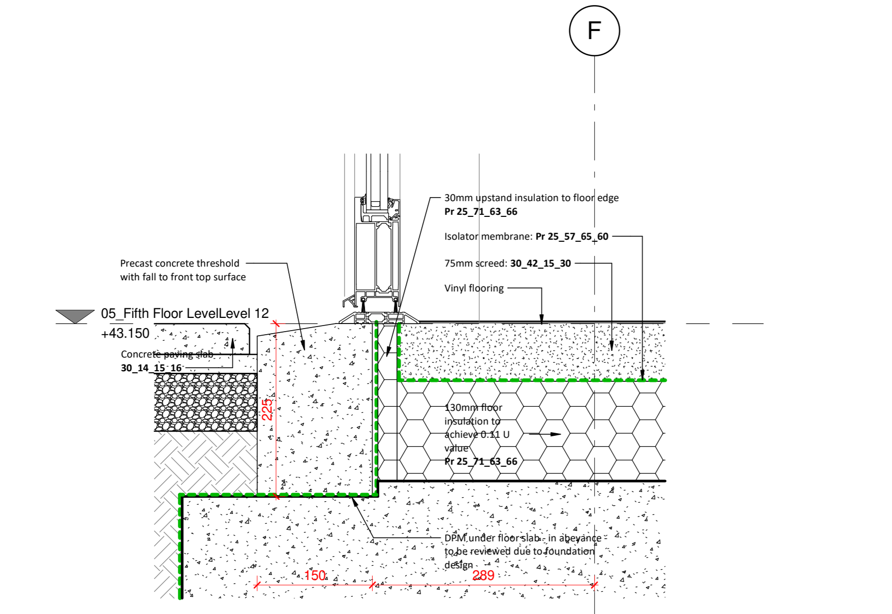
6 Community Room External Door Threshold Detail 1 : 5
