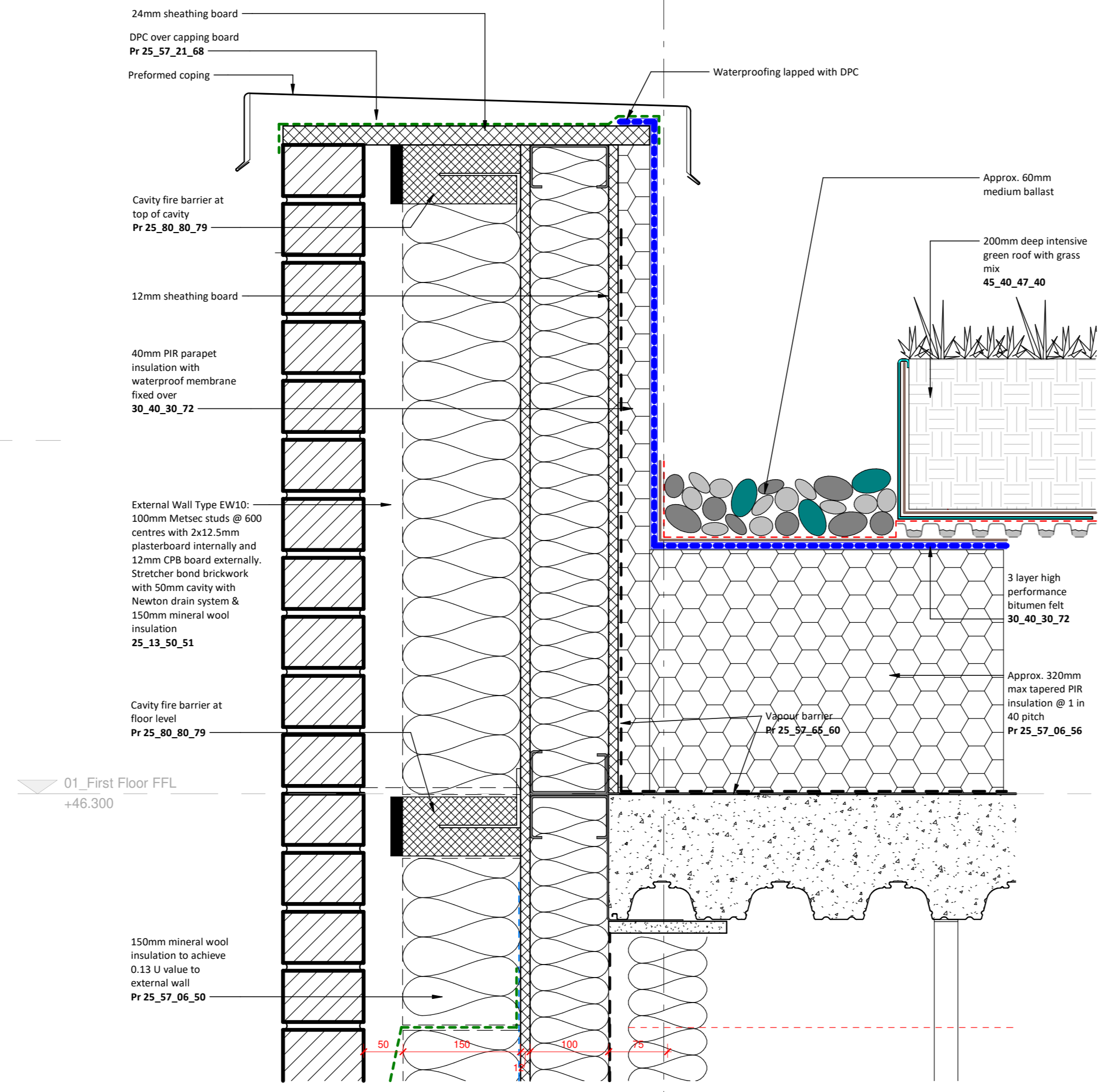
1 Accessible Unit Side Wall Parapet Detail 1 : 5
