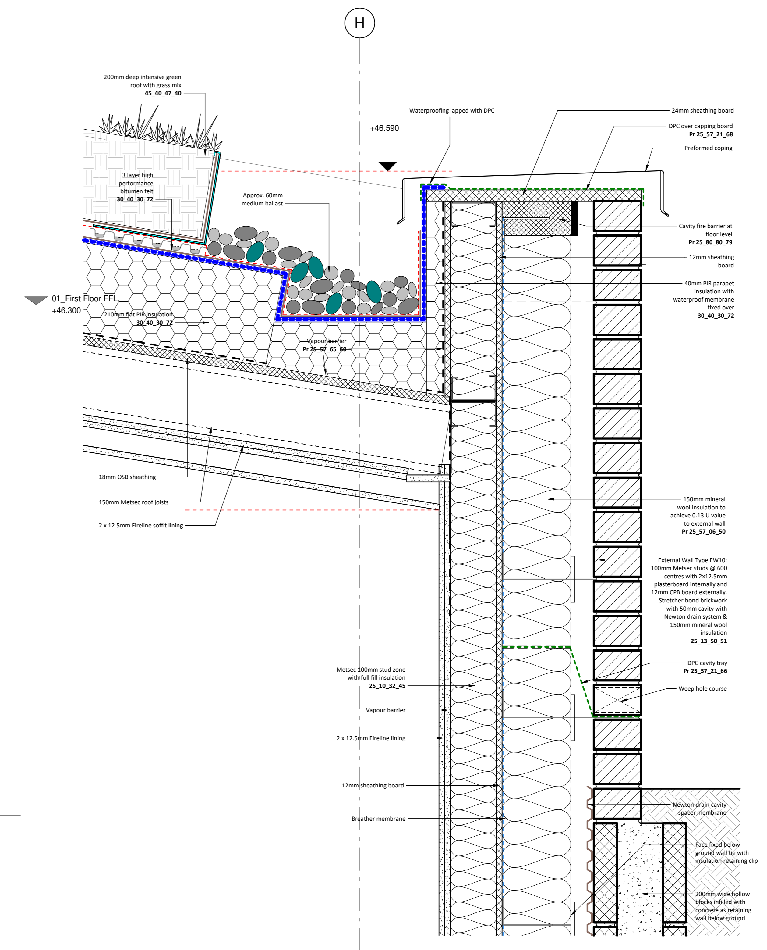
5 Community Room Rear Wall Parapet Detail 1 : 5
