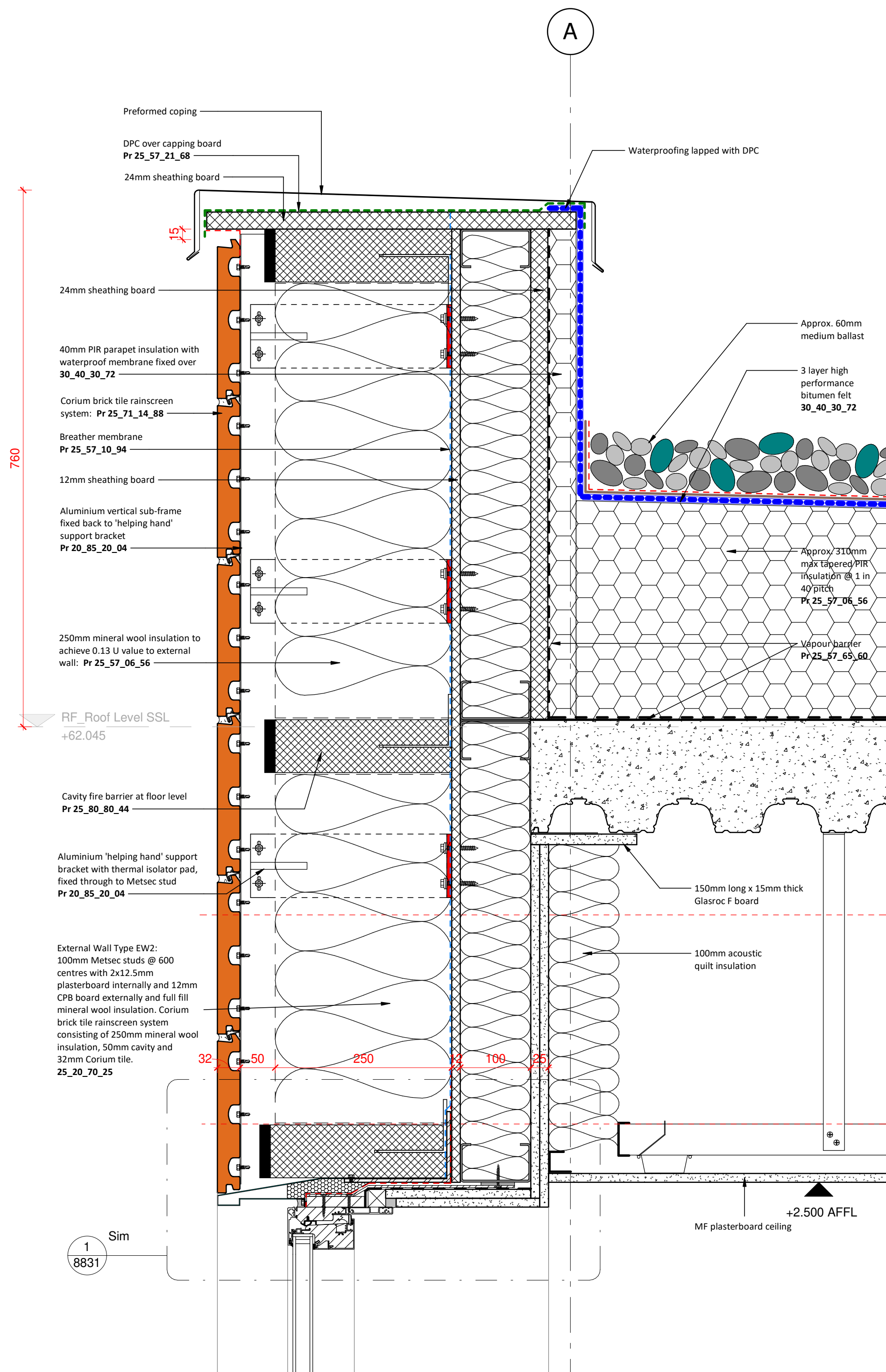
1 Corium Typical Top Parapet 1 : 5
