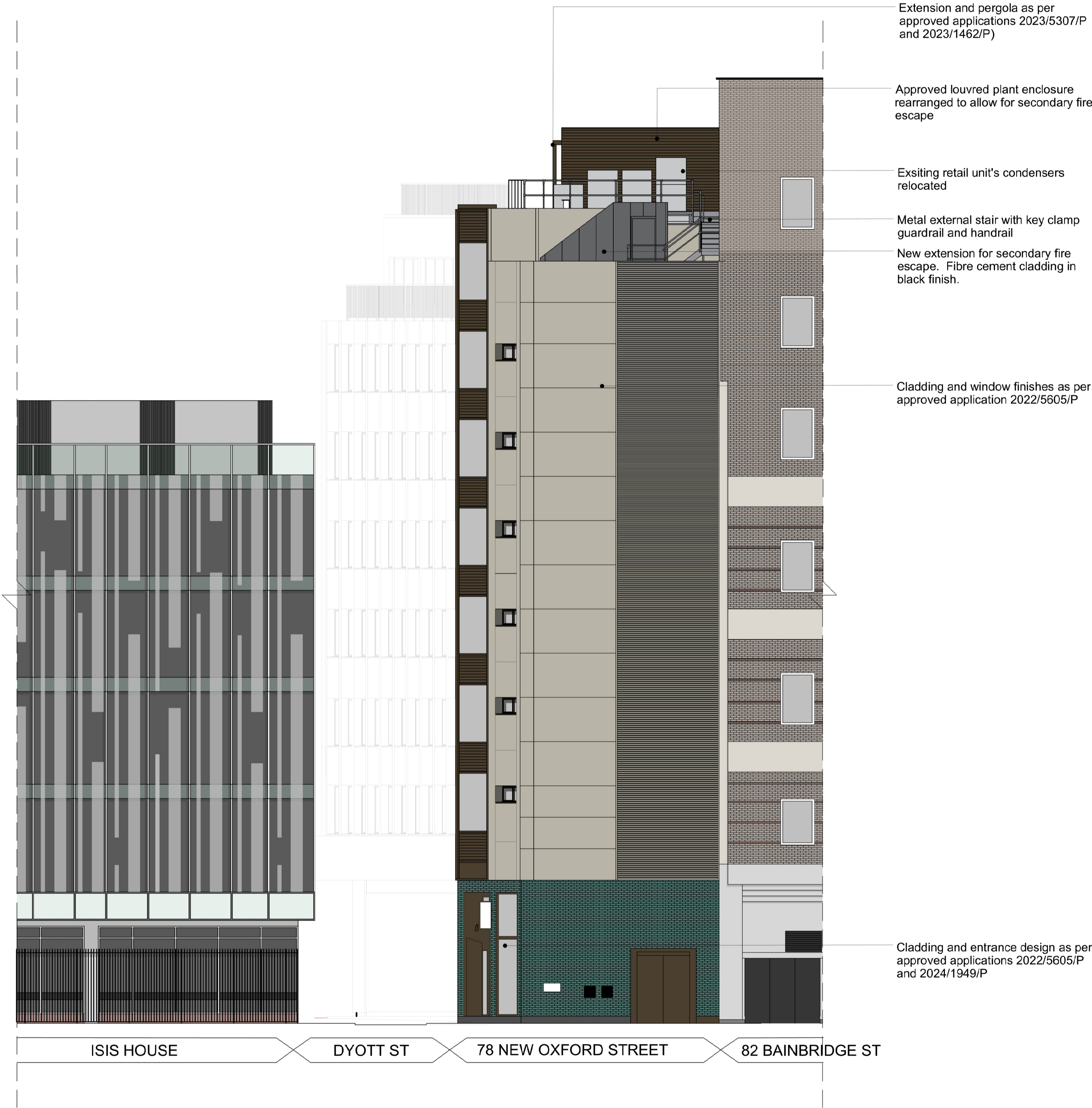
1 Proposed Bainbridge Street Elevation 1 : 100
