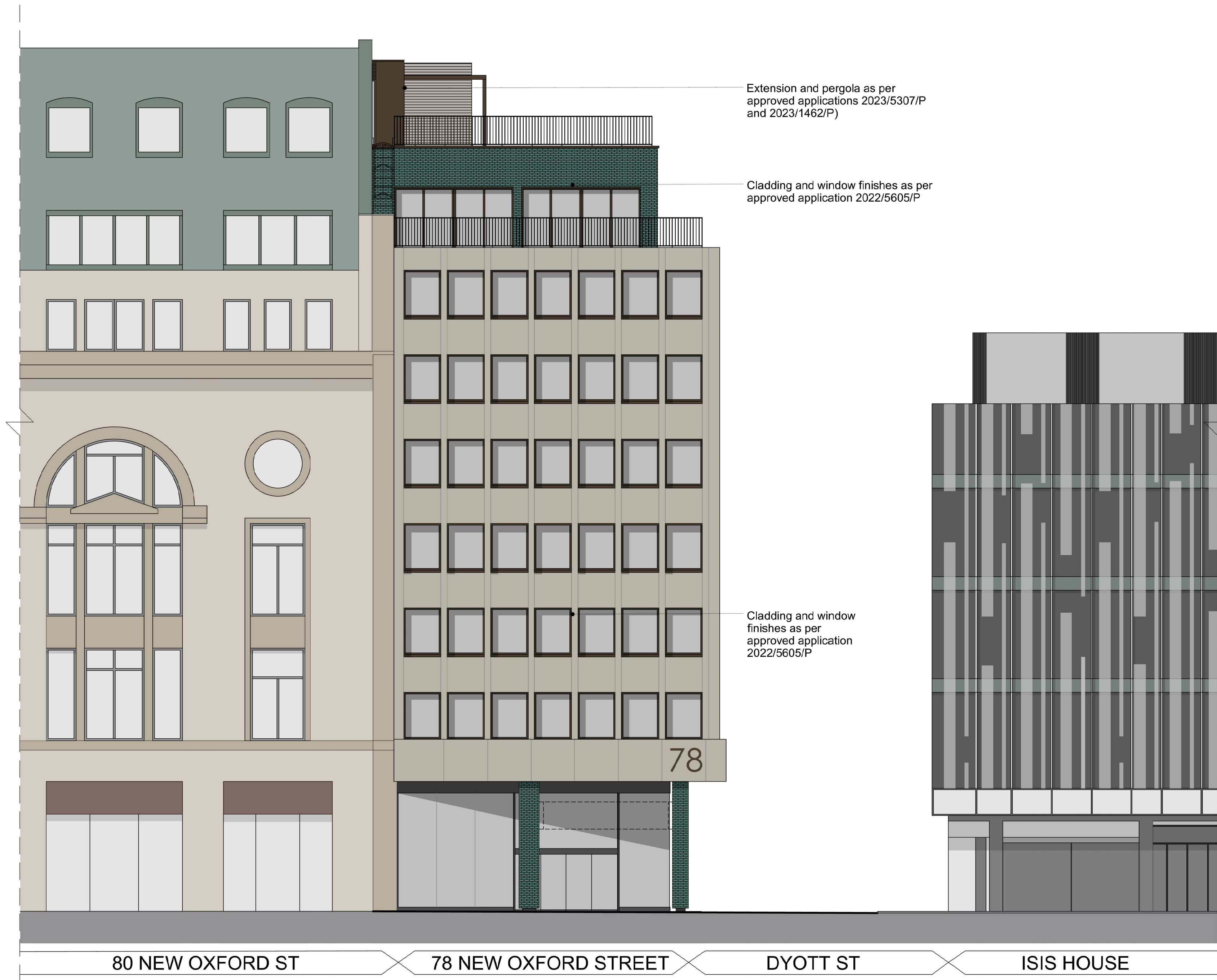
1 Proposed New Oxford Street Elevation 1 : 100
