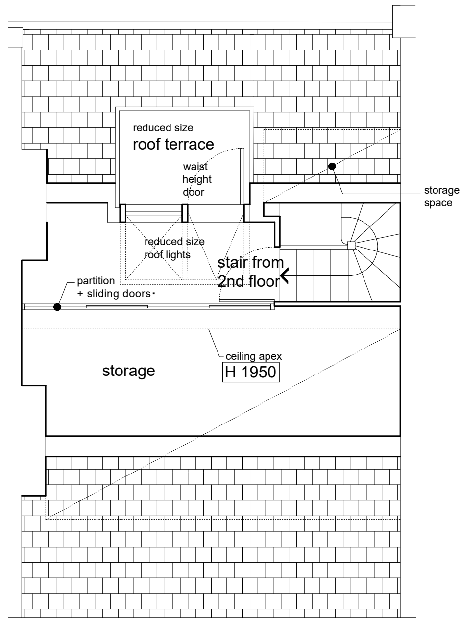
THIRD FLOOR PLAN LOFT + ROOF TERRACE PROPOSED
