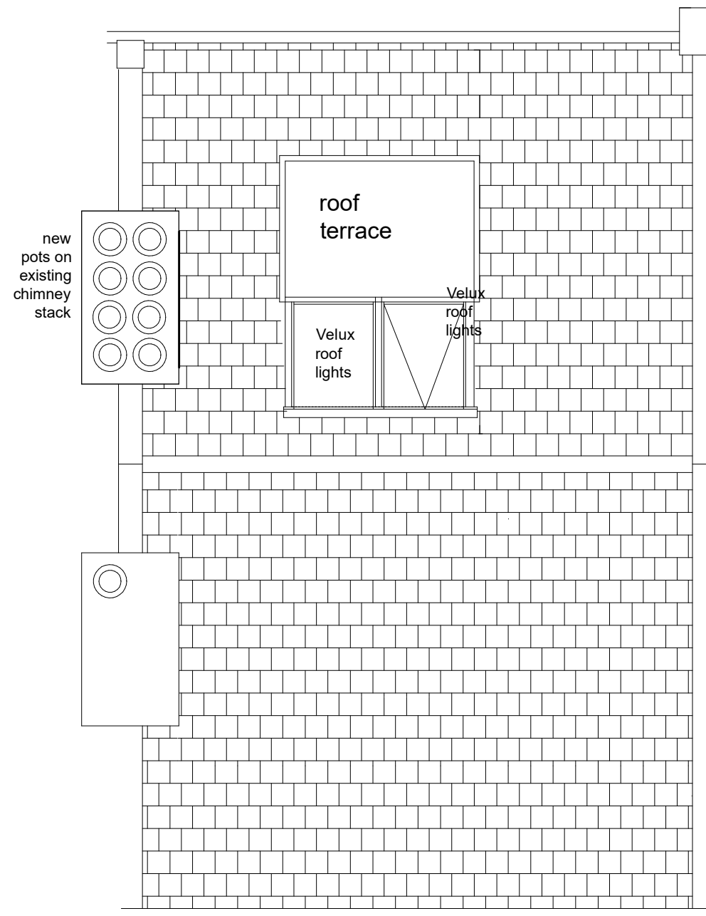
ROOF PLAN PROPOSED
