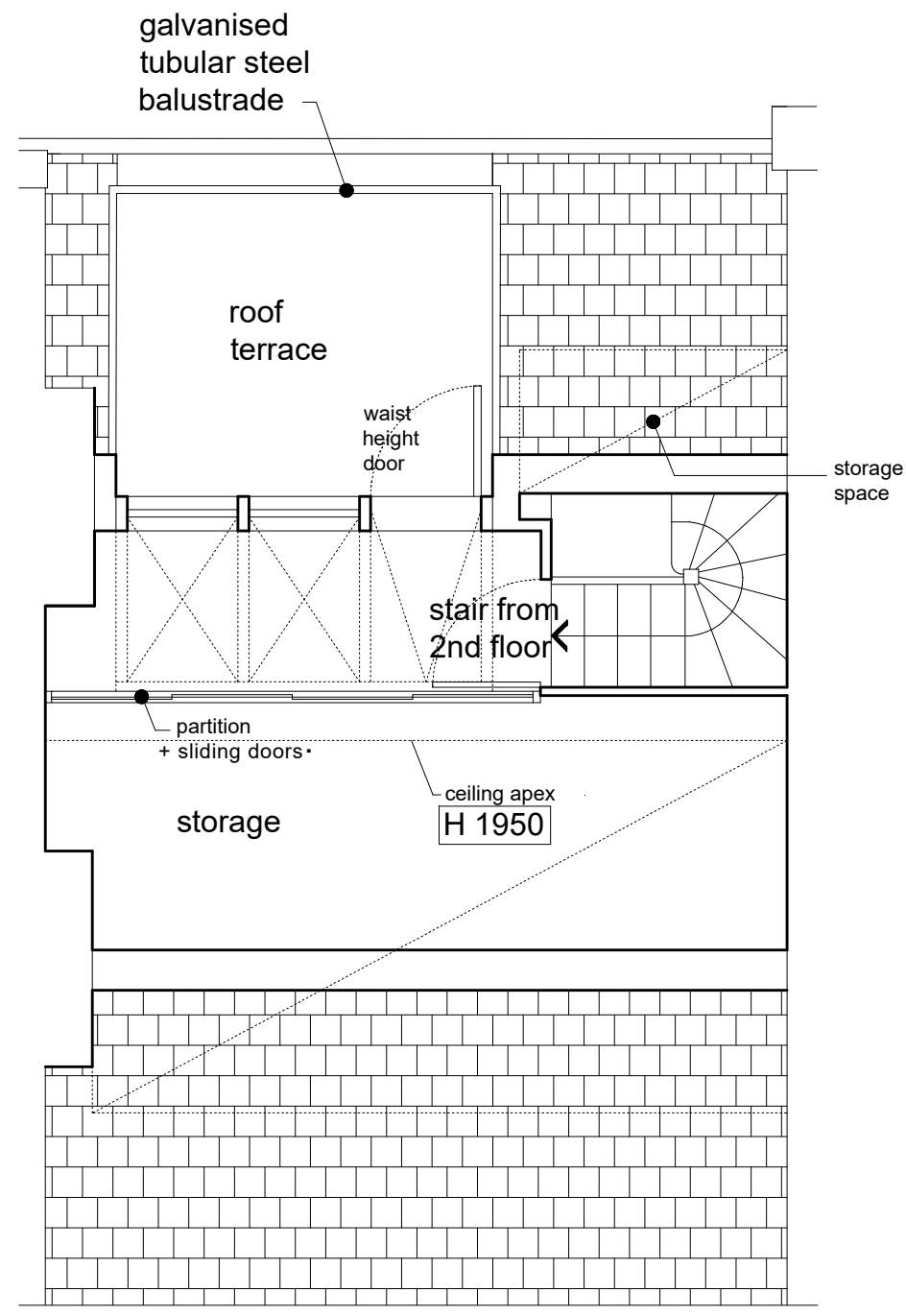
THIRD FLOOR PLAN LOFT + ROOF TERRACE EXISTING
