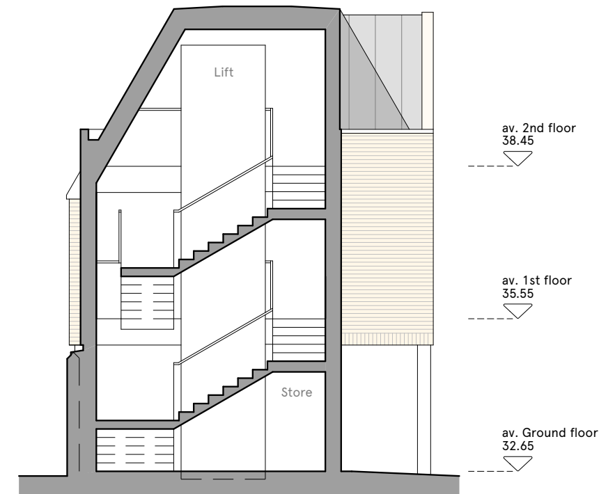
Section C-C
