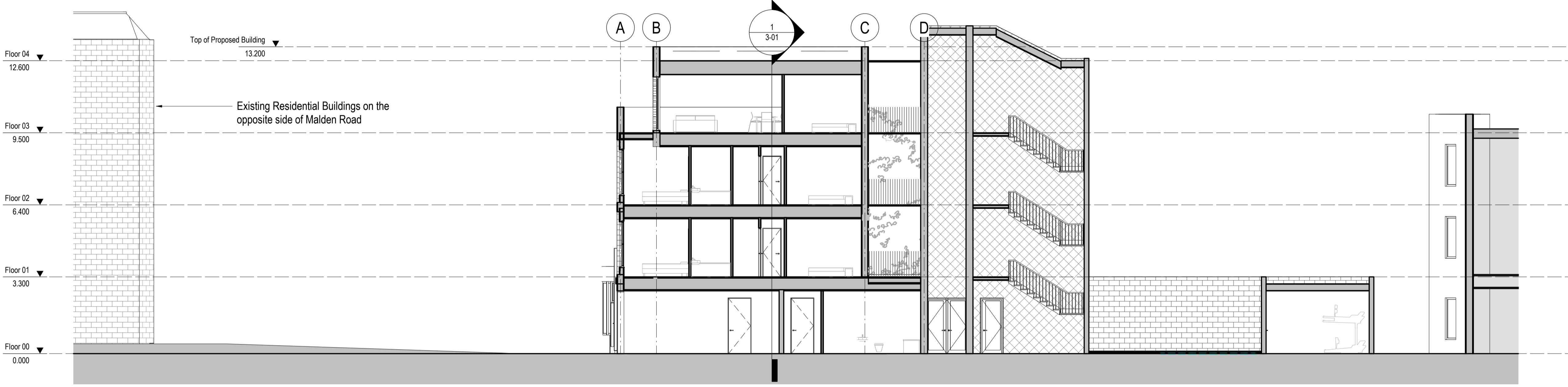
2 Section 2 1:100
