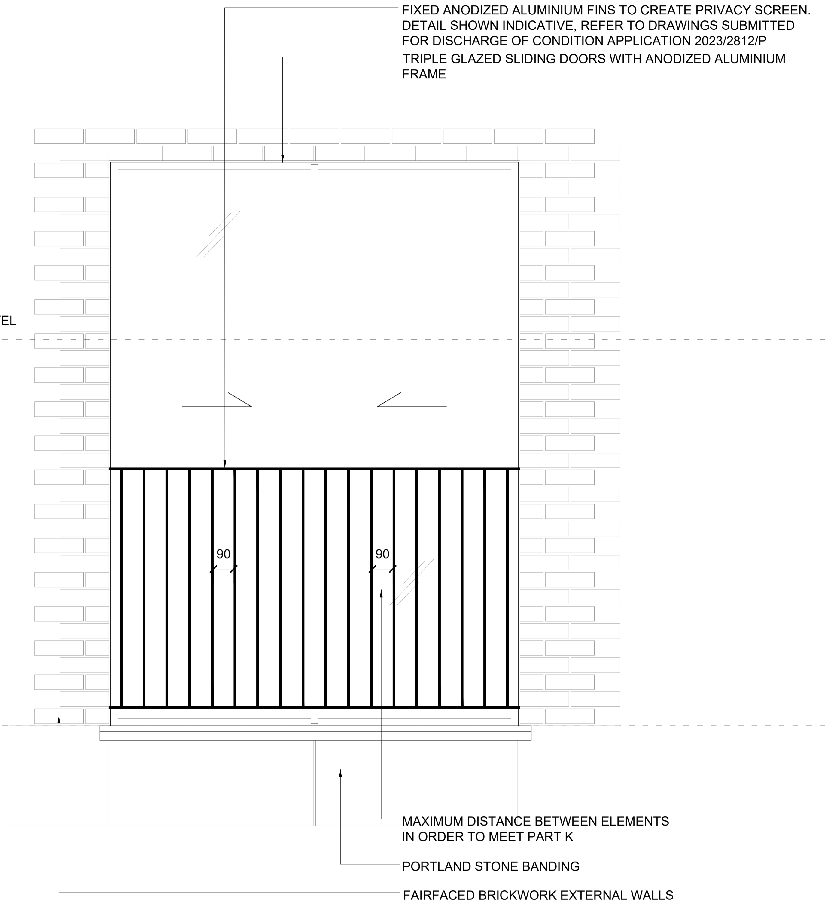
ELEVATION - Typical Window Assembly Type B Showing Aluminium Fins.
