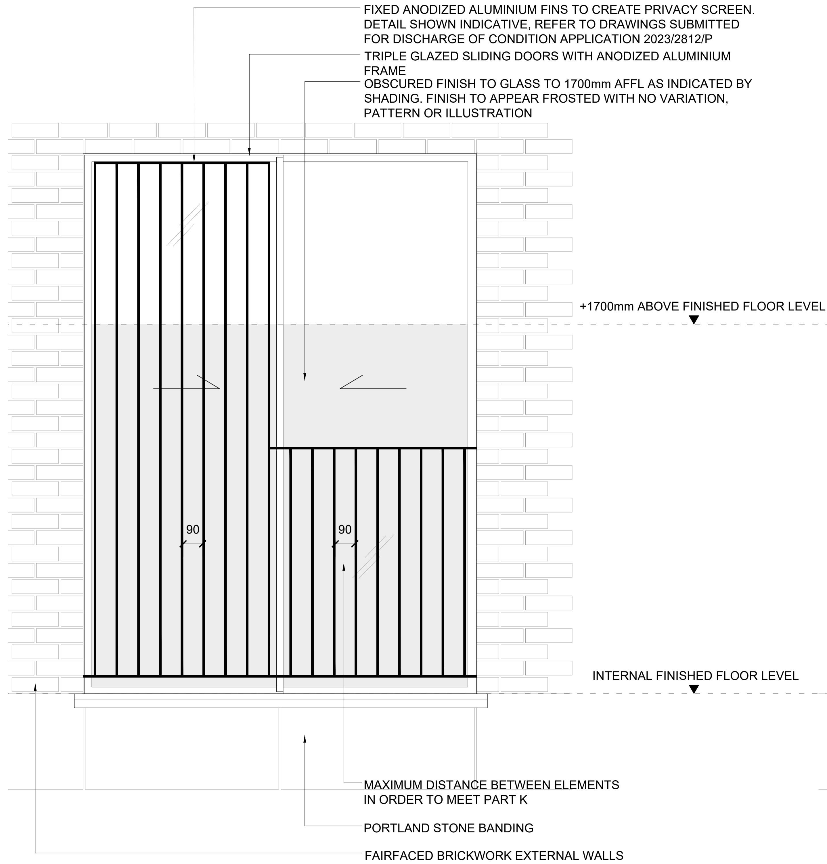
ELEVATION - Typical Window Assembly Type A Showing Aluminium Fins.
