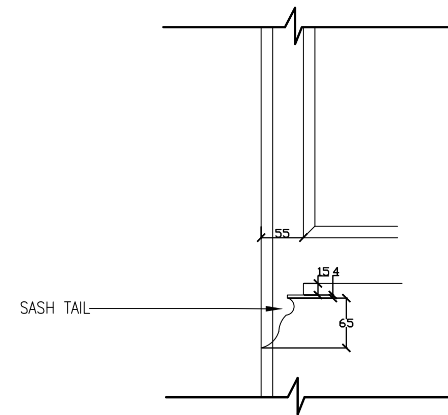
SASH TAIL DETAIL
