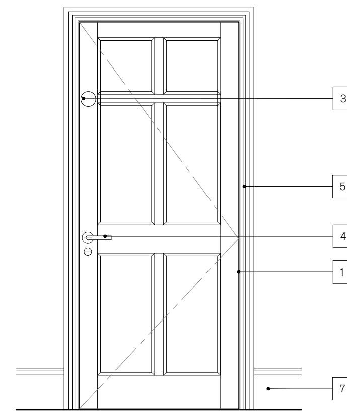
DOOR TYPE B Raised & fielded 6 panel Refer to Schedule CO.3300 Series for Fire Ratings and smoke seals
