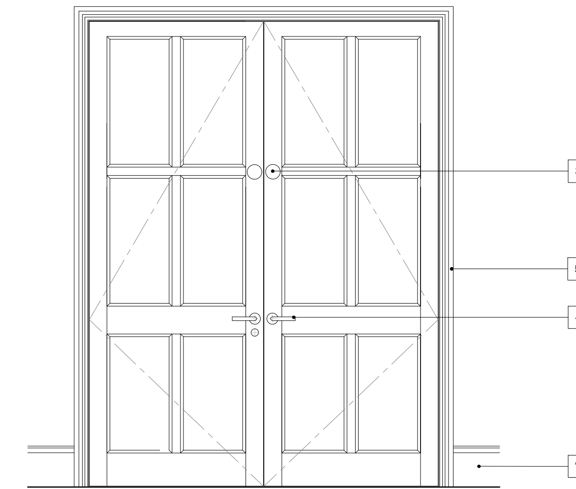
DOOR TYPE D Raised & fielded 6 panel double doors Refer to Schedule CO.3300 Series for Fire Ratings and smoke seals
