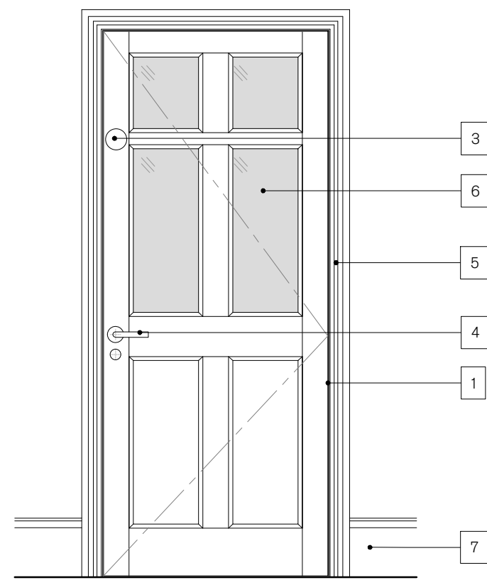
DOOR TYPE A Raised & fielded 6 panel with Glazed Vision Panels Refer to Schedule CO.3300 Series for Fire Ratings and smoke seals
