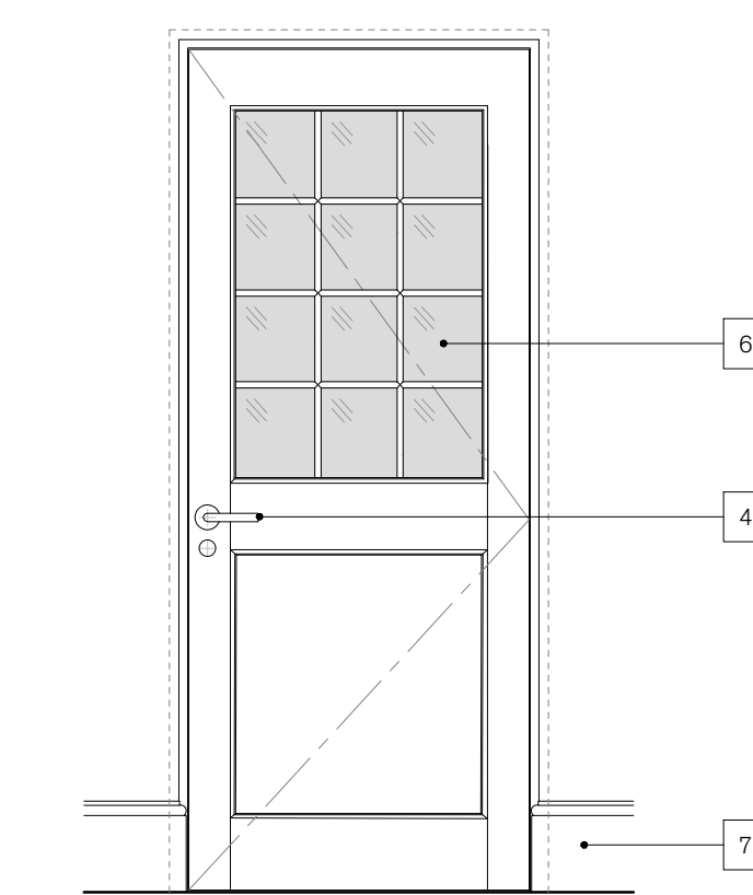
DOOR TYPE G Half glass raised & fielded 2 panel with planted bars External Door.
