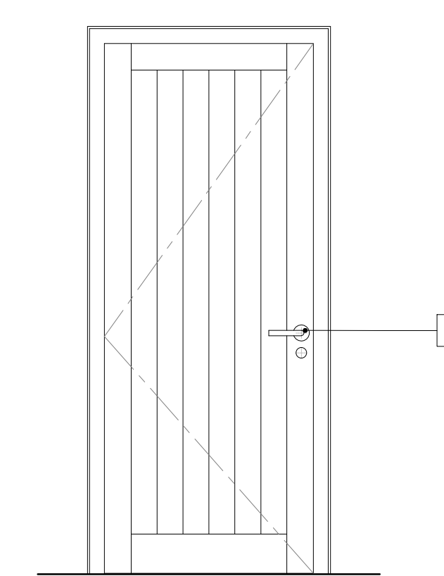
DOOR TYPE H Vertically boarded external door.
