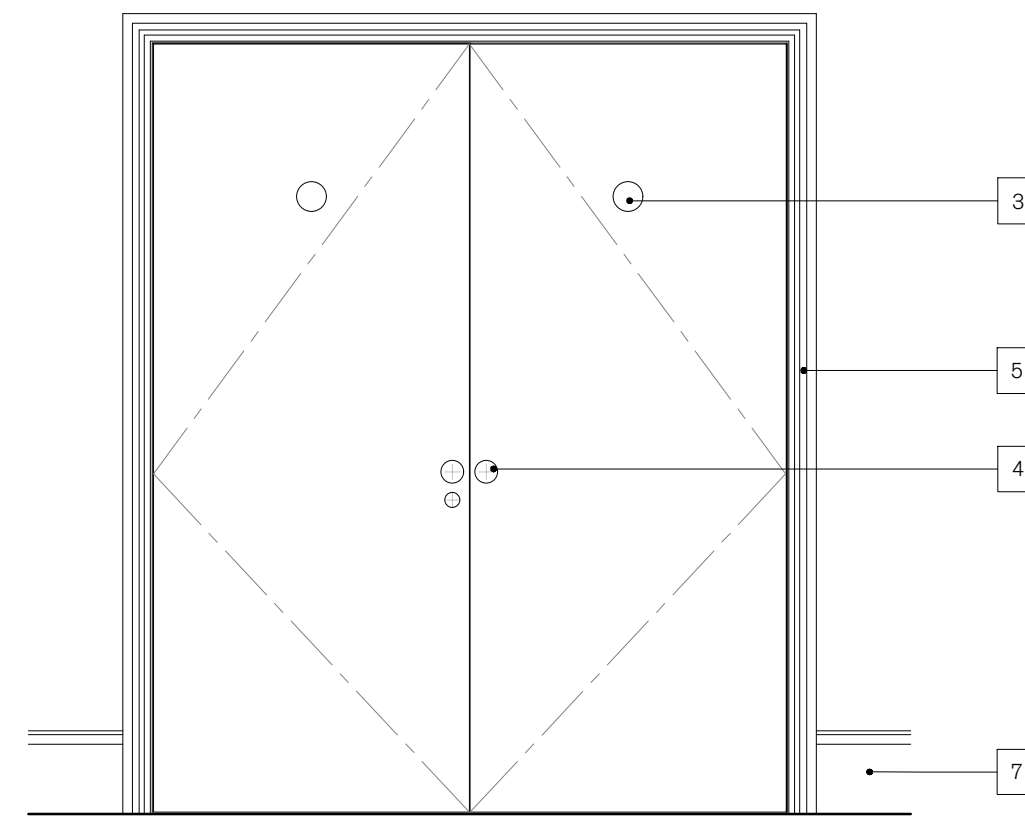
DOOR TYPE C Internal flush double doors. Refer to Schedule CO.3300 Series for Fire Ratings and smoke seals
