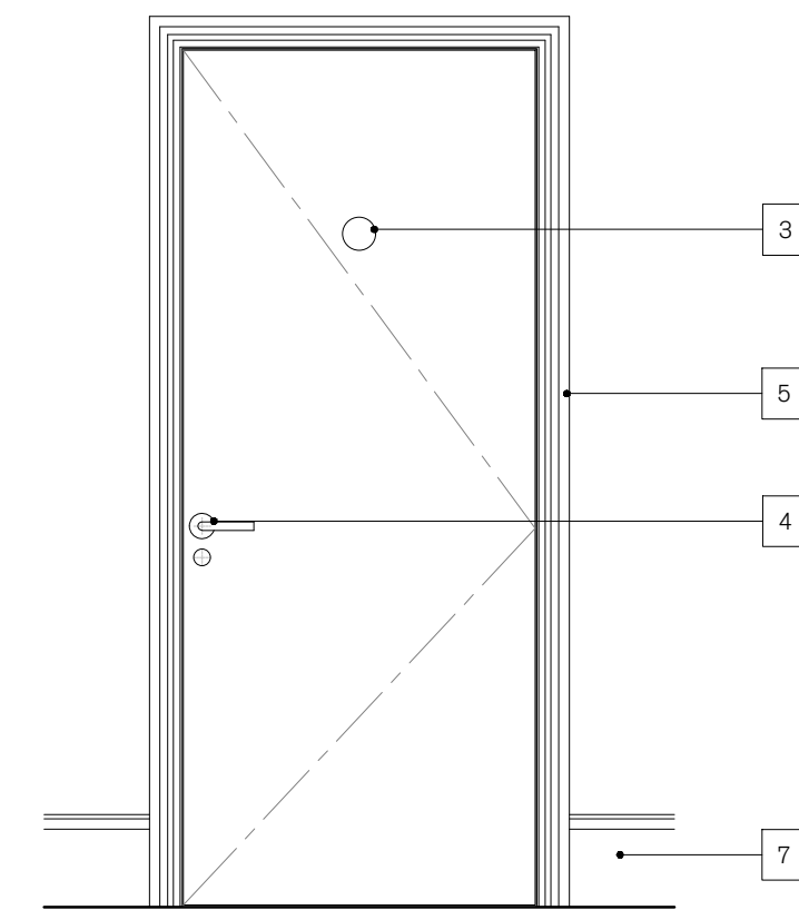
DOOR TYPE E Single leaf internal flush door. Refer to Schedule CO.3300 Series for Fire Ratings and smoke seals
