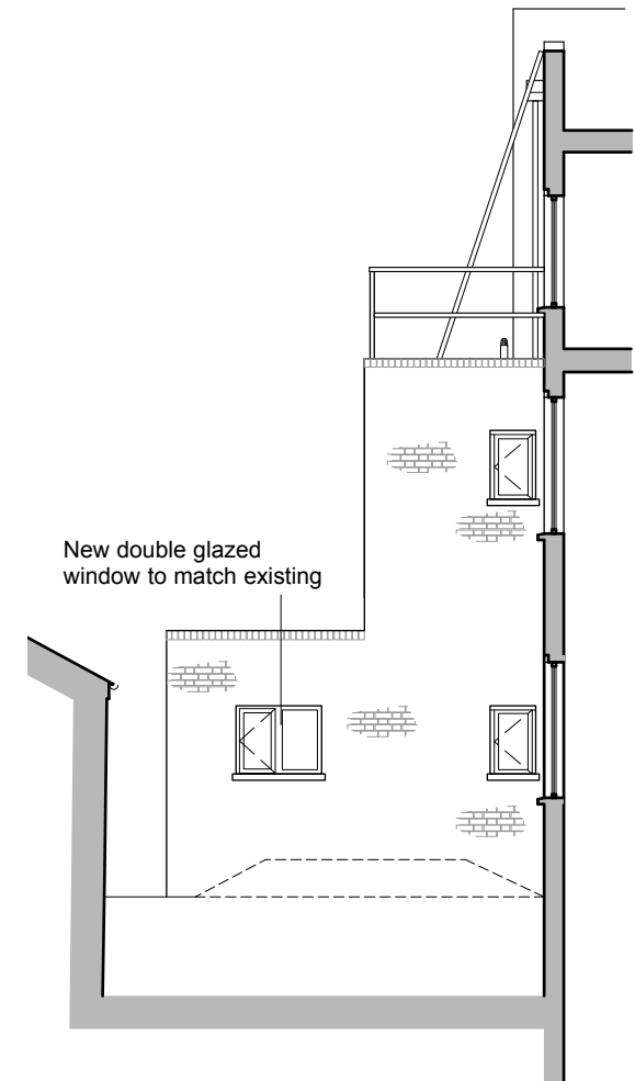
EAST ELEVATION
