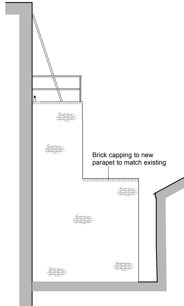
WEST ELEVATION
