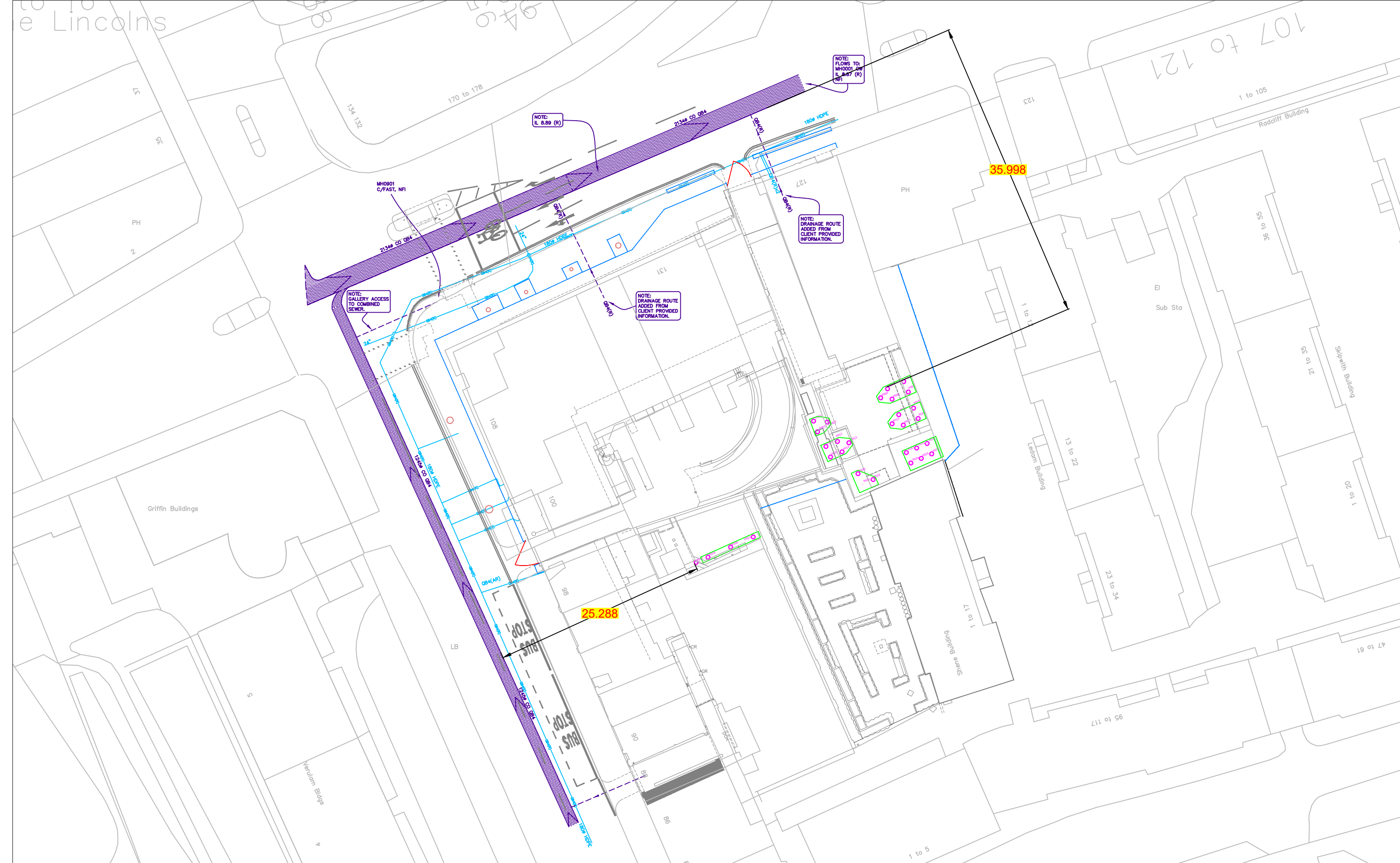
100GIR Proposed Piles Position vs Existing Sewer and Water supply 22.07.2024
