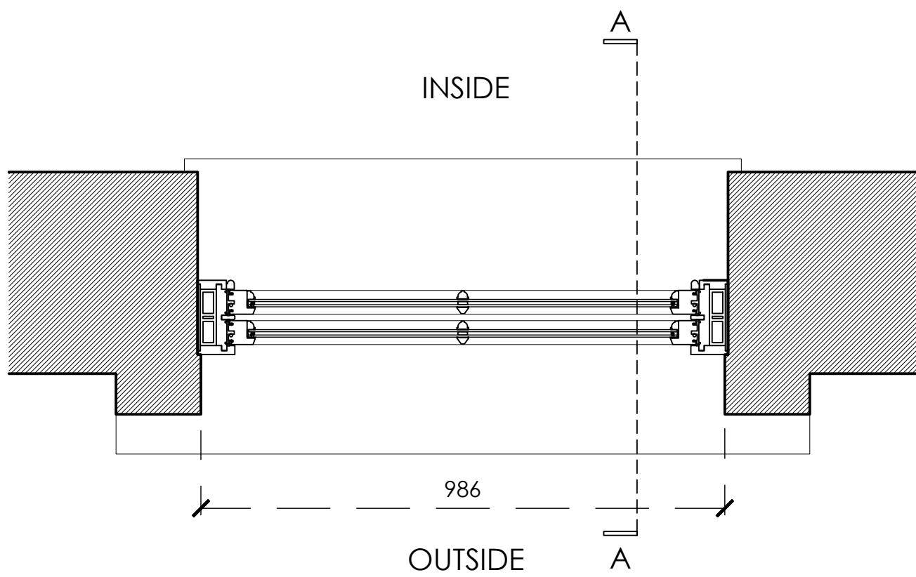
Front Dormer Window Elevation
