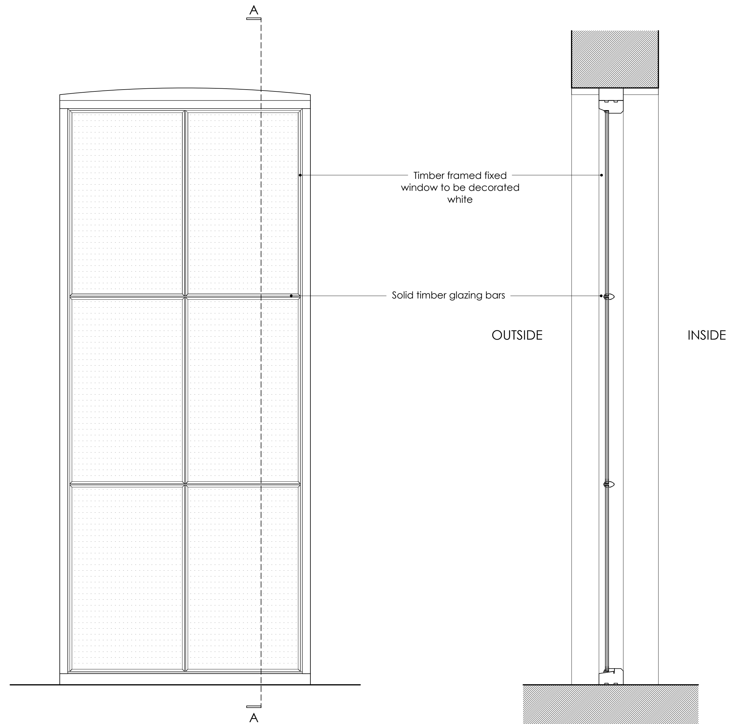
Window 4 Section AA
