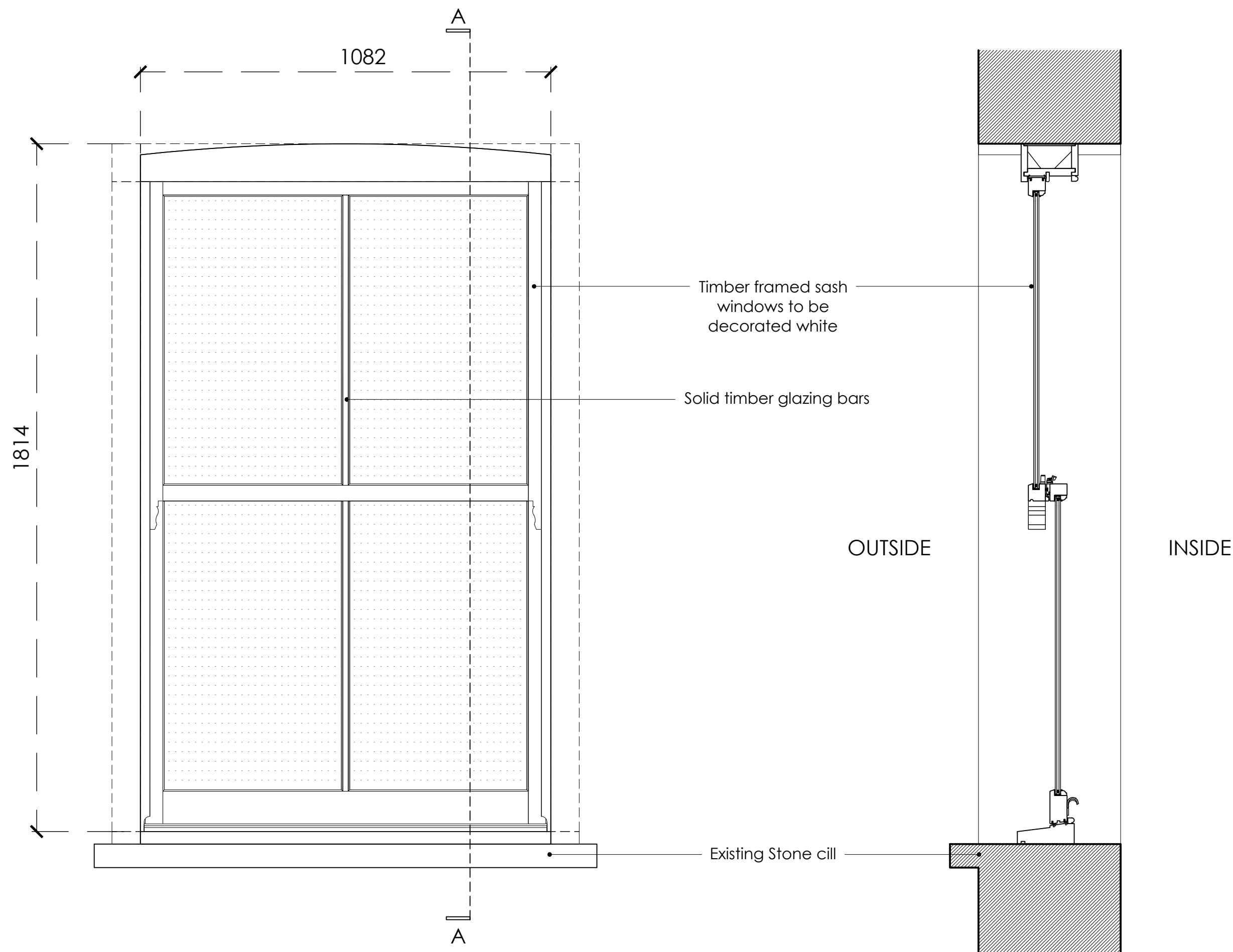
Window 3 Section AA
