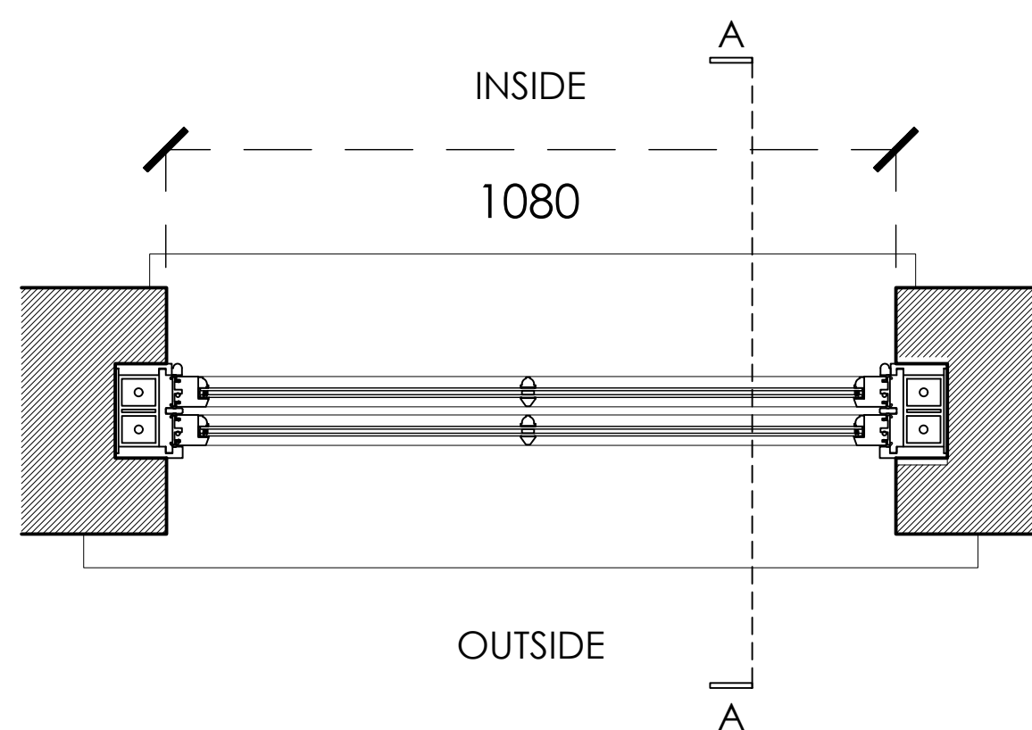
Window 3 Plan
