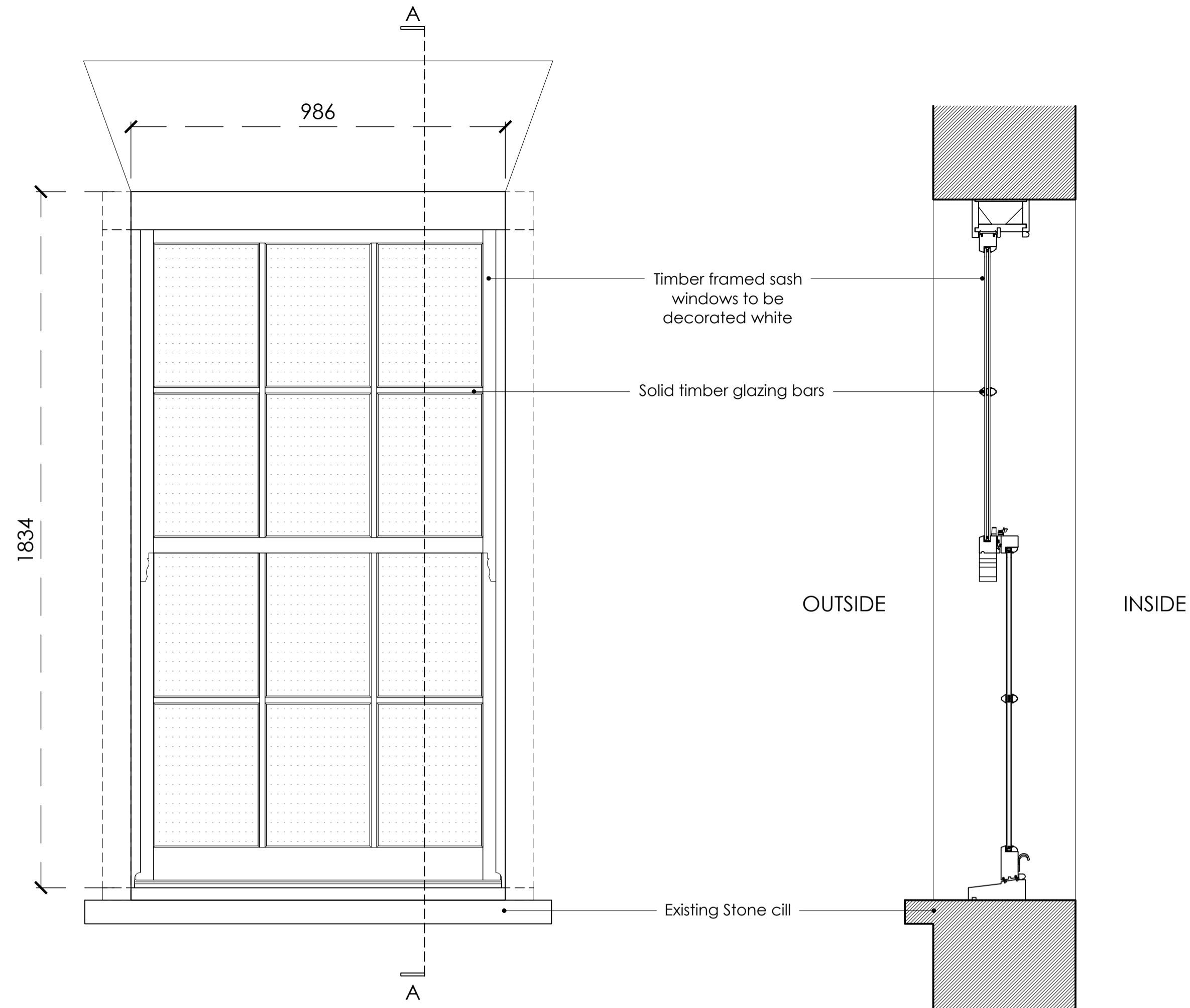
Window 1 Section AA
