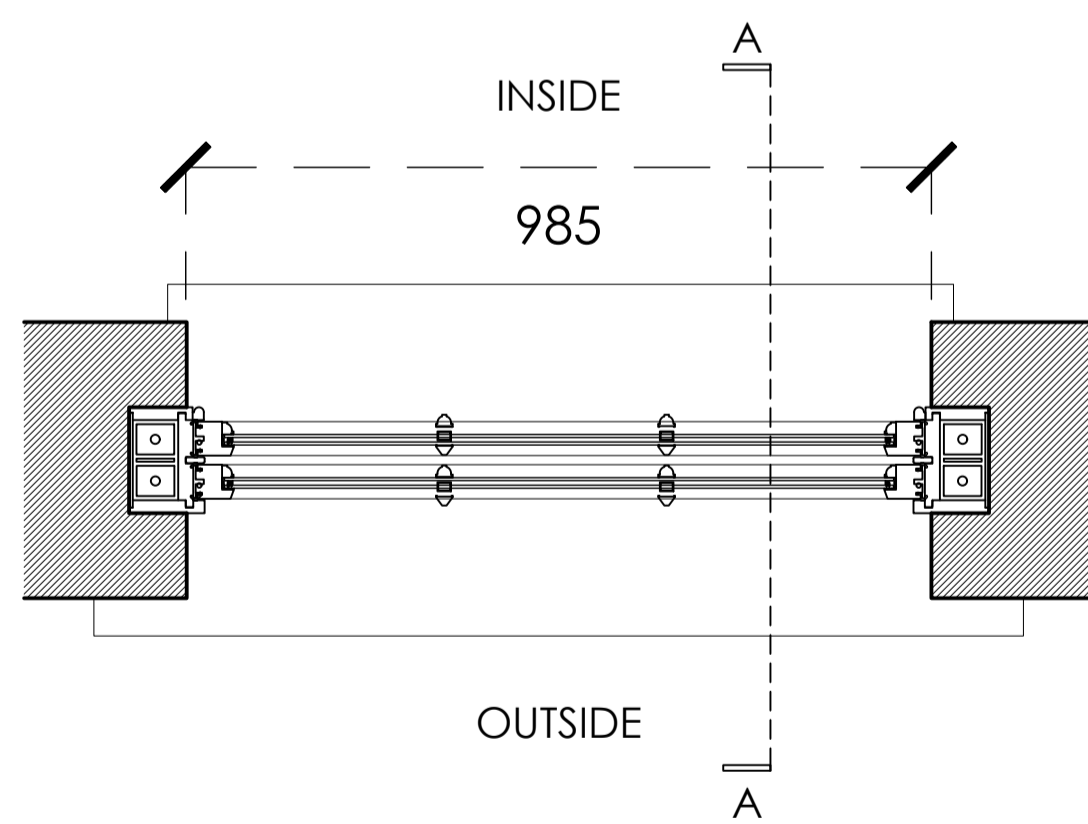
Window 1 Plan
