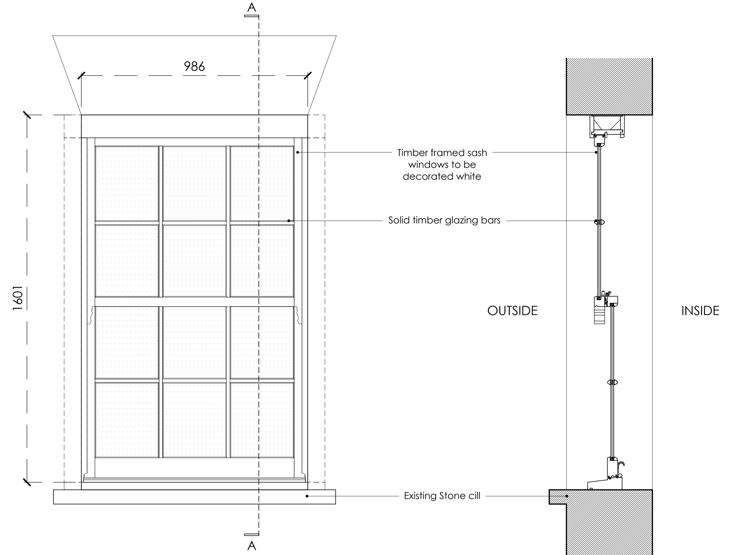
Window 2 Section AA
