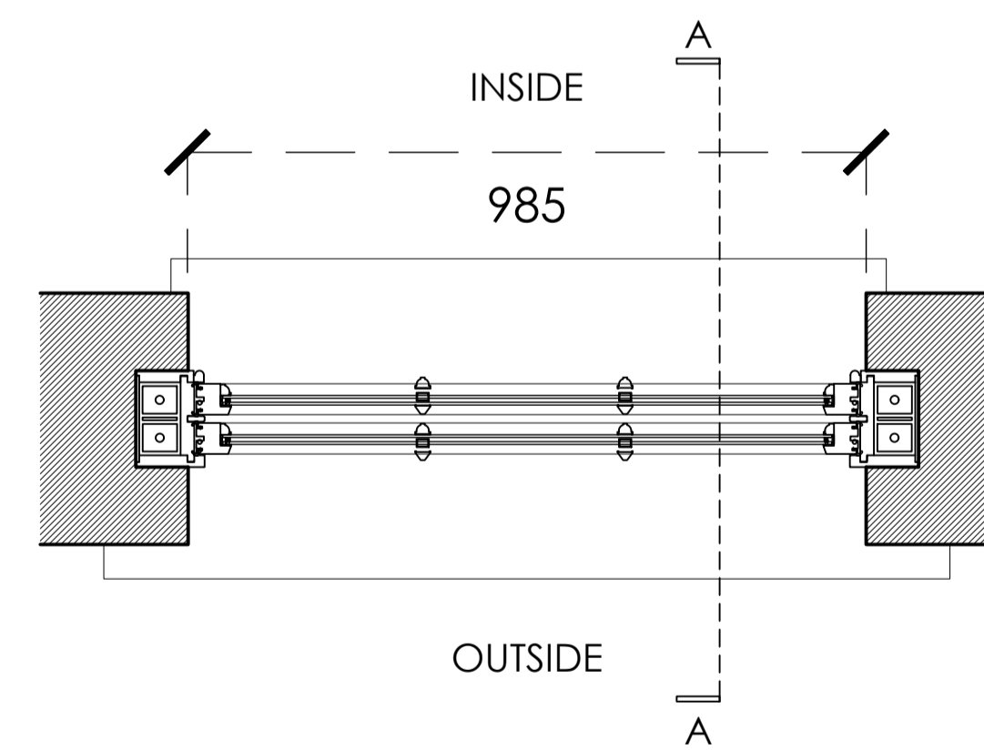
Window 2 Plan
