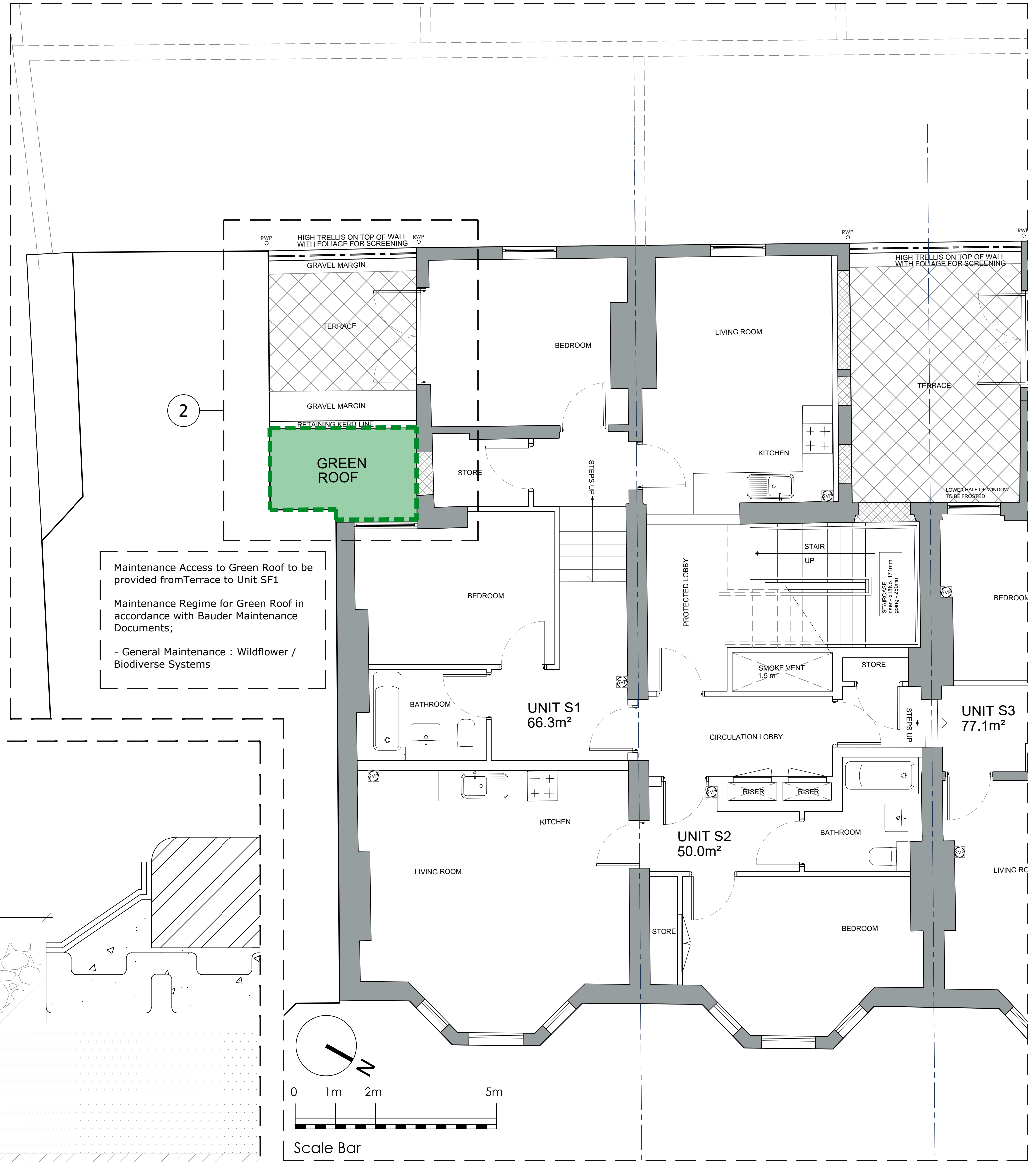
1 SECOND FLOOR GA Scale: 1:50
