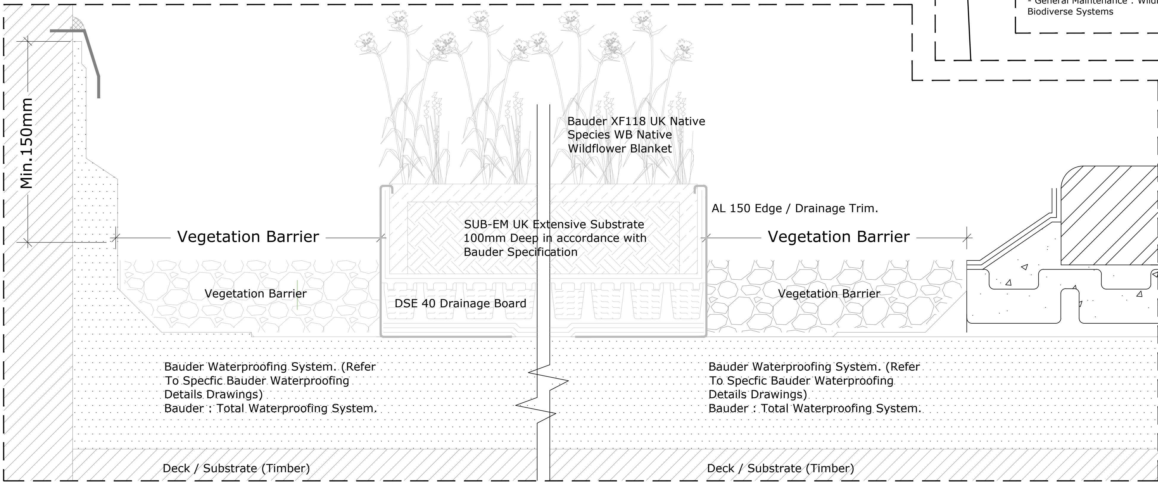
3 GREEN ROOF DETAIL Scale: 1:5
