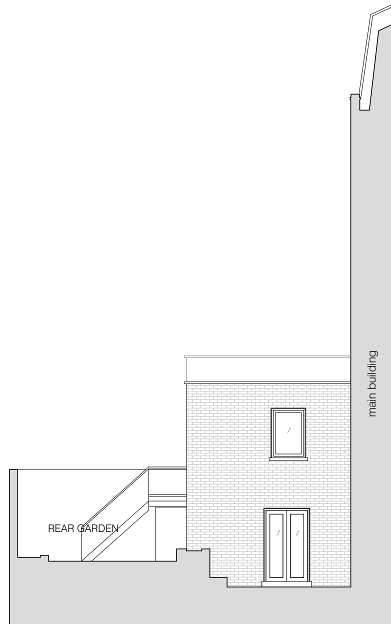
01 EXISTING SIDE ELEVATION/ SECTION B-B scale 1:100
