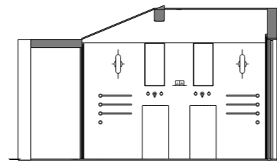
ELEVATION 03
