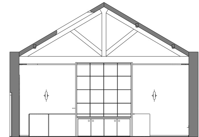
ELEVATION 03
