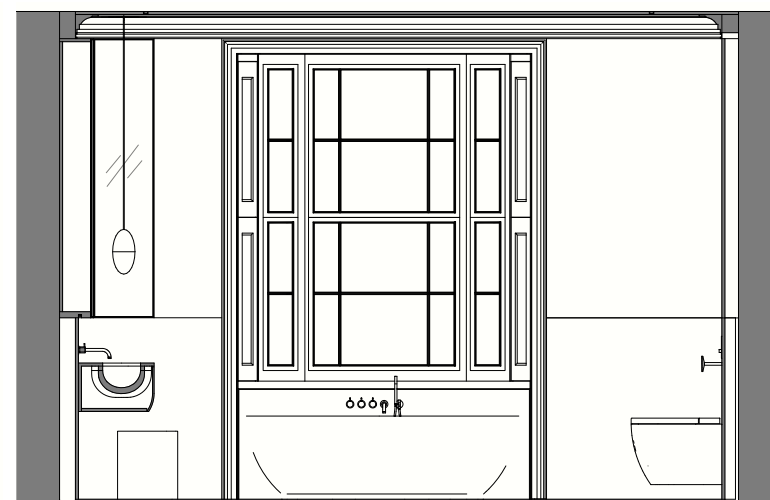
ELEVATION 02, 1:50 @ A3
