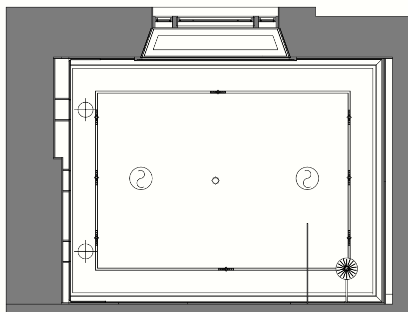
PROPOSED RCP, 1:50 @ A3
