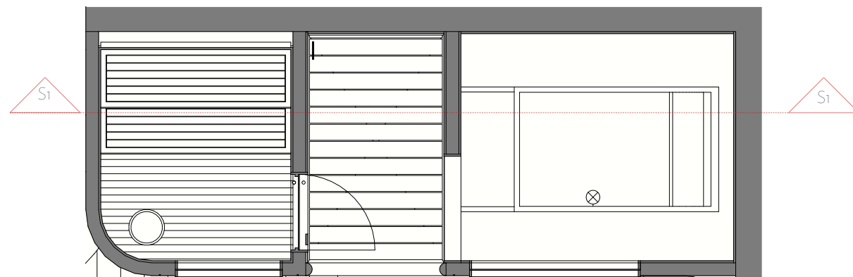
PROPOSED PLAN, 1/50 @ A3
