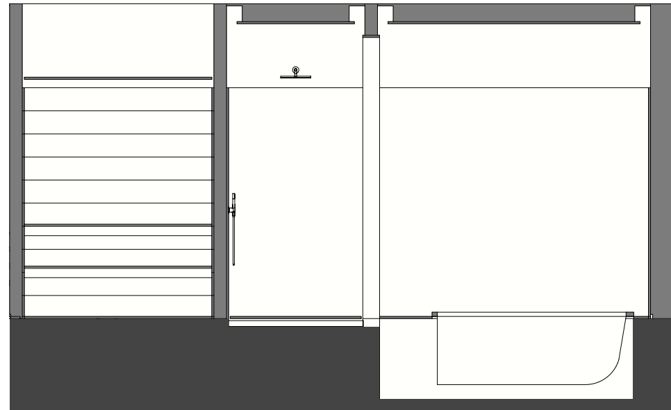
PROPOSED SECTION 01, 1/50 @ A3
