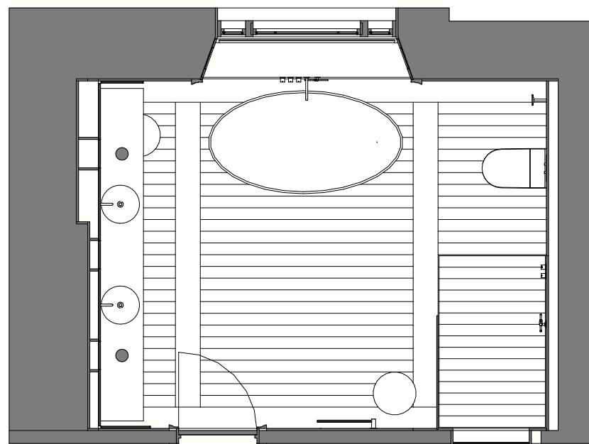
PROPOSED PLAN, 1:50 @ A3
