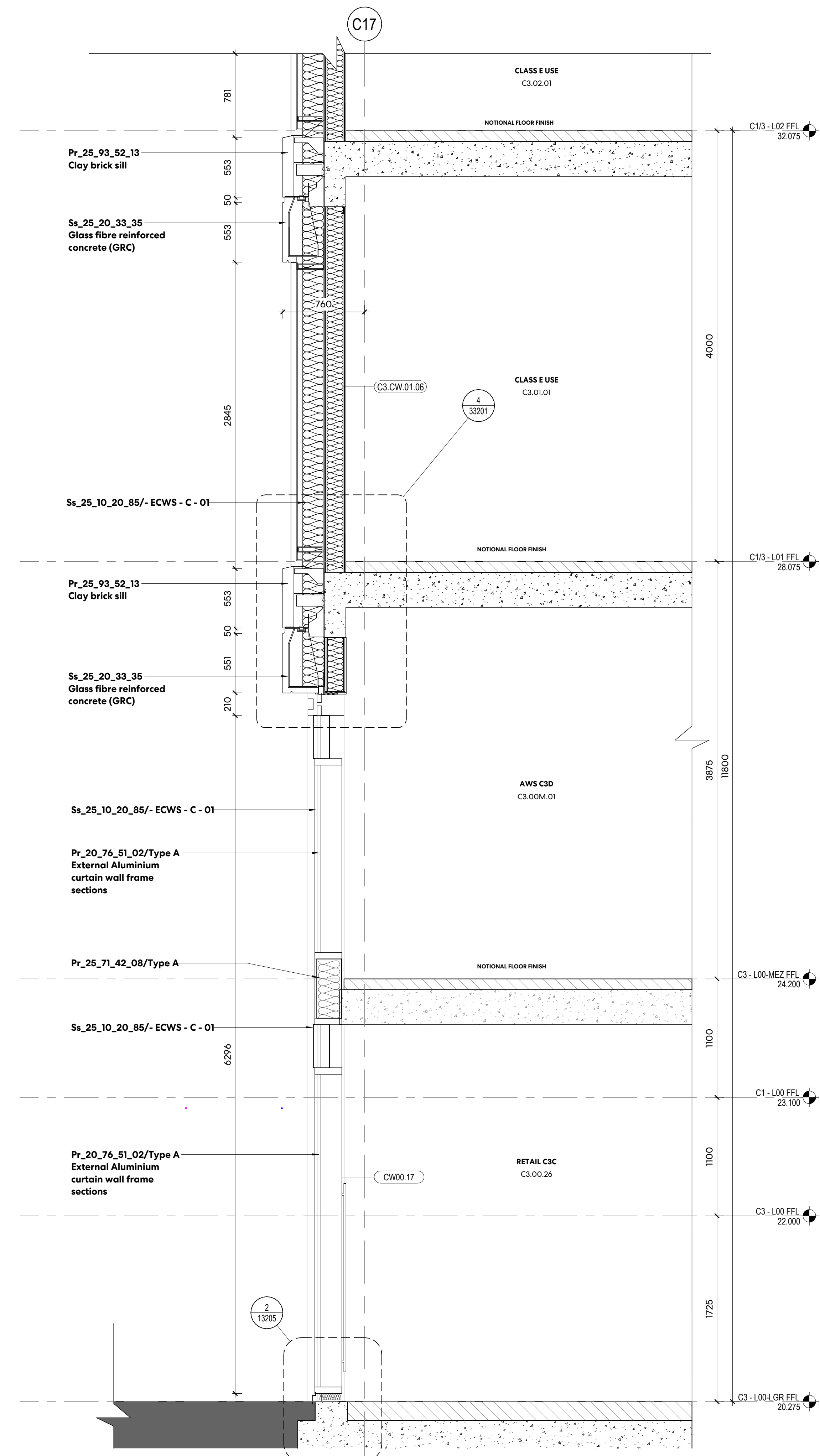
3 C3 - TYPICAL LOWER LEVEL BAY WITH CONCRETE FIN - LEVEL 00-02 - ENLARGED SECTION 1 : 25
