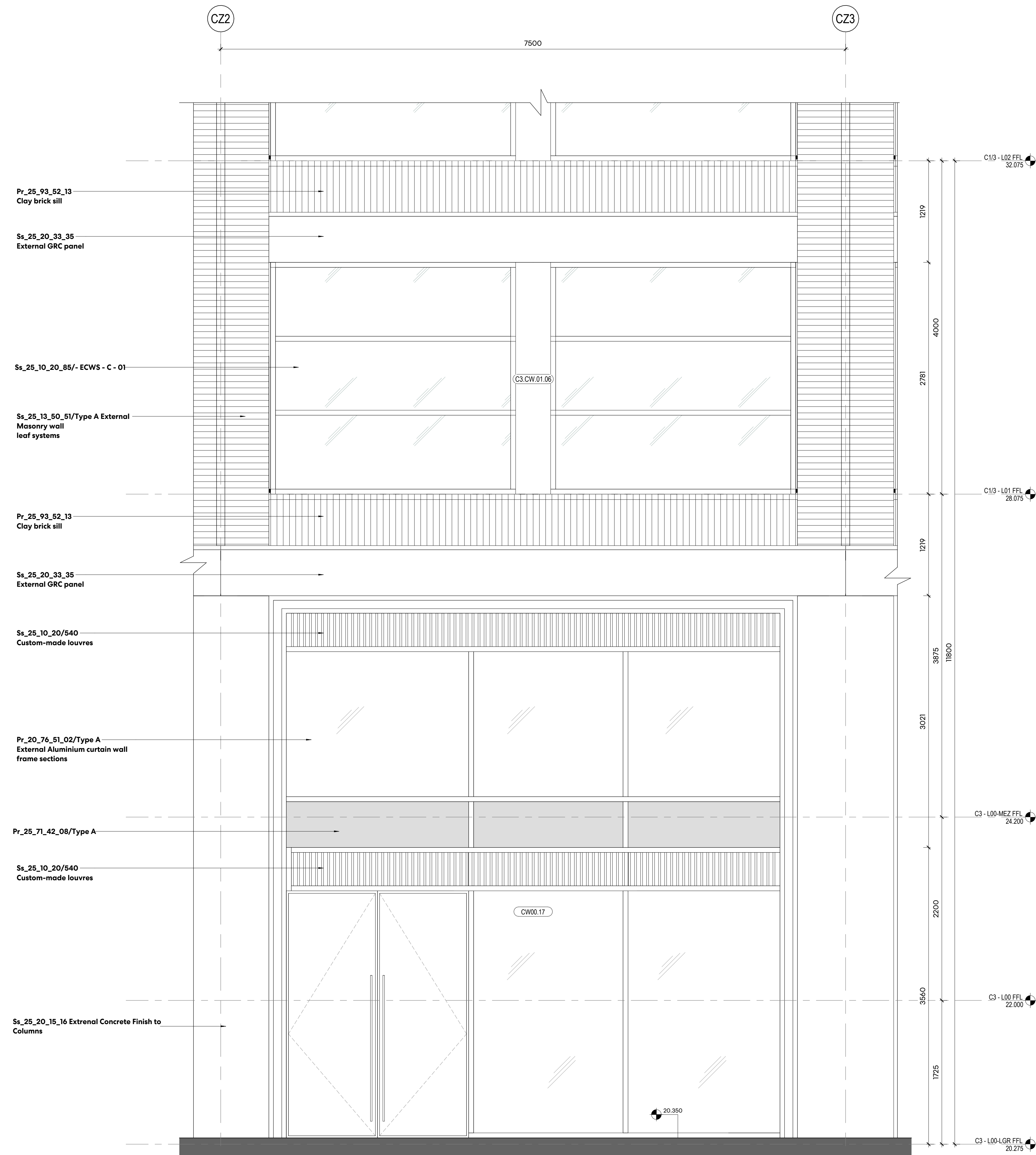
1 C3 - TYPICAL LOWER LEVEL WITH CONCRETE FIN - ENLARGED ELEVATION 1 : 25
