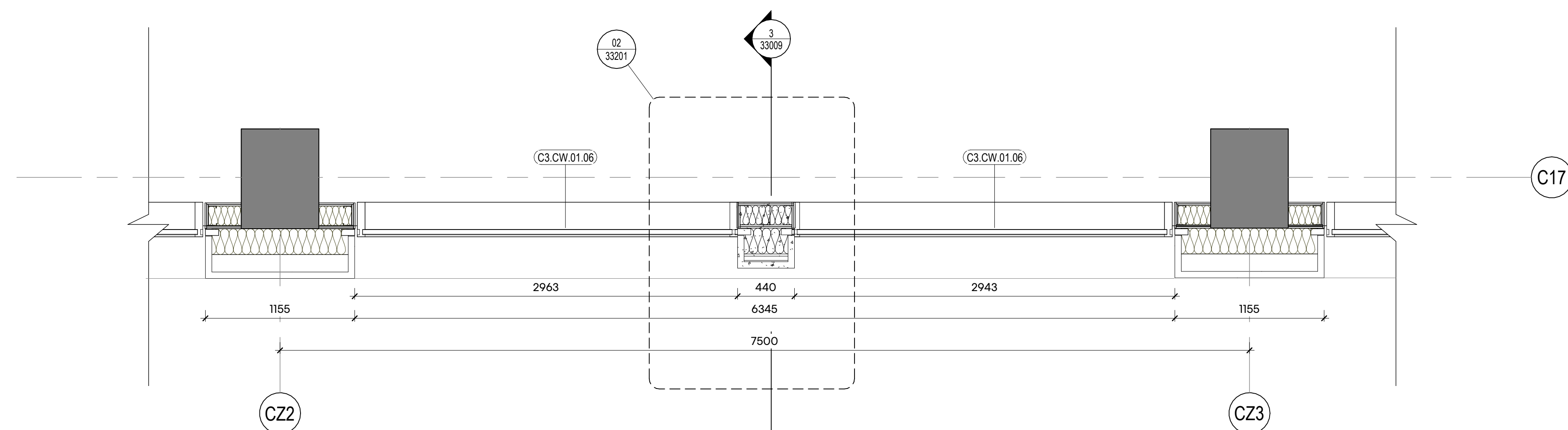
2 C3 - TYPICAL WINDOW BAY WITH CONCRETE FIN - LEVEL 01 - ENLARGED PLAN 1 : 25
