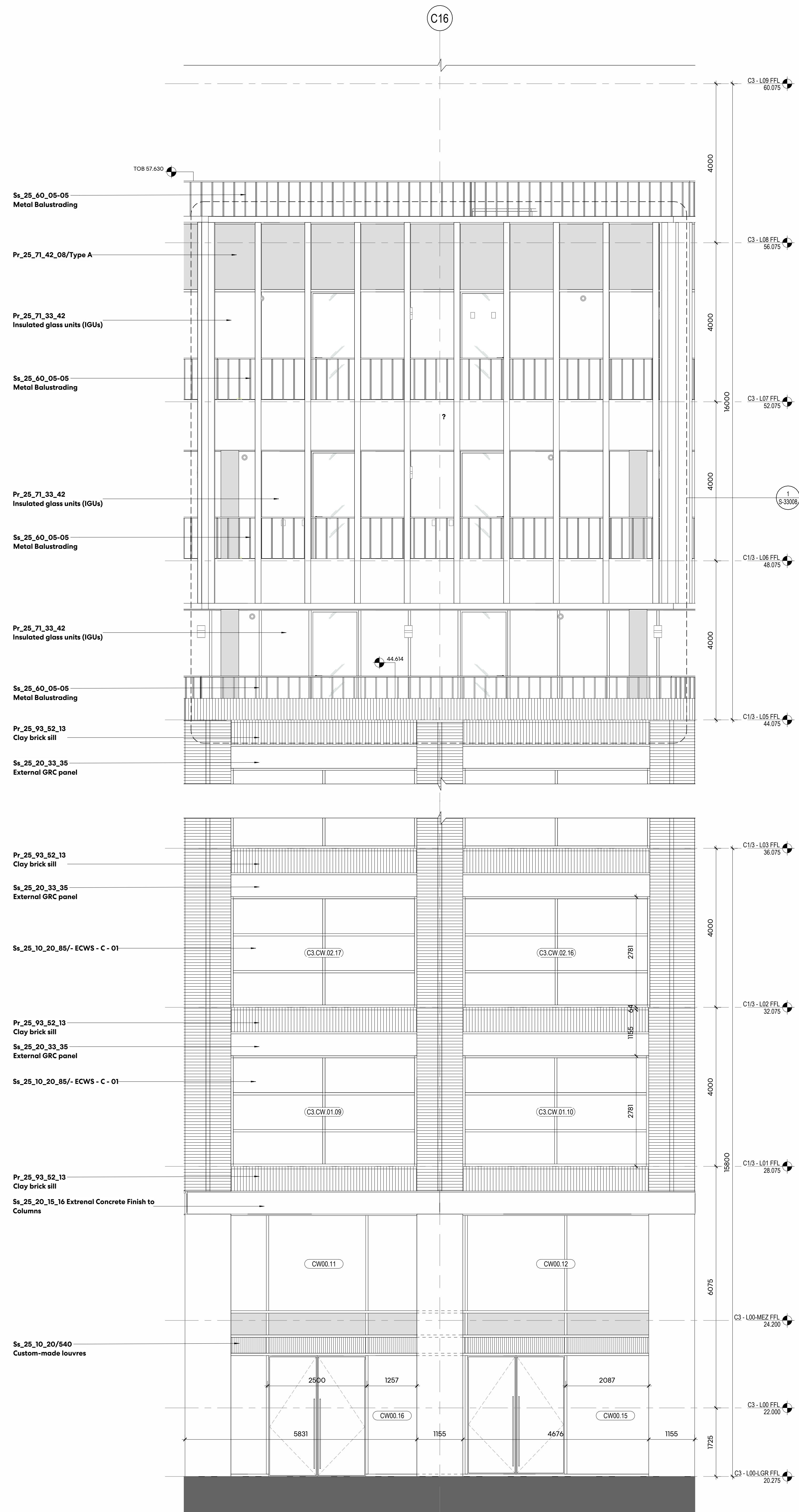
1 S3 C3 - ENLARGED SOUTH CORNER ELEVATION 1 : 50
