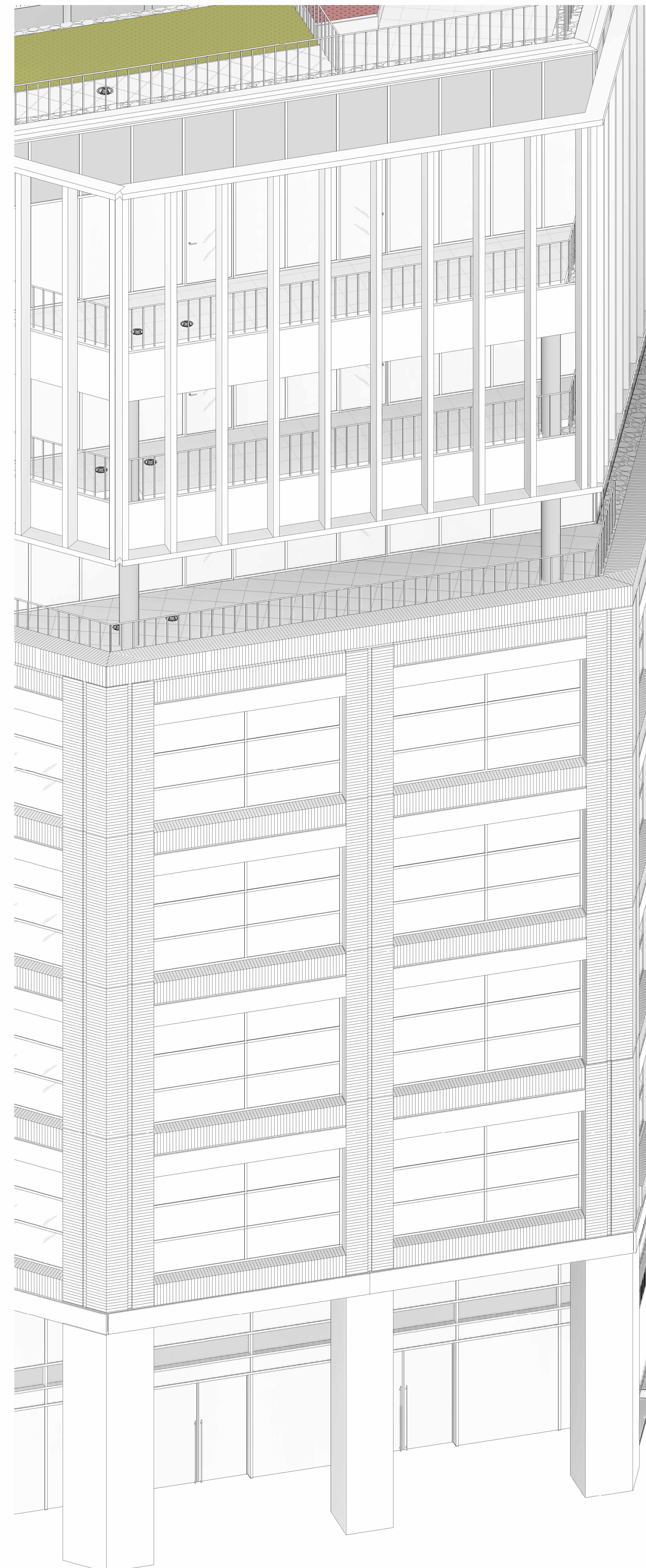
3 c3 - SOUTH CORNER AXONOMETRIC
