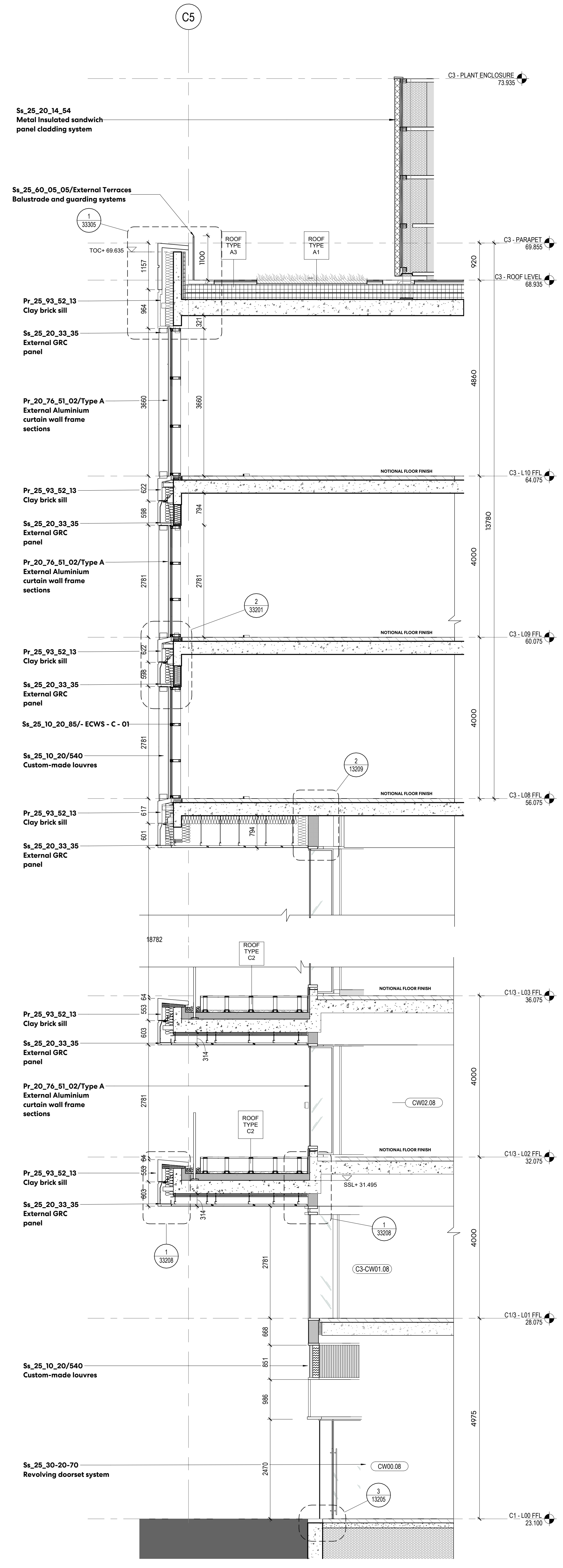
2 TYPICAL LOUVERED BAY SECTION THROUGH DOOR 1 : 50
