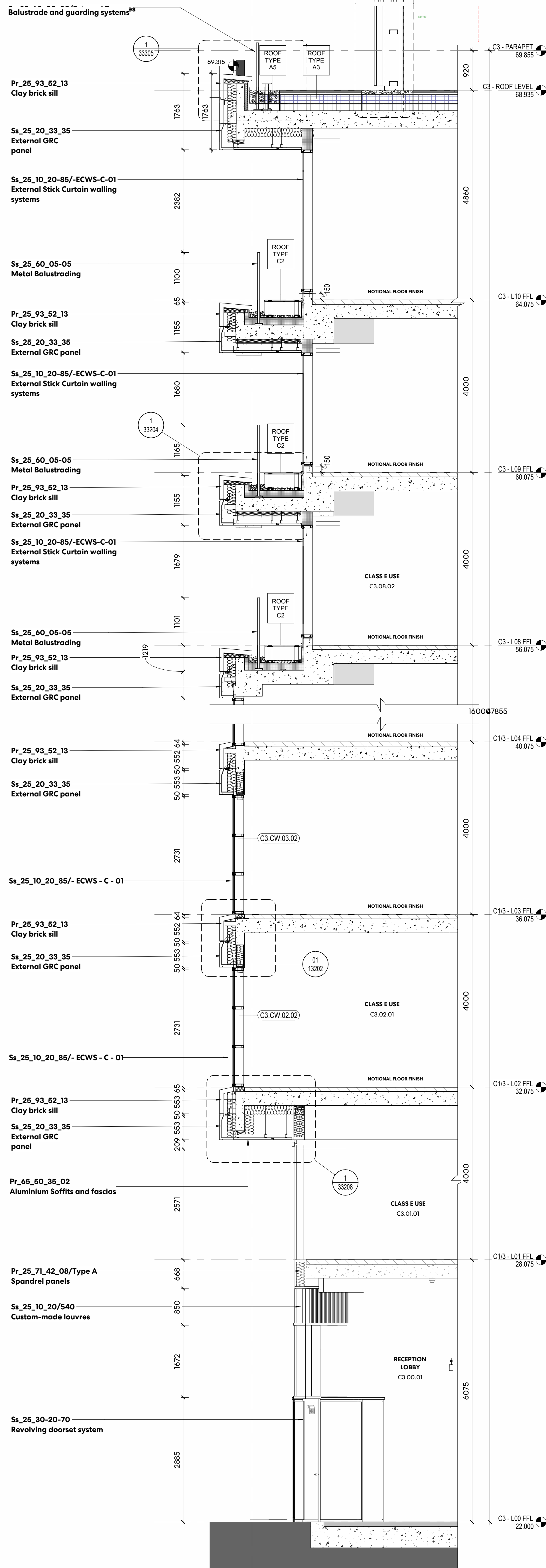
② C3 - NORTH EAST CORNER ENLARGED SECTION THROUGH REVOLVING DOOR 1:50
