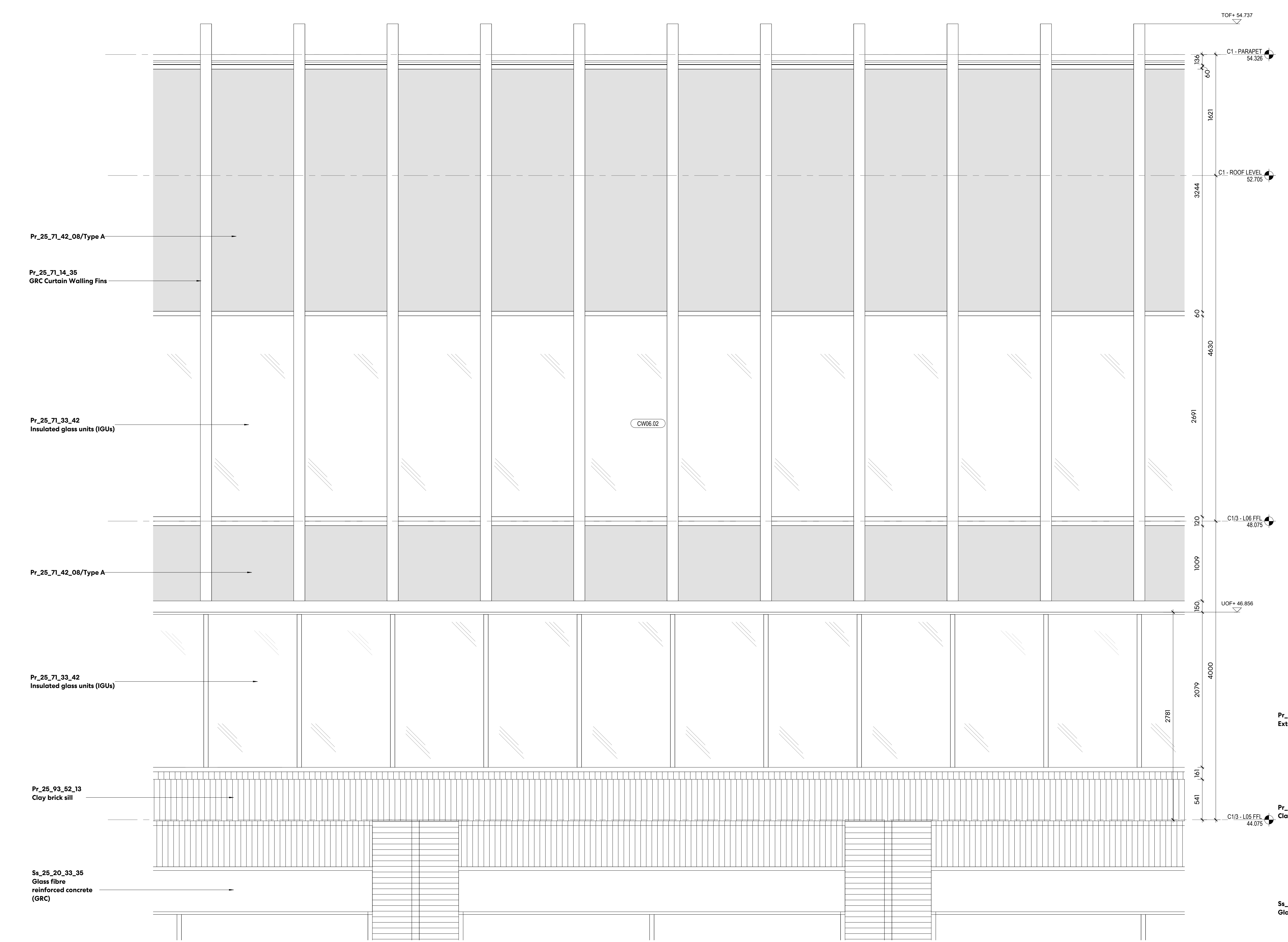
③ TYPICAL MID LEVEL FACADE LEVEL - ELEVATION 1:25
