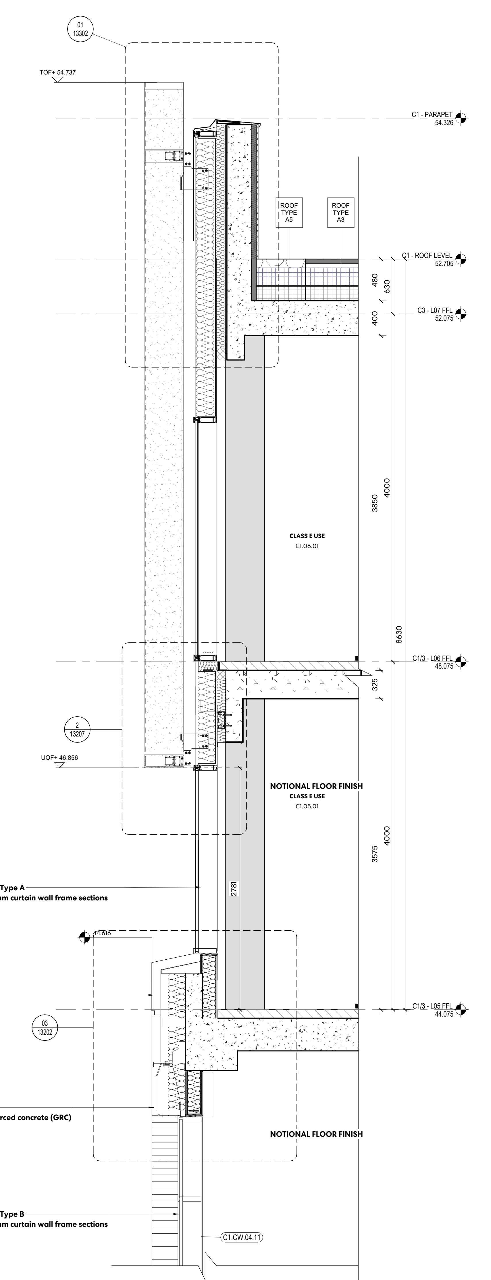
④ TYPICAL MID LEVEL FACADE LEVEL 05-07 DETAIL SECTION 1:25
