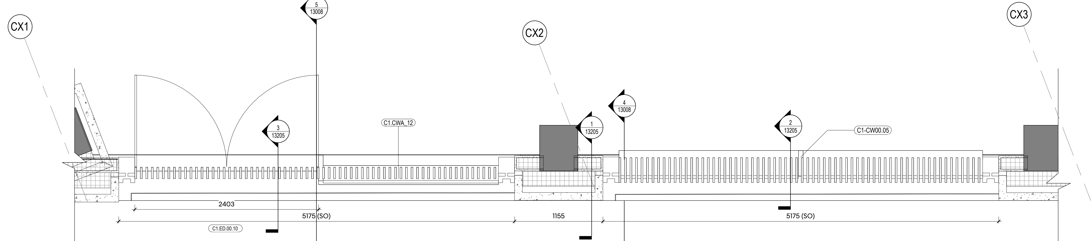
2 TYPICAL LOWER LEVEL FACADE LEVEL 01 DETAIL PLAN 1:25
