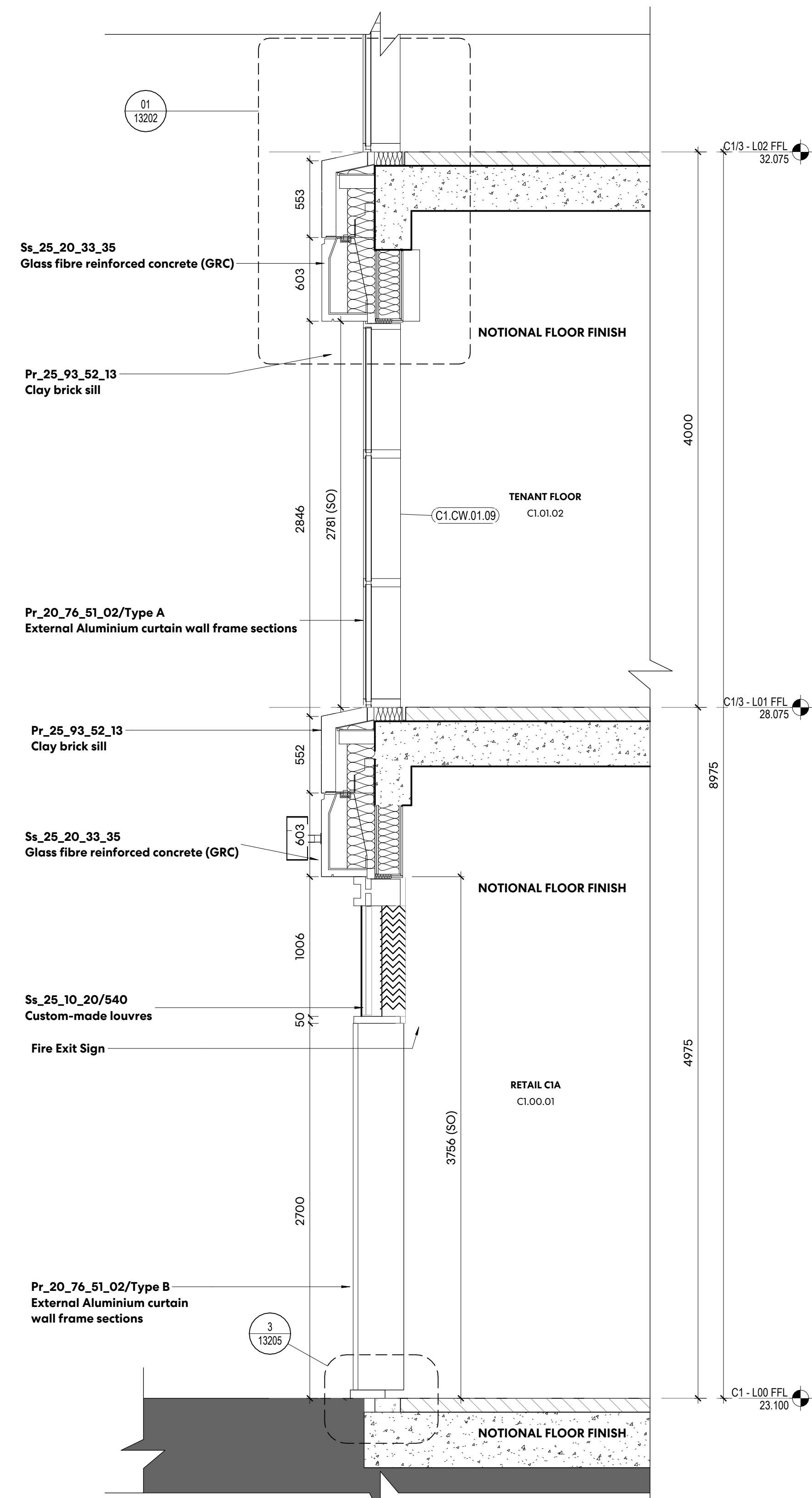
4 TYPICAL LOWER LEVEL FACADE LEVEL 00-02 DETAIL SECTION 1:25
