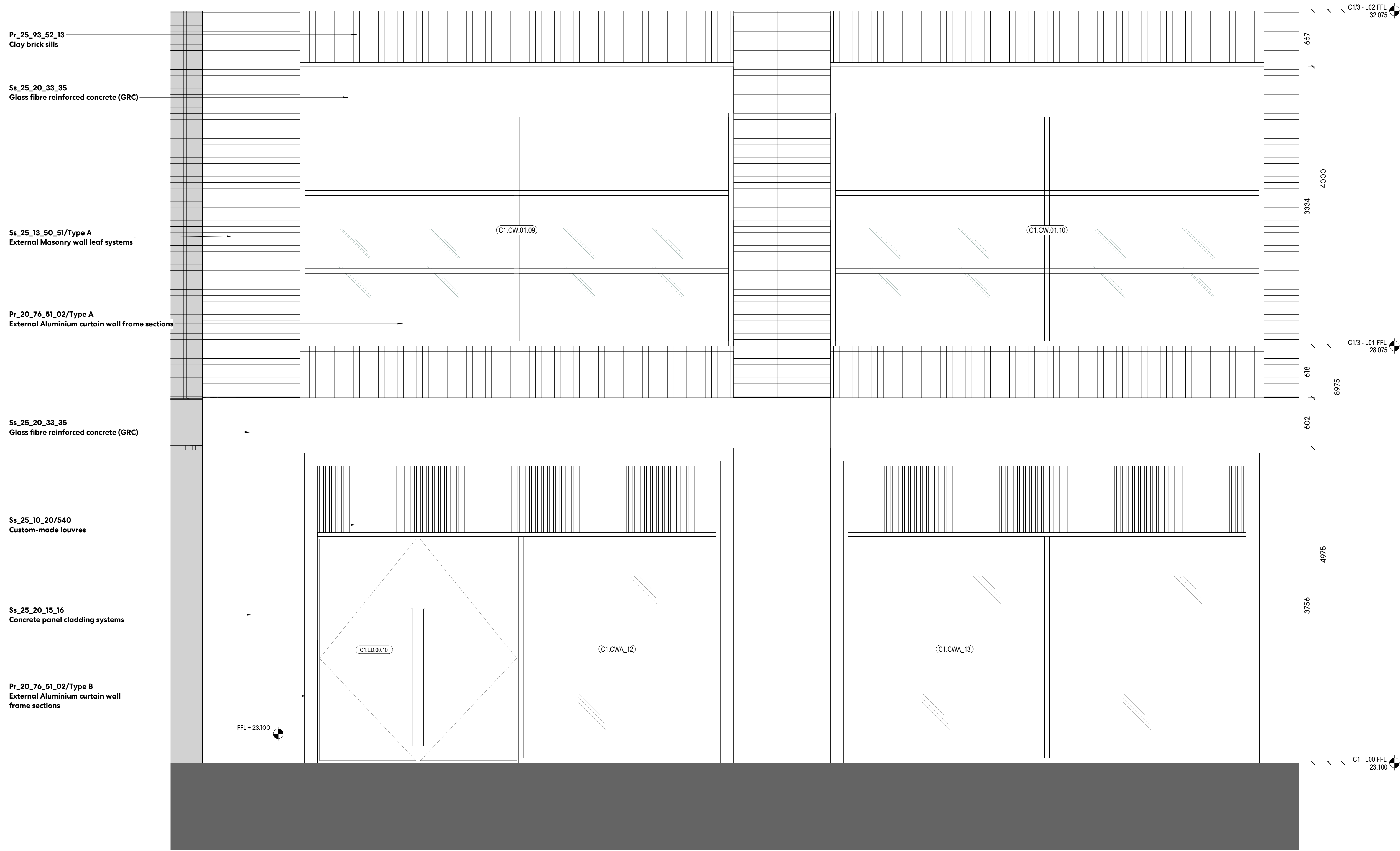
3 TYPICAL LOWER LEVEL FACADE LEVEL 01 - ELEVATION 1:25
