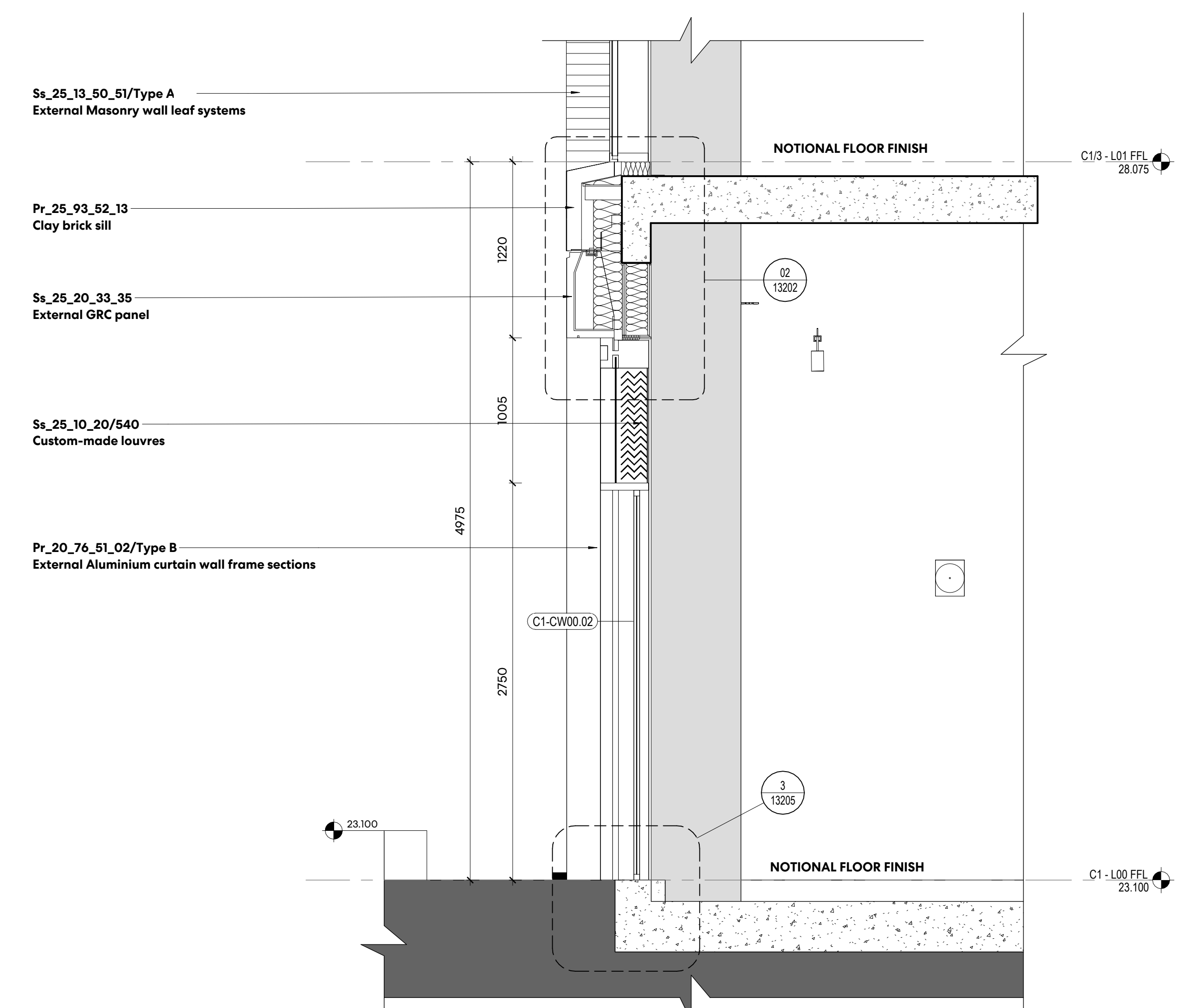
4 WEST RETAIL ENTRANCE GLAZING LEVEL 00-02 DETAIL SECTION 1:25
