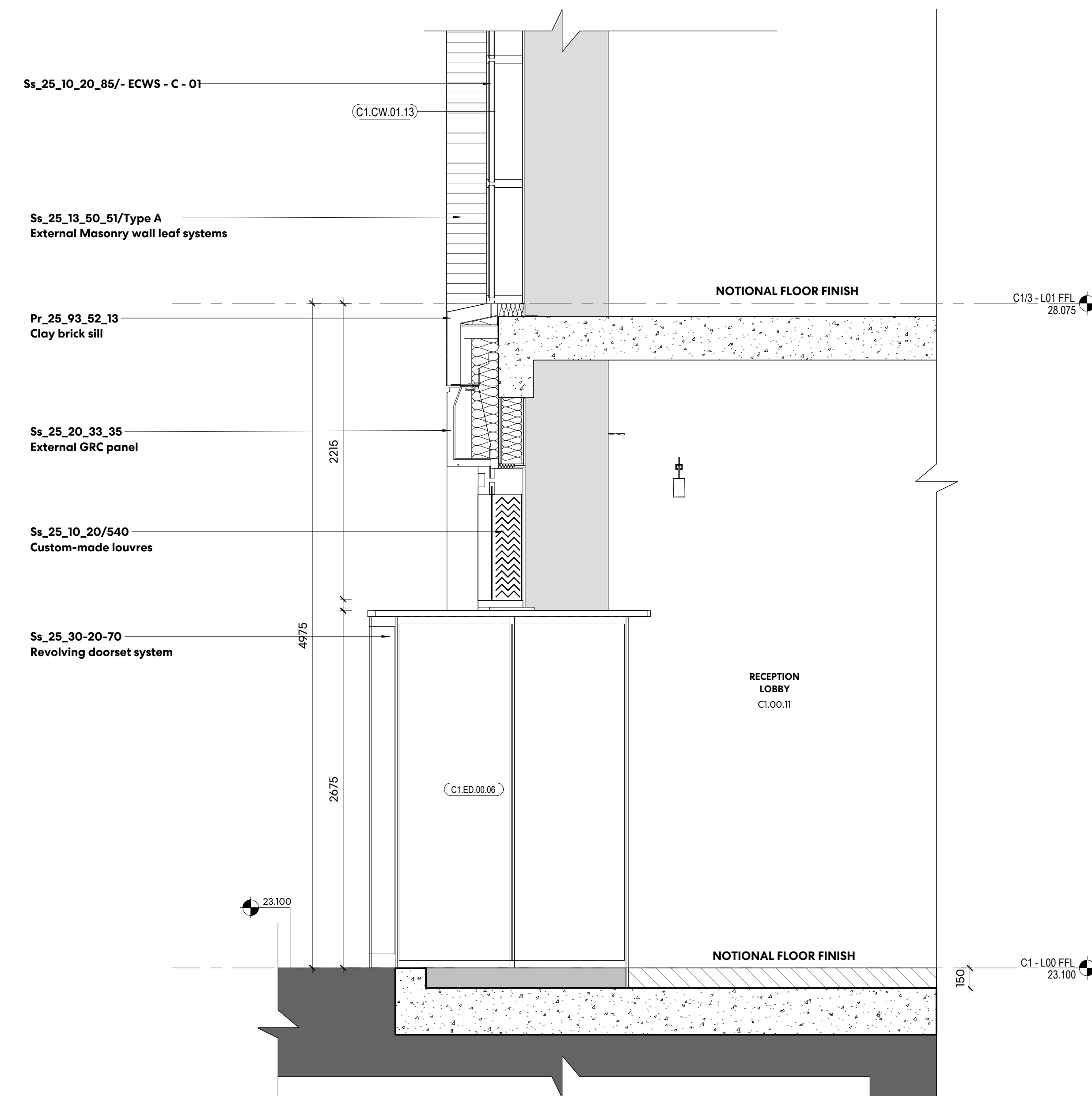
3 WEST RETAIL ENTRANCE REVOLVING DOOR LEVEL 00-01 DETAIL SECTION 1:25
