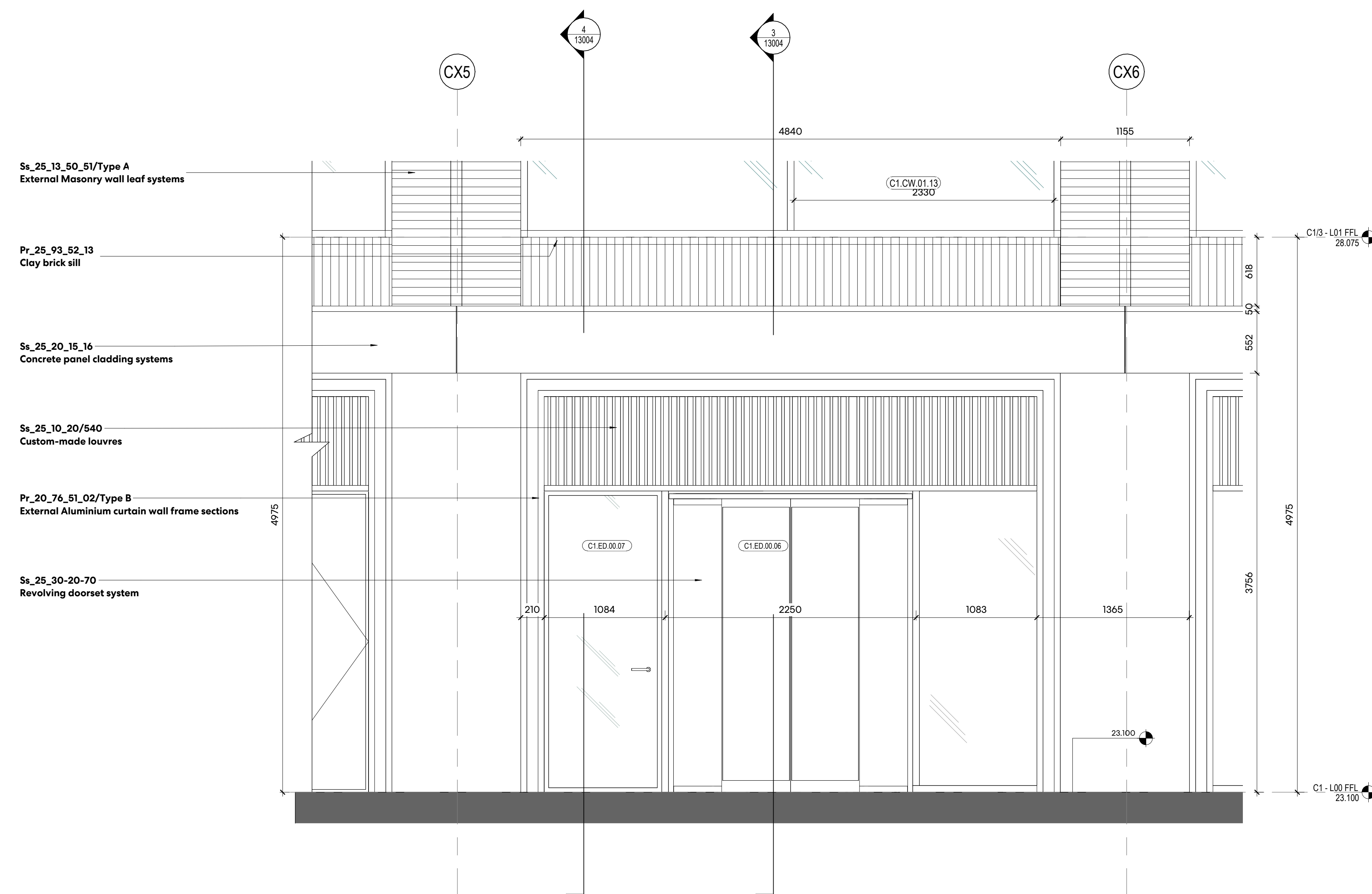
2 WEST RETAIL ENTRANCE FACADE DETAIL ELEVATION 1:25
