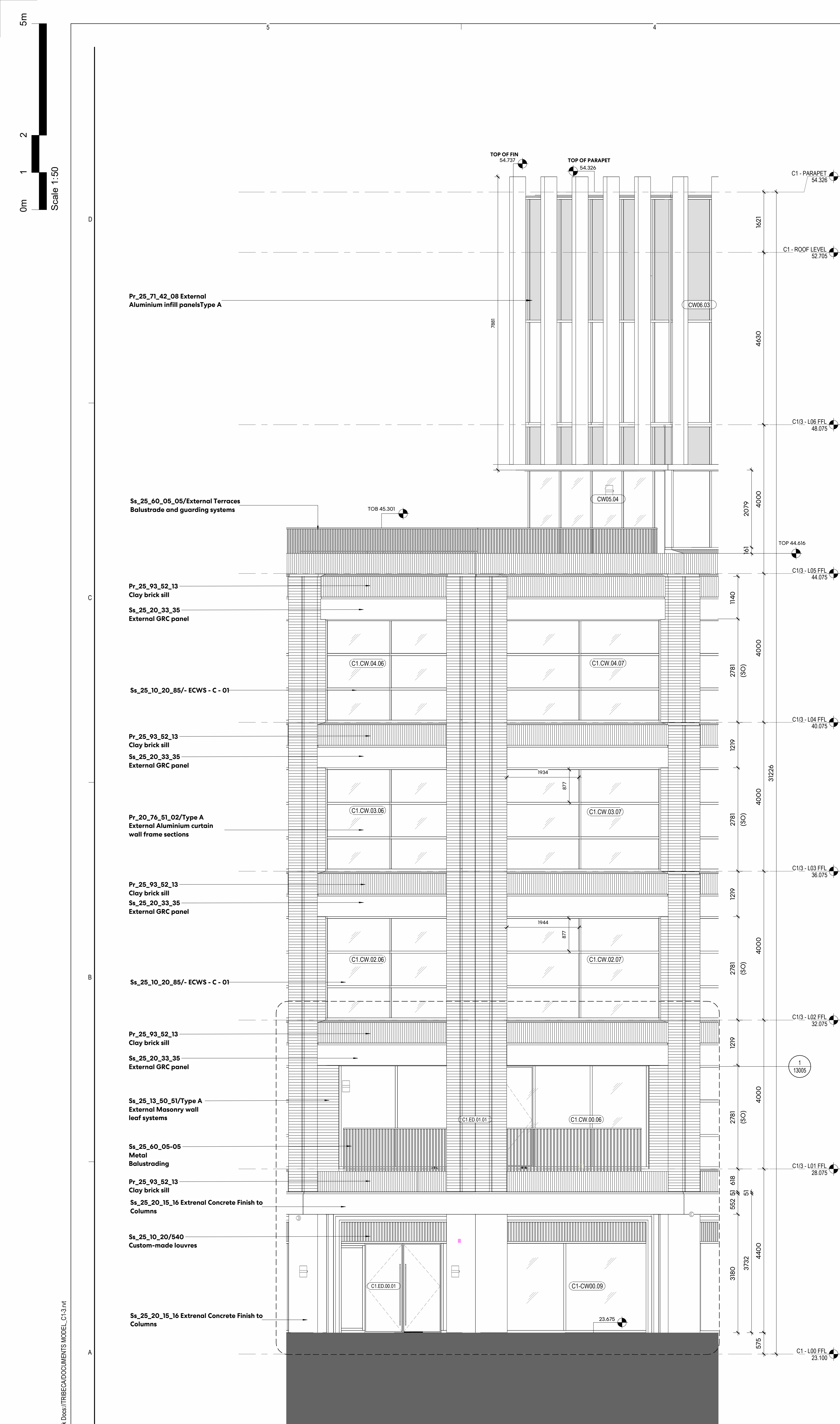
1 NORTH EAST CORNER FACADE ENLARGED ELEVATION 1 : 50
