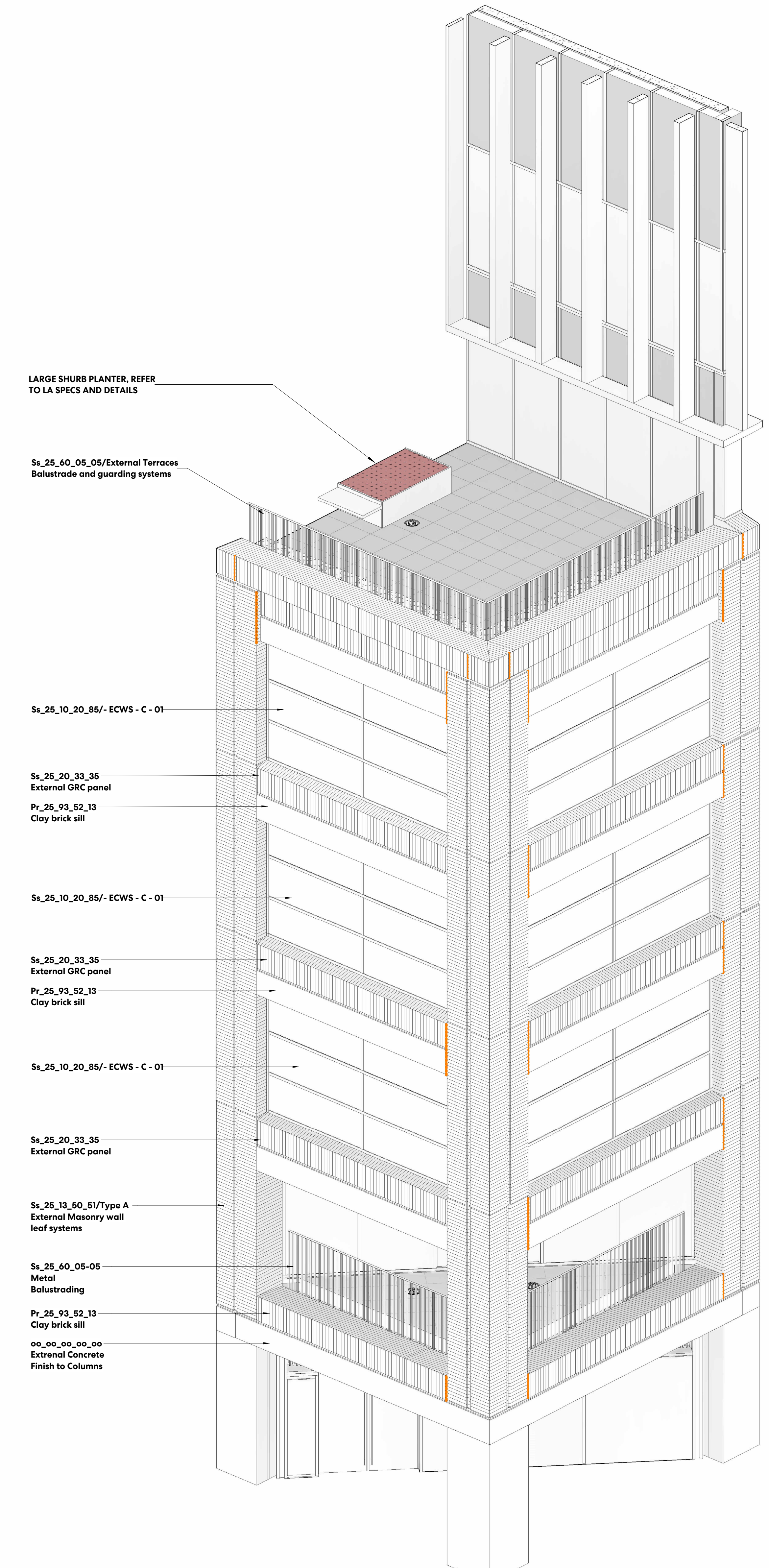
3 NORTH EAST CORNER ENLARGED AXONOMETRIC
