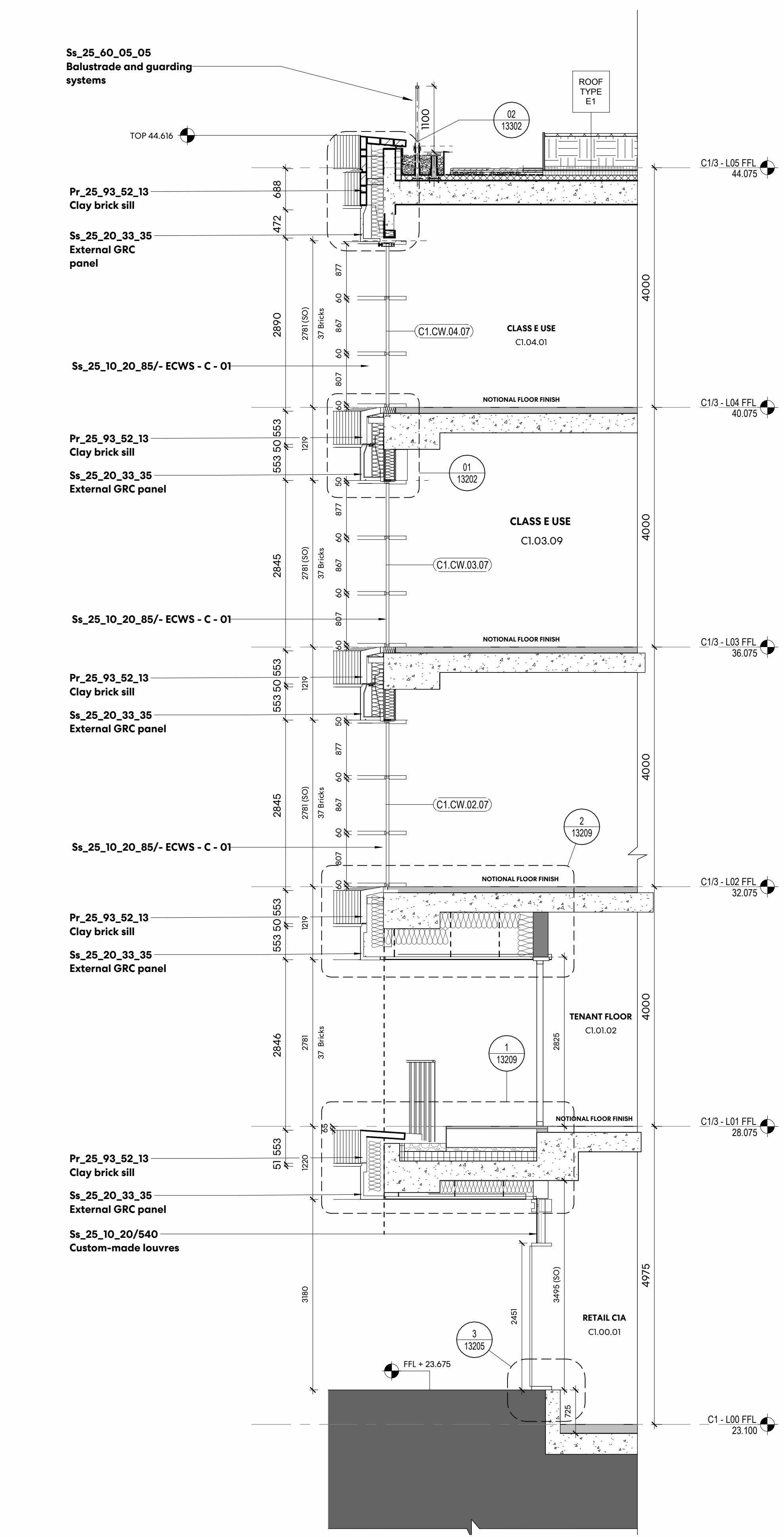
2 NORTH EAST CORNER FACADE ENLARGED SECTION THROUGH DOOR 1 : 50
