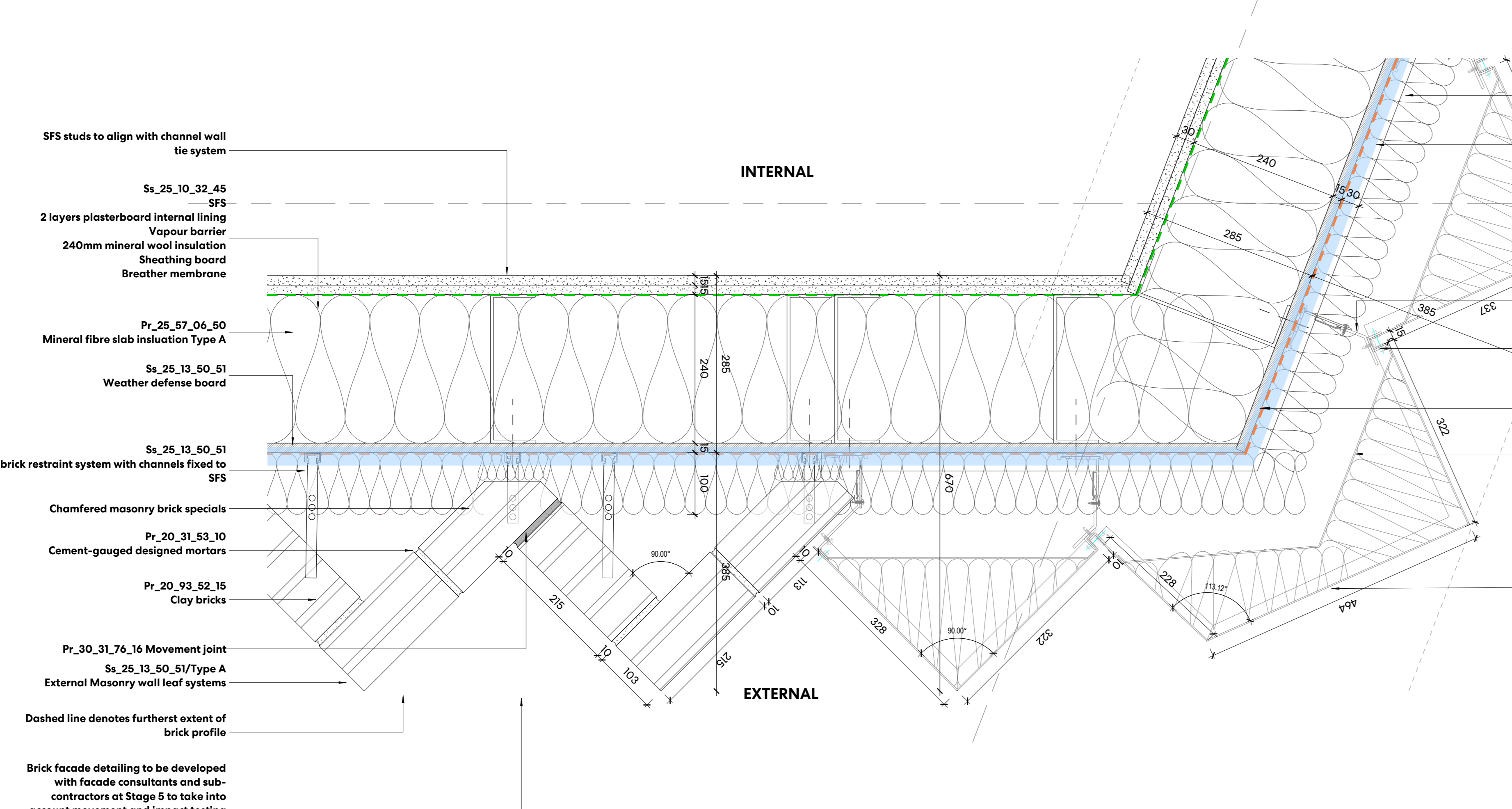
2 C4 - BRICK + CORTEN JUNCTION 1:5
