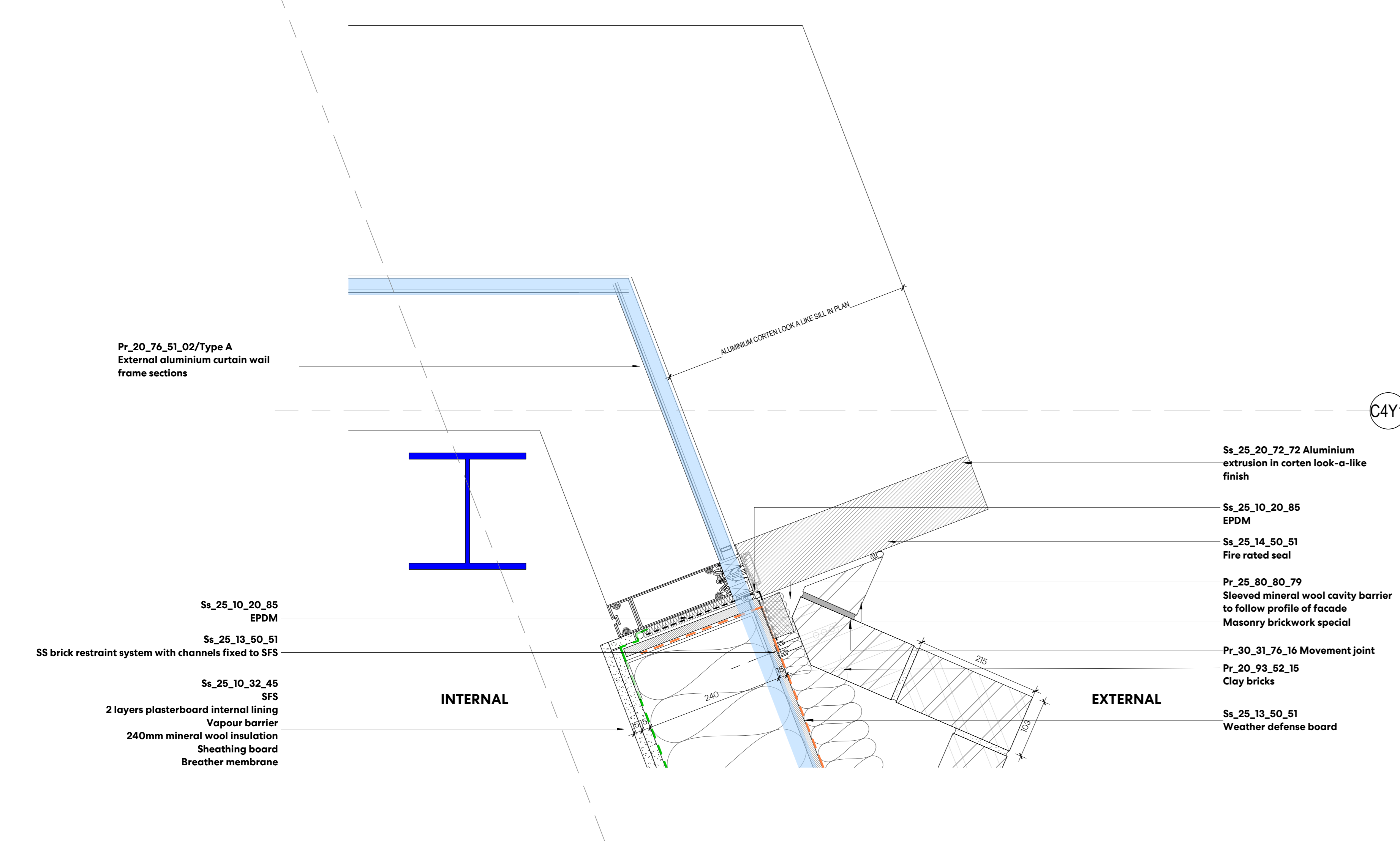
1 C4 - TYPICAL BRICK + CURTAIN WALL DETAIL PLAN DETAIL 1:5
