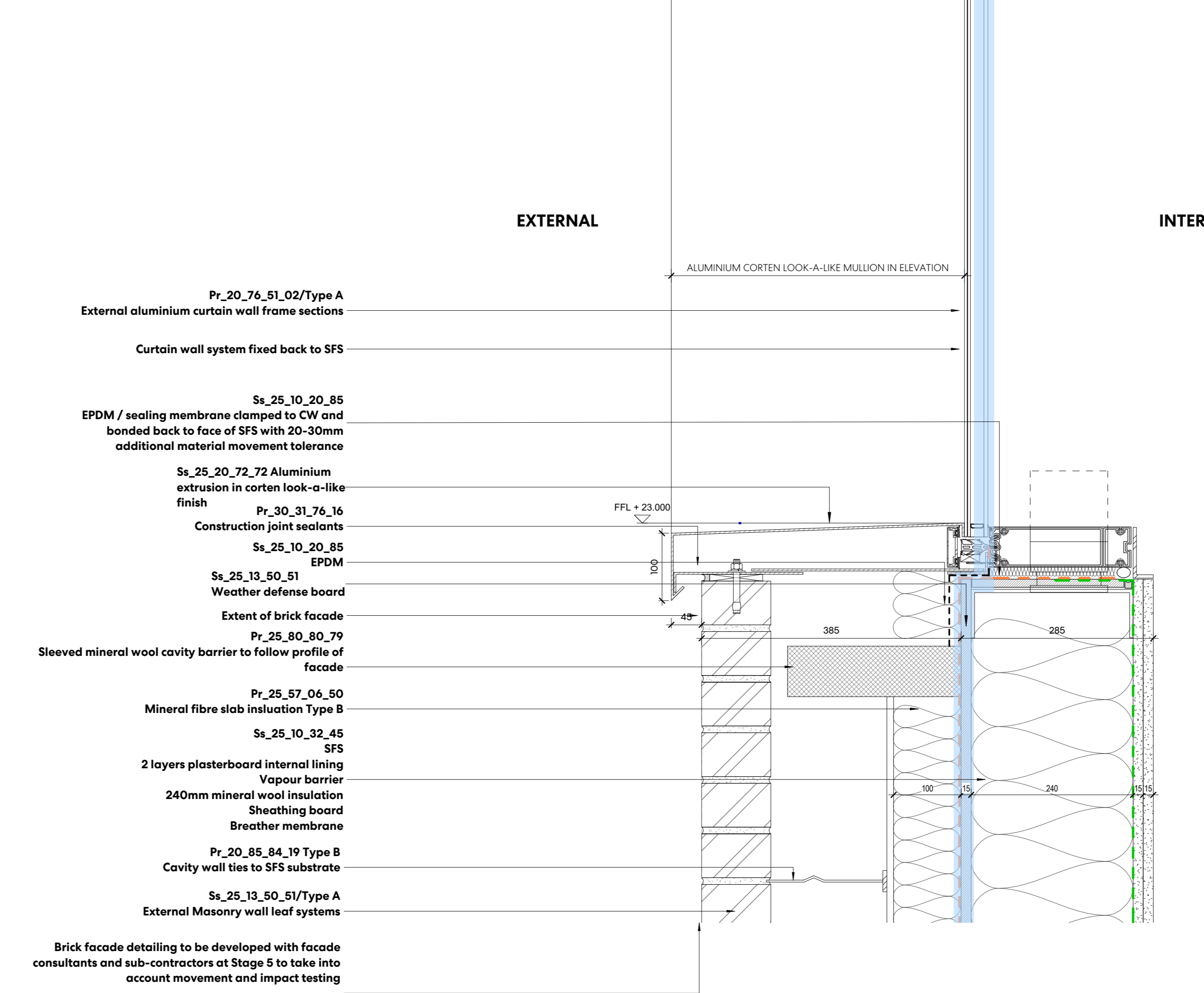
3 C4 - TYPICAL BRICK + CURTAIN WALL DETAIL SECTION 1:5
