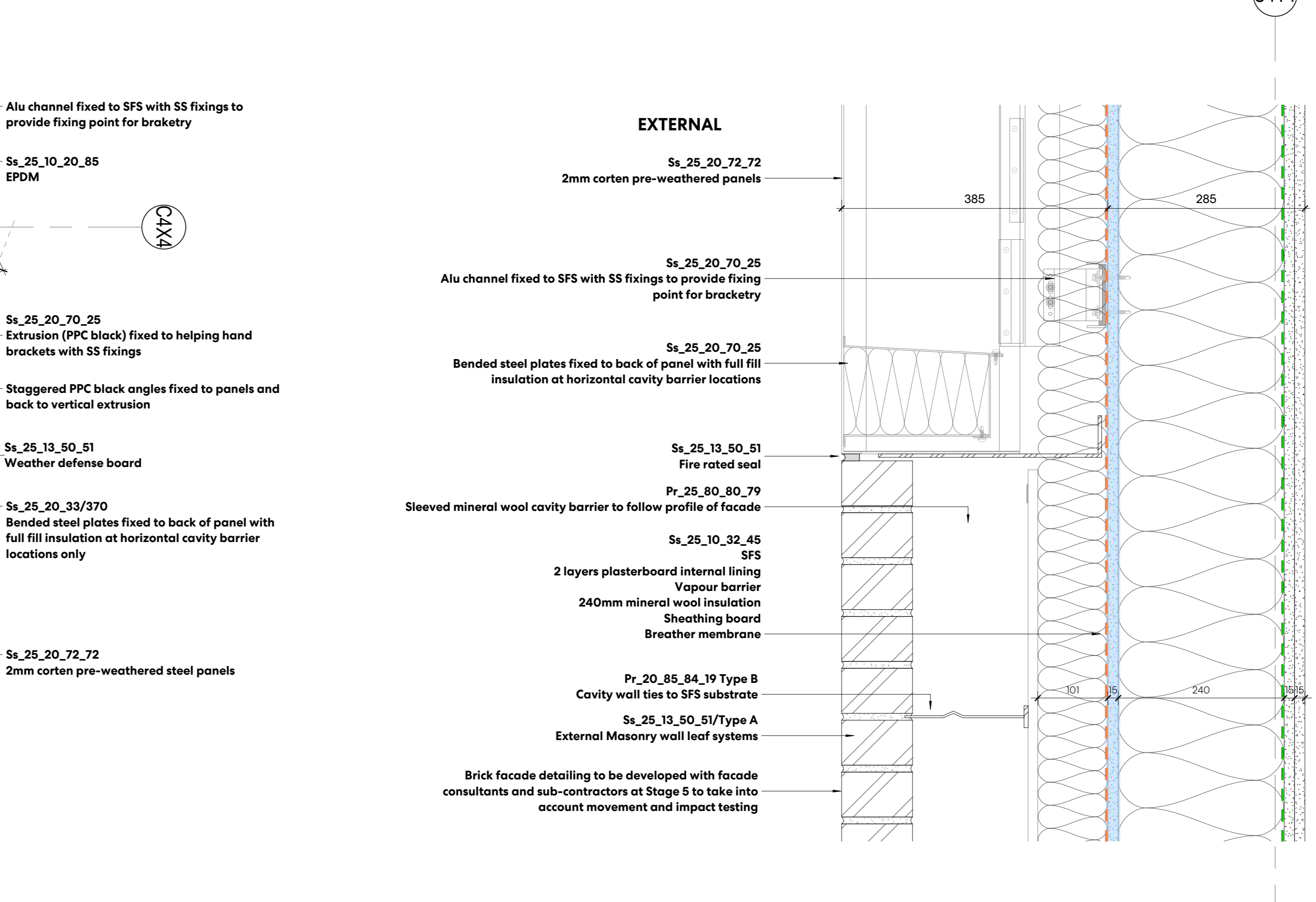
4 C4 - TYPICAL CORTEN + BRICK SECTION 1:5
