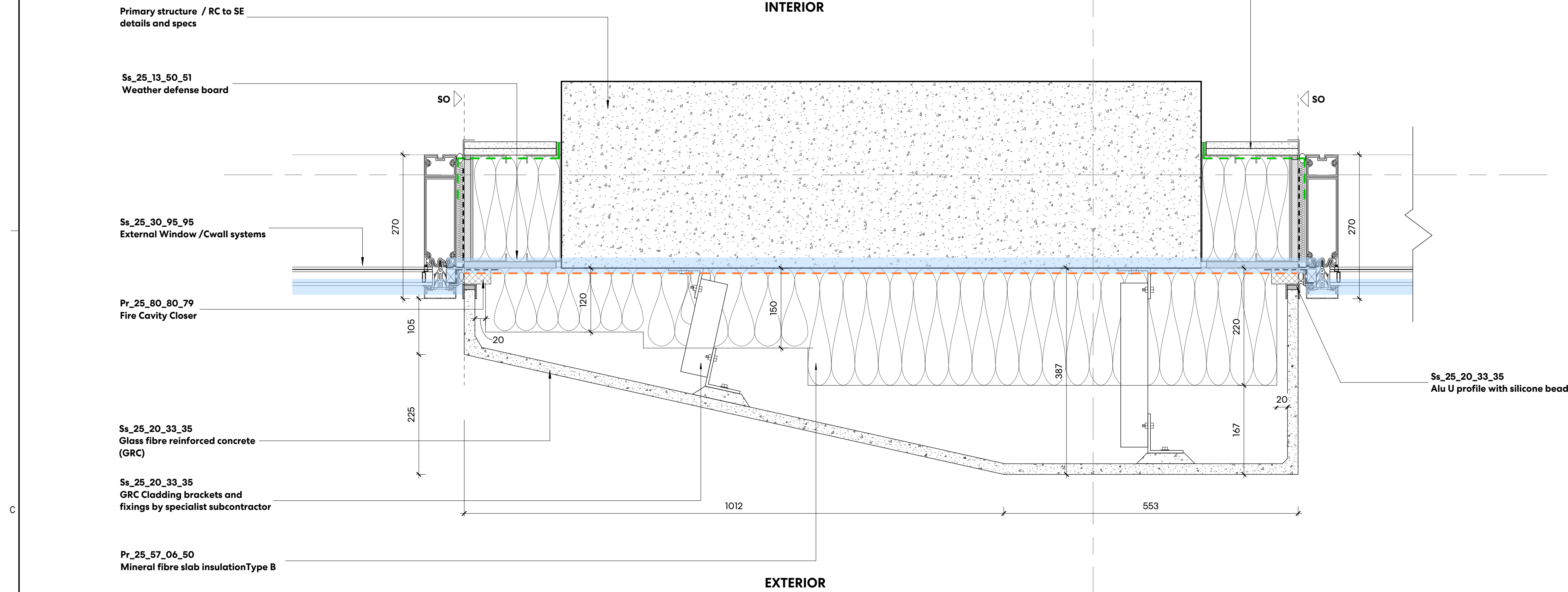
1 TYP GROUND FLOOR LEVEL PIER IN GRC 1:5
