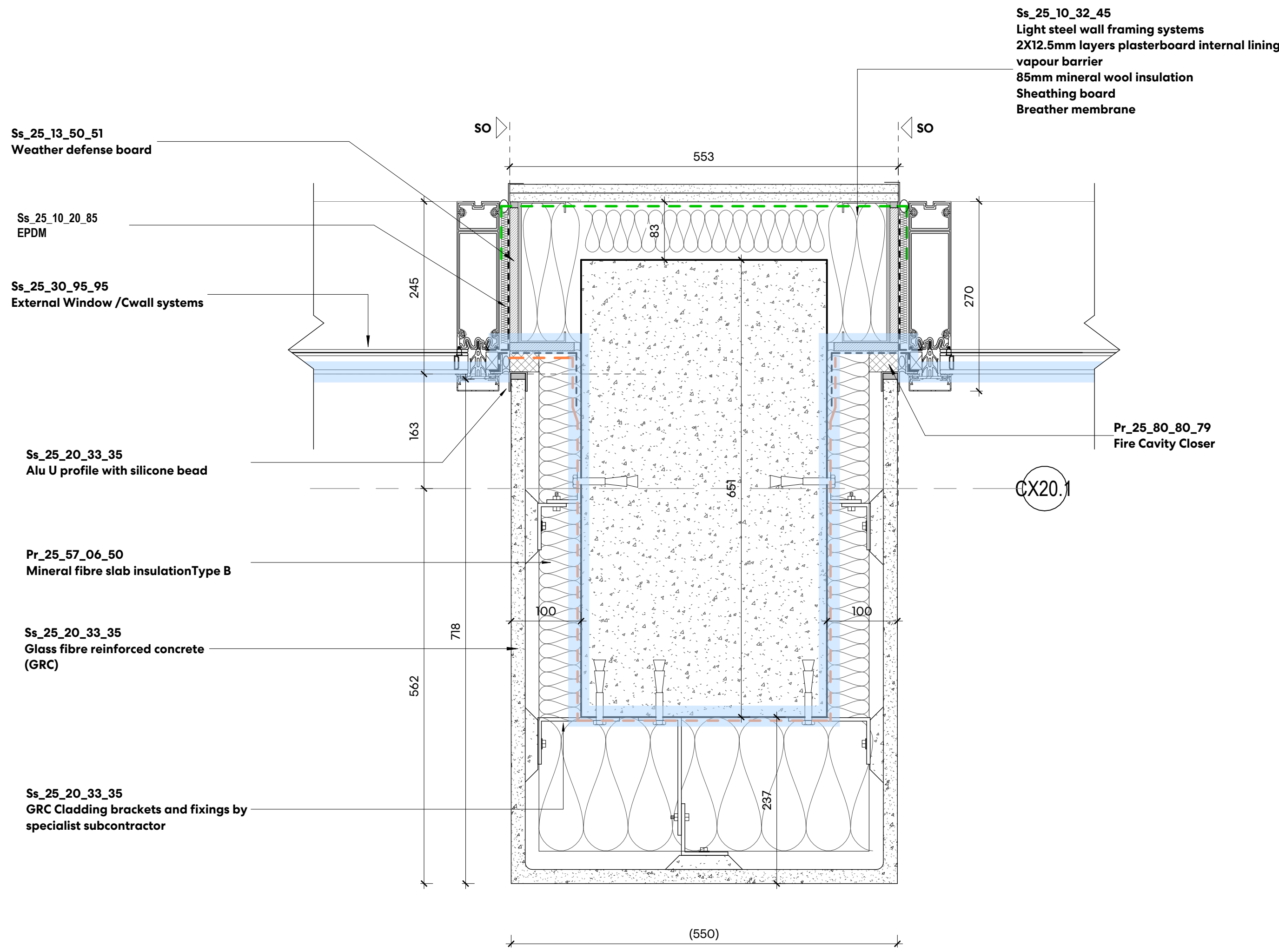
2 TYP GFL(SOUTH) PIER IN GRC 1:5
