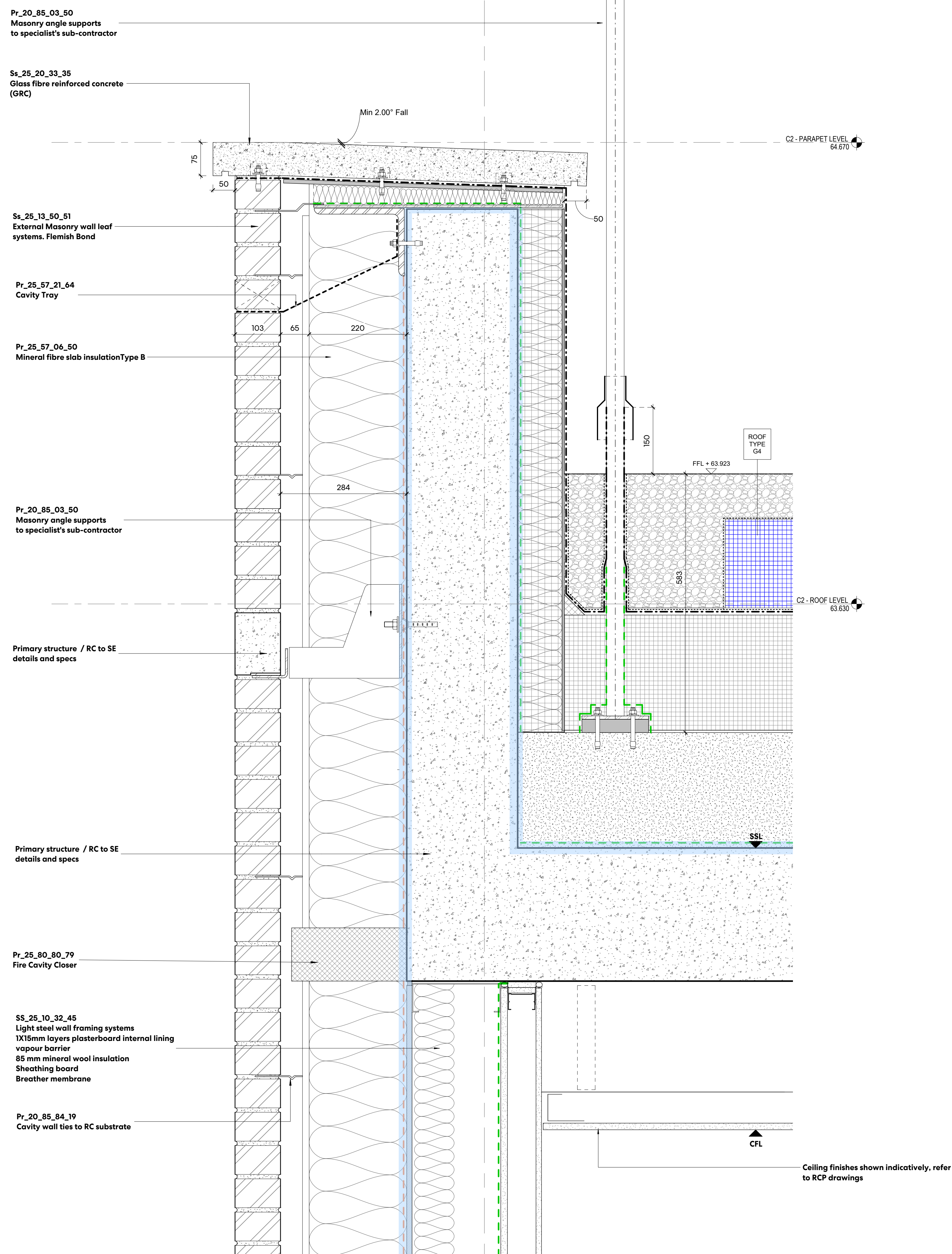
③ TYPICAL PARAPET EDGE DETAIL / BRICK 1:5
