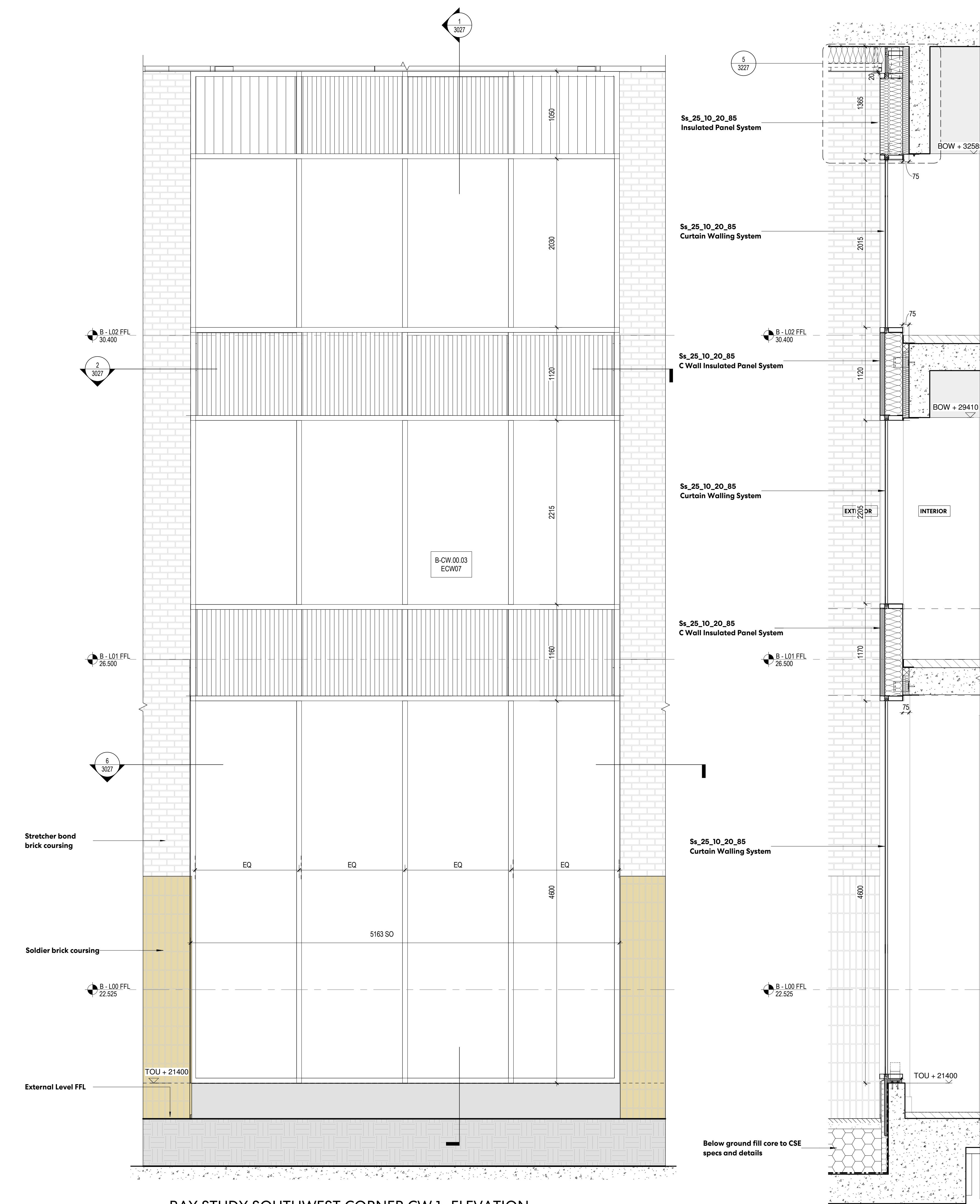
⑤ BAY STUDY SOUTHWEST CORNER CW 1- ELEVATION 1 : 25
