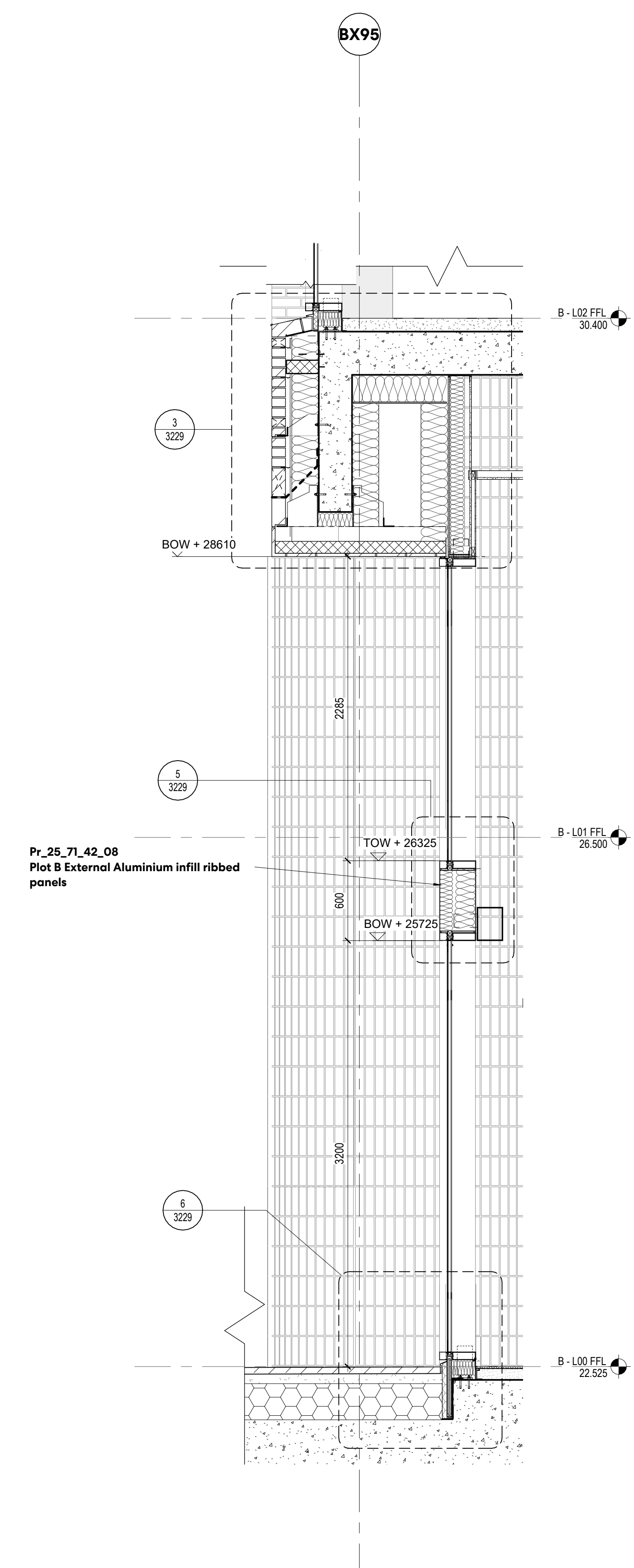
2 SOUTH MAIN ENTRANCE LEVEL 00-02 DETAIL SECTION - 2 1:25
