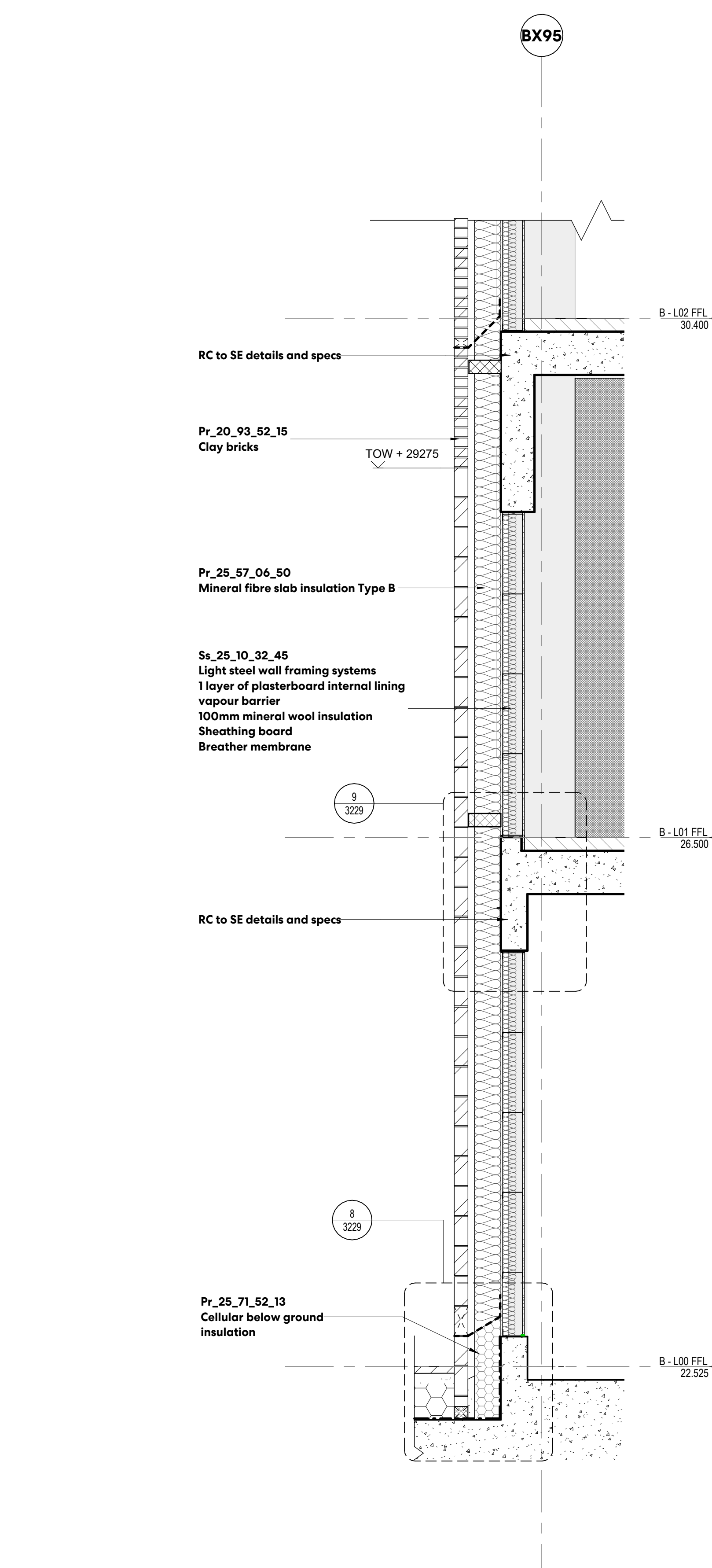
3 SOUTH MAIN ENTRANCE LEVEL 00-02 DETAIL SECTION - 3 1:25
