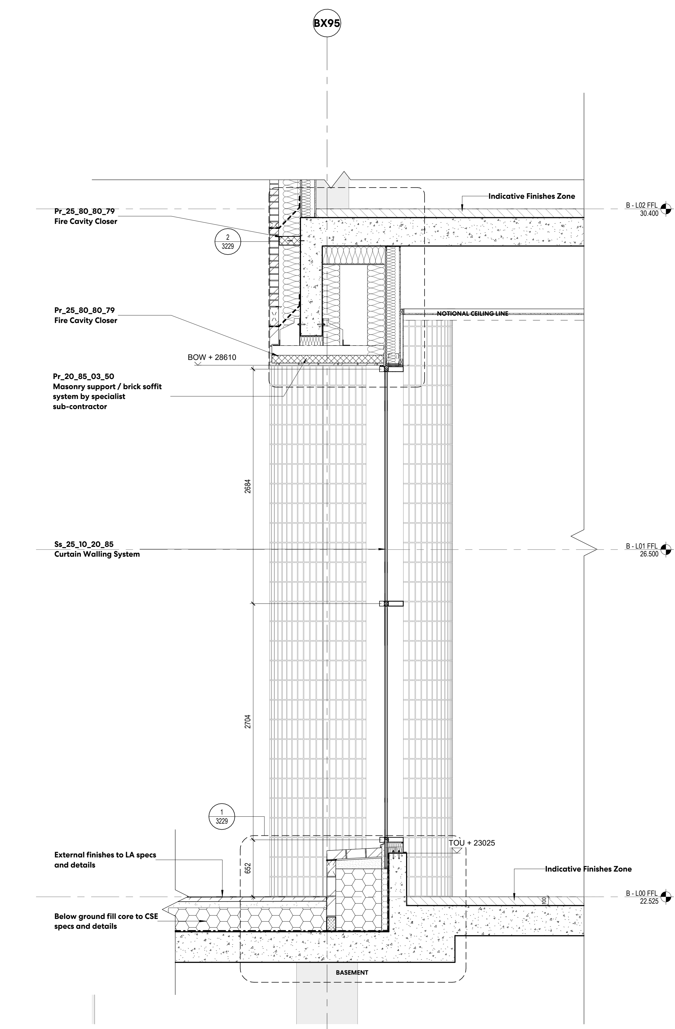
1 SOUTH MAIN ENTRANCE GLAZING LEVEL 00-02 DETAIL SECTION 1:25
