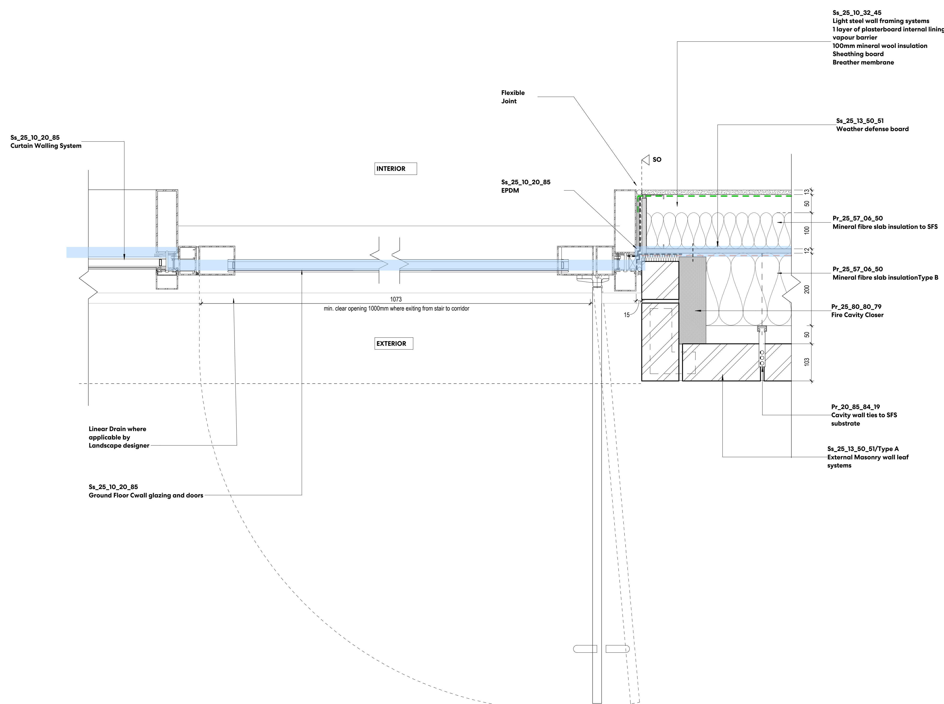
1 TYP CURTAIN WALL DOOR AT GF LEVEL - PLAN DETAIL 1:5
