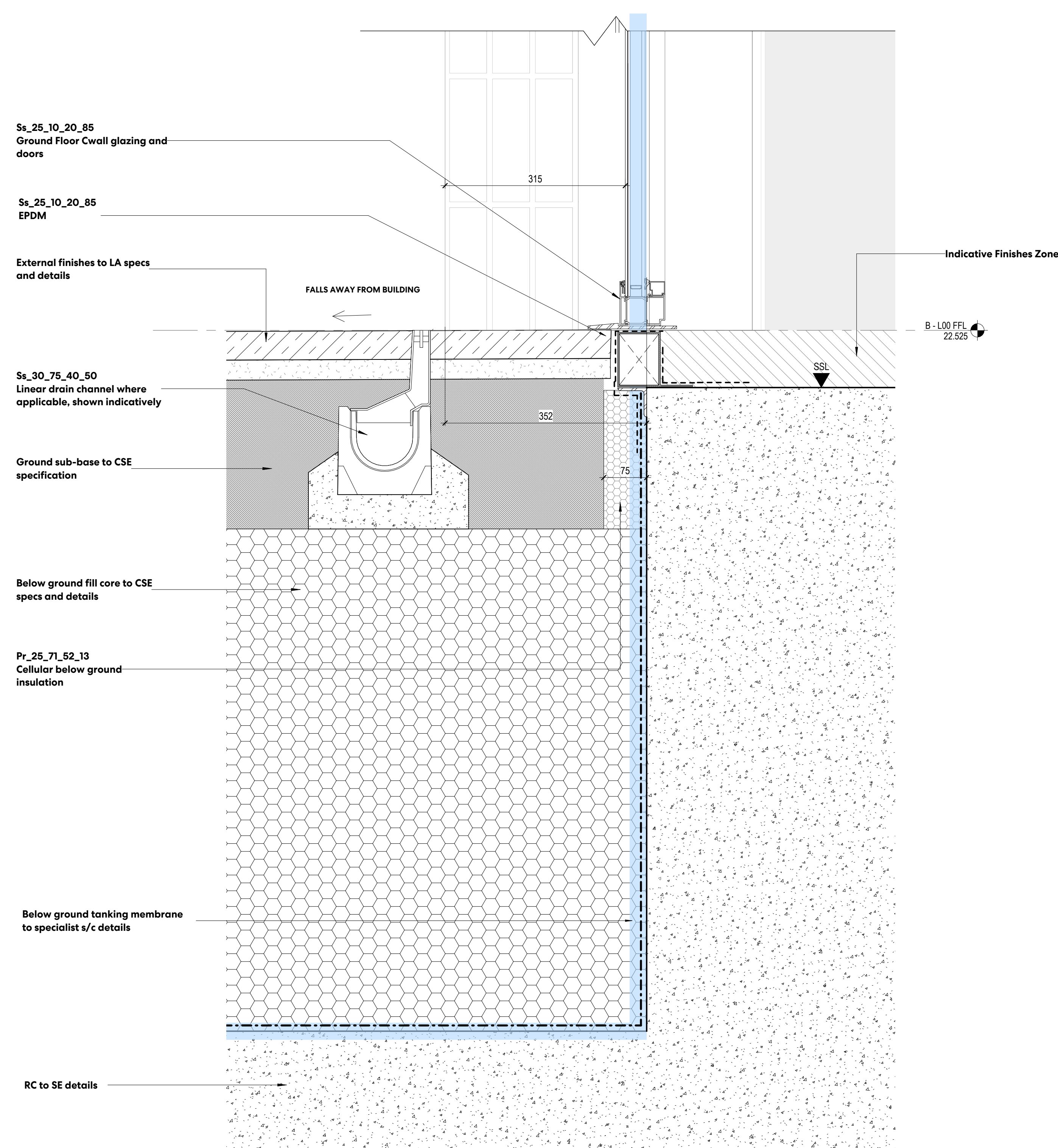
2 CURTAIN WALL DOOR GF LEVEL - HEAD AND FOOT DETAIL 1:5
