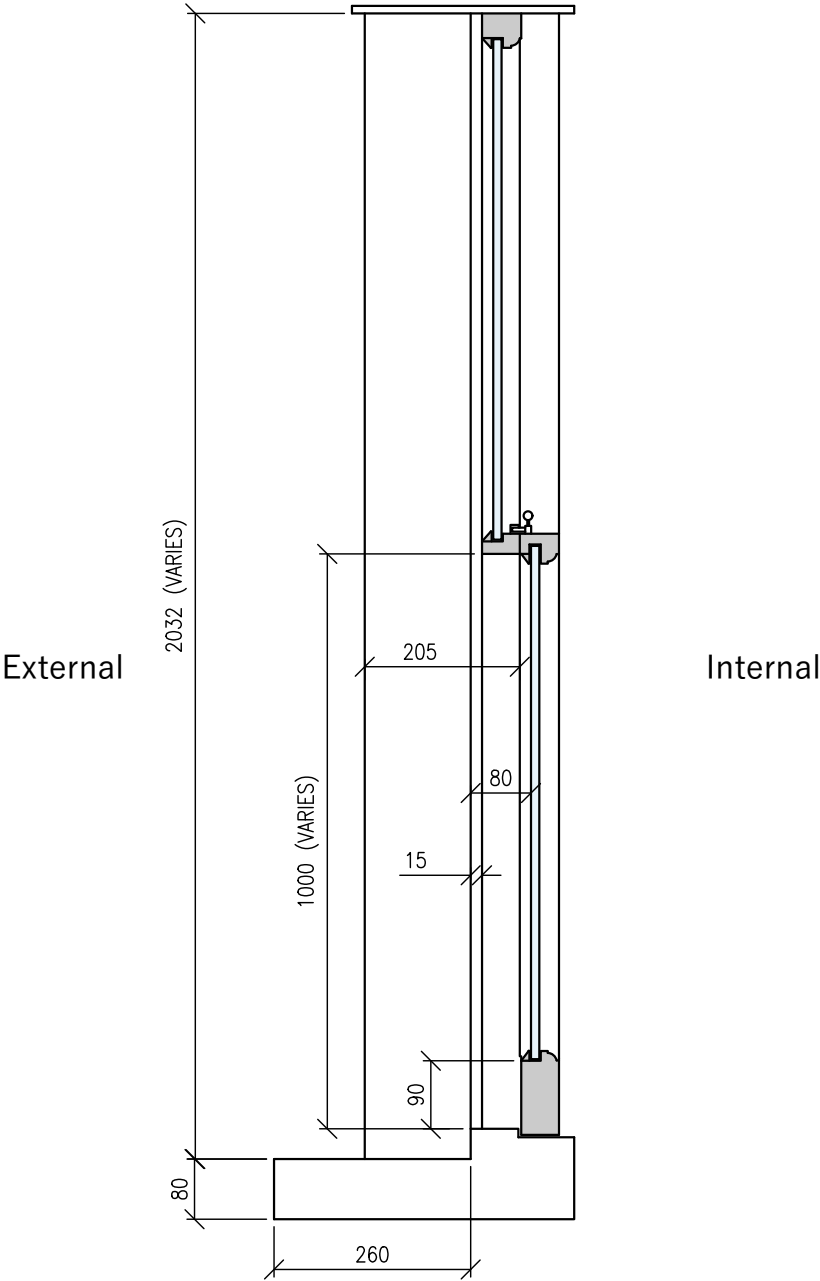
Typical Cross Section of Existing Sash Window
