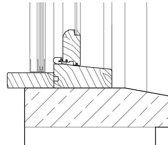
05 Section detail C (51)005 1:5@A3
