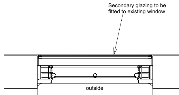
02 Plan C (51)005 1:20@A3
