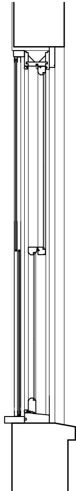
03 Section C (51)005 1:20@A3
