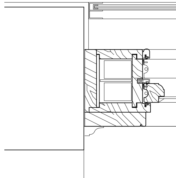
04 Jamb detail C (51)005 1:5@A3
