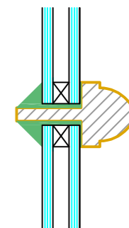
Glazing bar cross section @ 1:2
