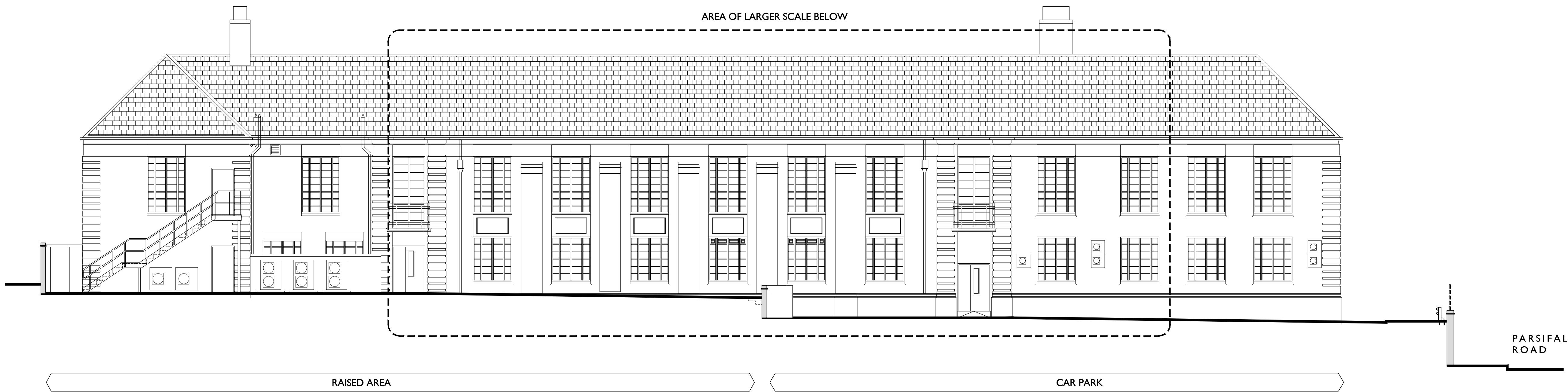
EXISTING ELEVATION B - FROM CAR PARK ( refer to drawing 711 for elevation location ) Scale 1:100
