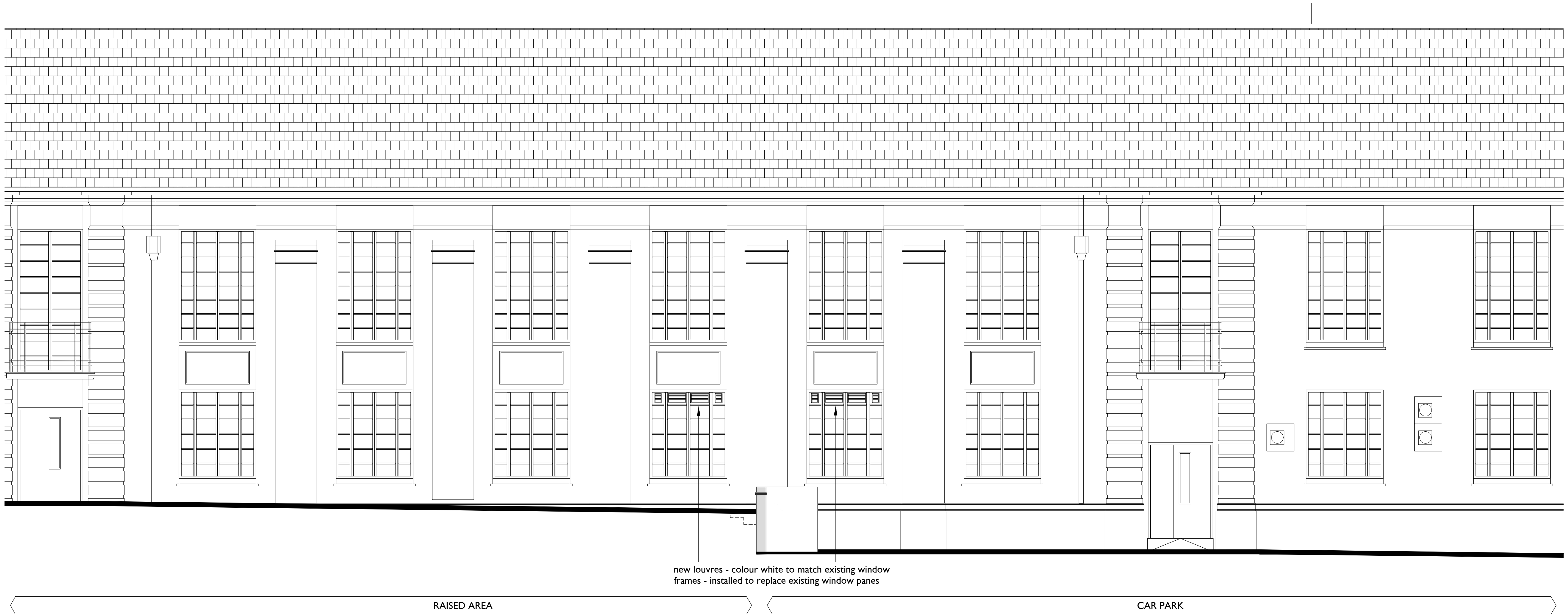
EXISTING LARGER SCALE ELEVATION B - FROM CAR PARK Scale 1:50
