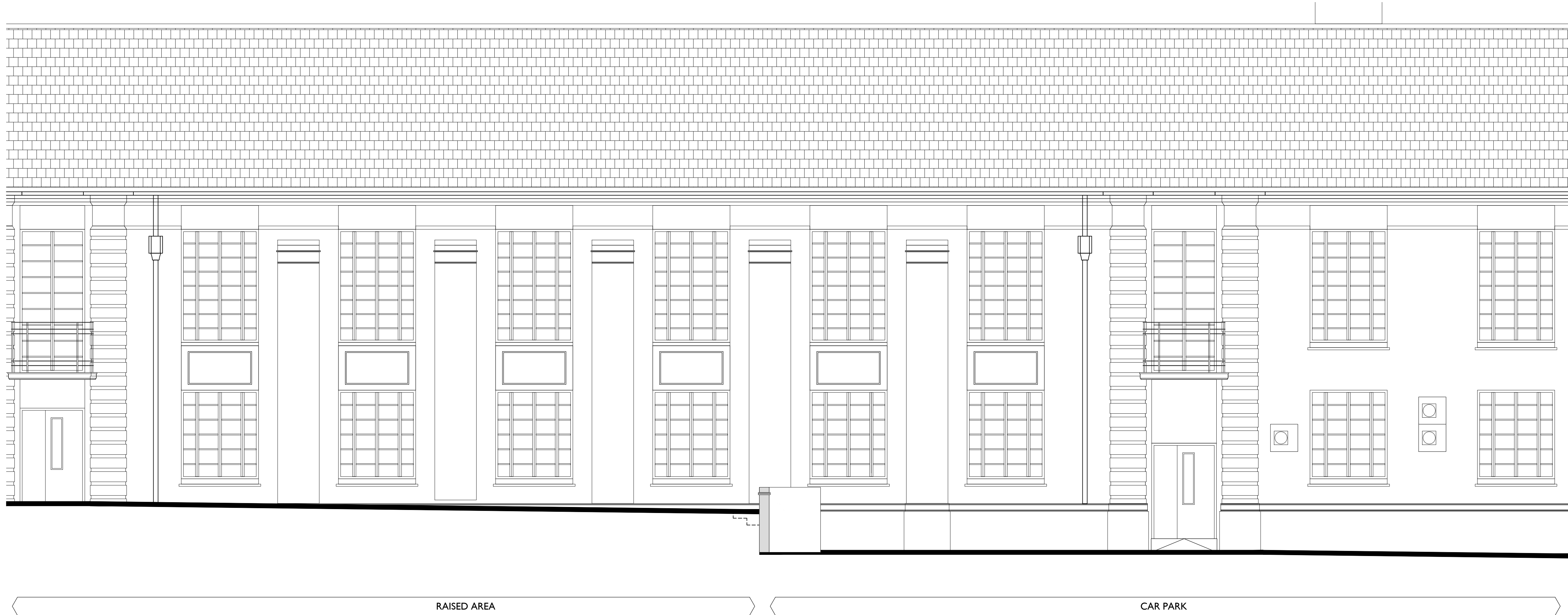
PRE EXISTING LARGER SCALE ELEVATION A - FROM CAR PARK Scale 1:50
