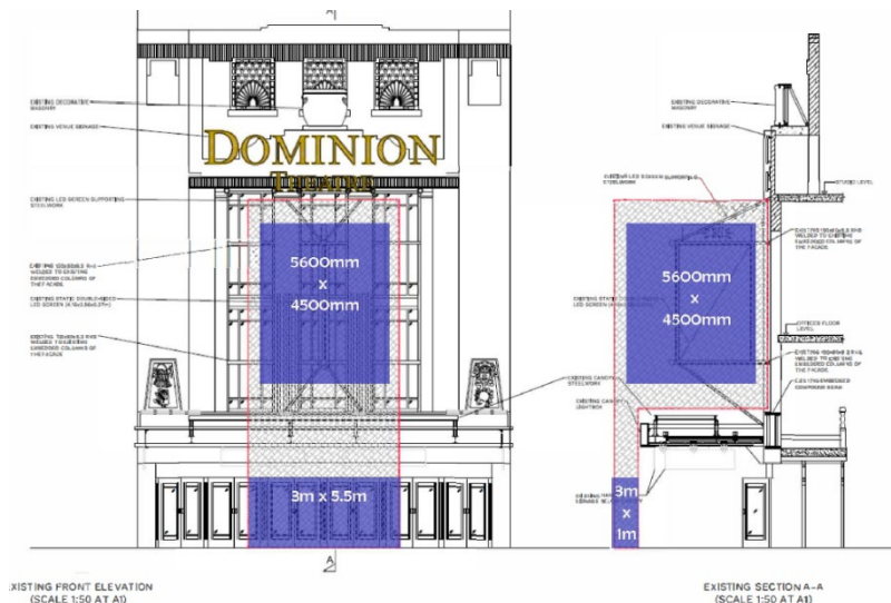
Scaffold for existing sign removal
