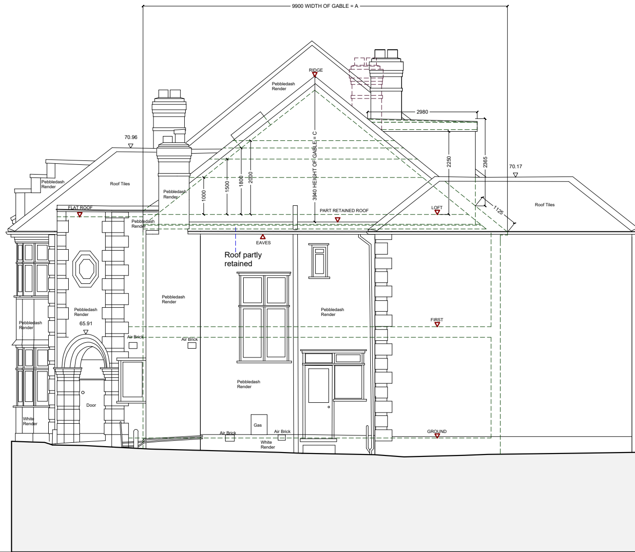
Side elevation proposed
