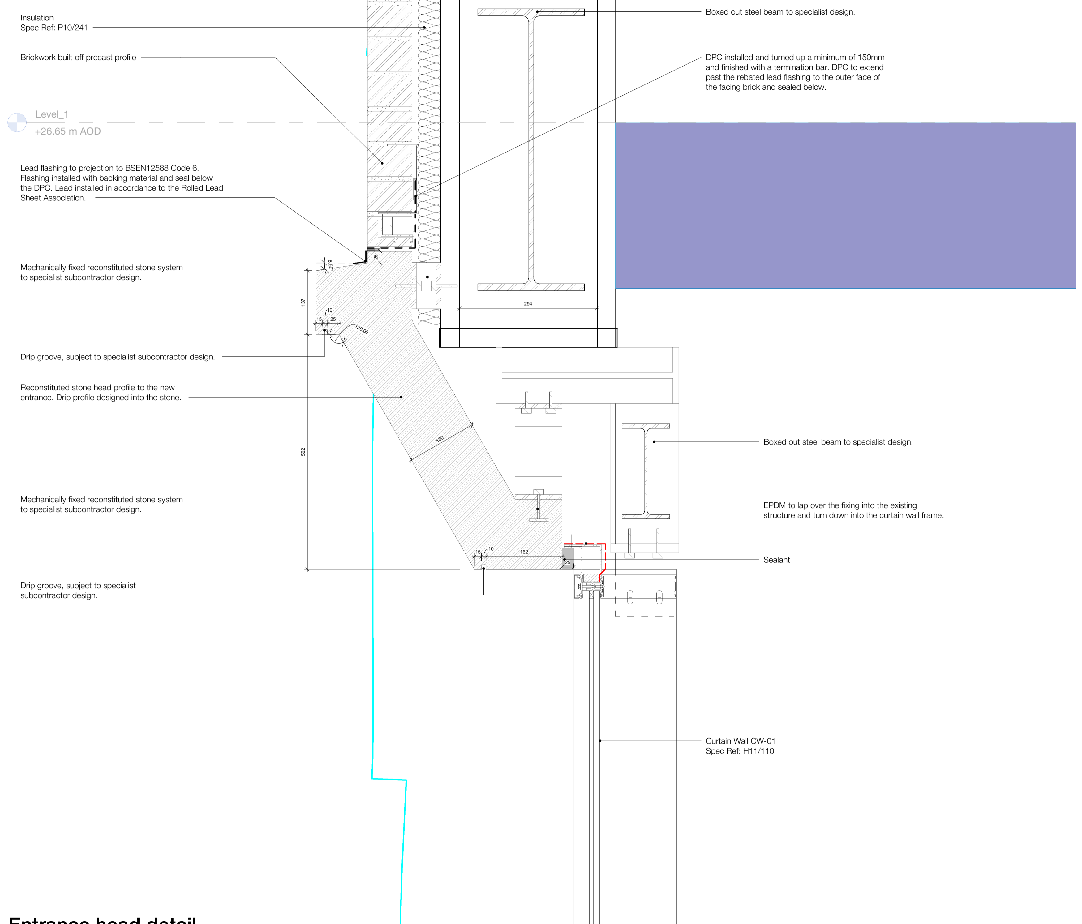
Entrance head detail 1 : 5
