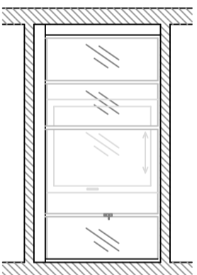
Internal existing wall elevation along A - A
