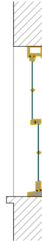
Vertical Sash window detail cross section @ 1:20
