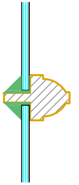
Glazing bar cross section @ 1:2
