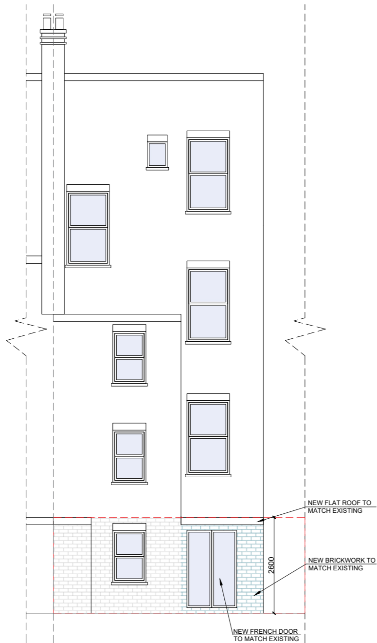
Proposed South Elevation
