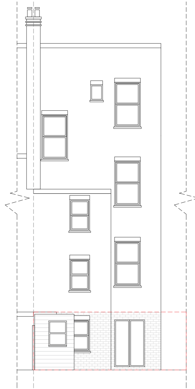
Existing South Elevation (with outbuilding)
