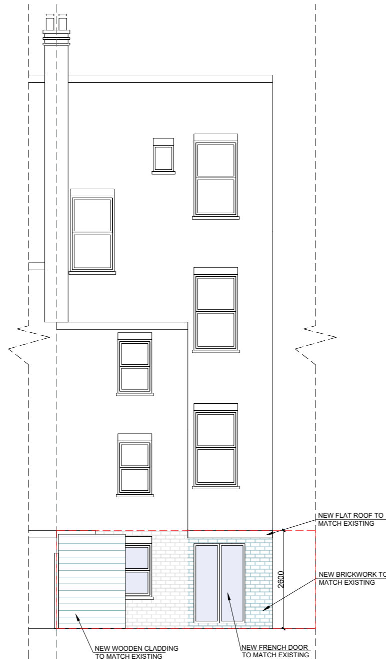
Proposed South Elevation (with outbuilding)
