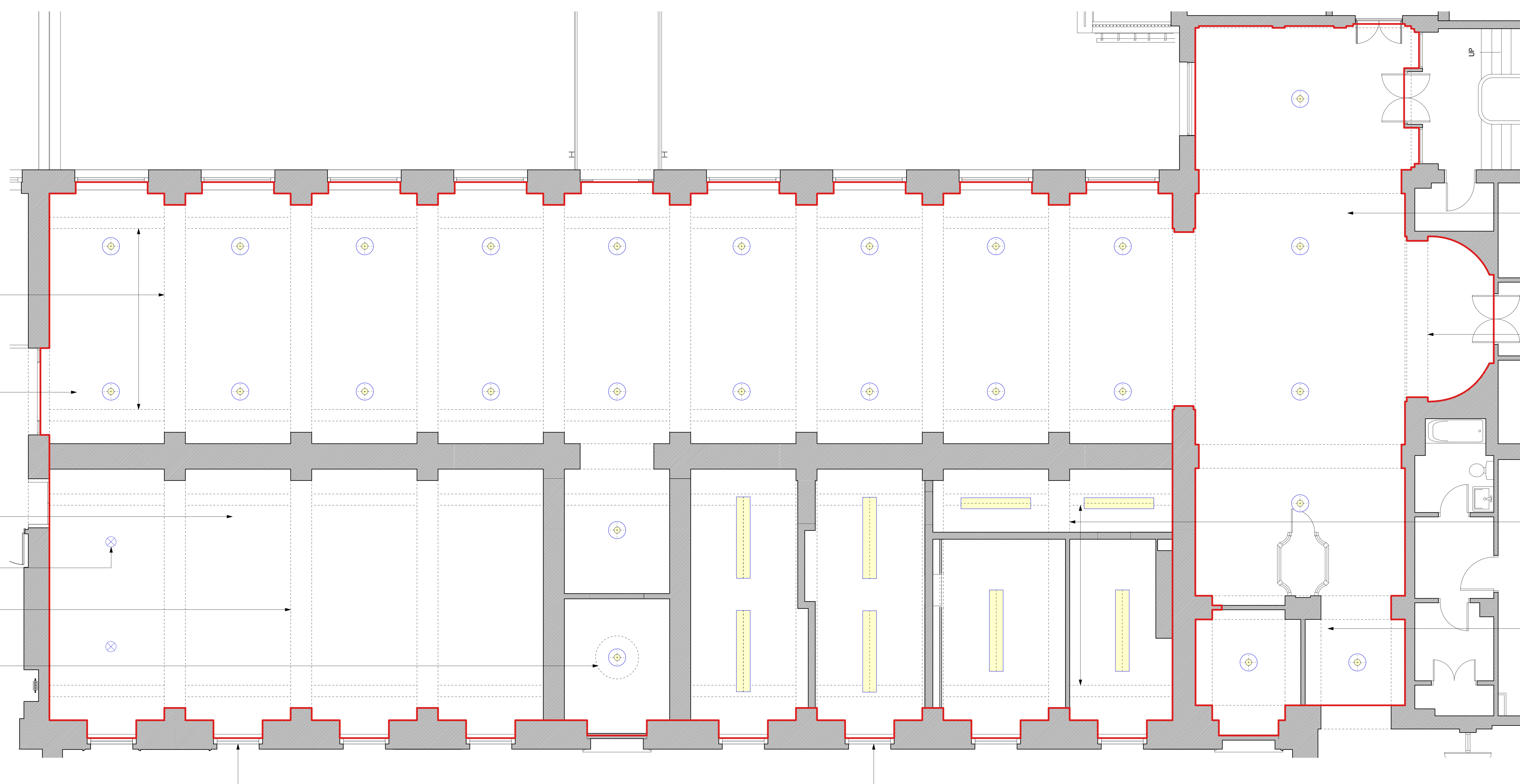
1 South Cloisters Existing RCP 150@A0
